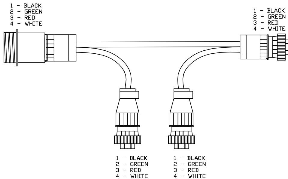
ITEM C02B: 44664 – CABLE UC4 CAN NODE DUAL
