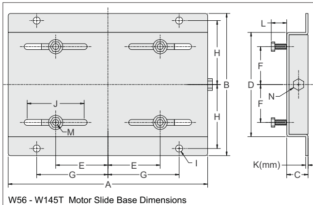
W56 - W145T Motor Slide Base Dimensions
