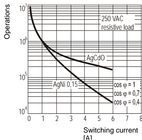
Electrical endurance
