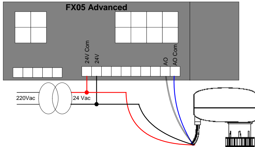
Figure 32: Connecting the Analog Output
