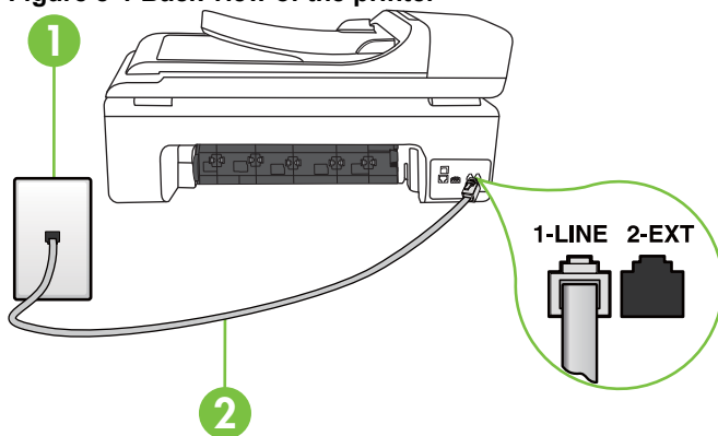
Figure 8-1 Back view of the printer
