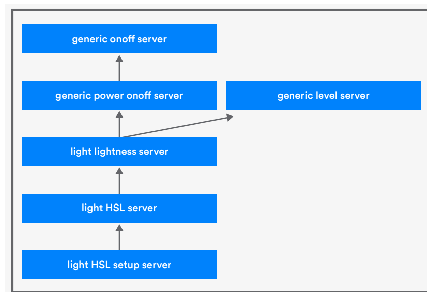
Figure 18 - Light HSL Server and Associated Models
