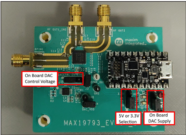
Figure 4. Connection Setup to Use the Onboard Power Supply and Control Voltage
