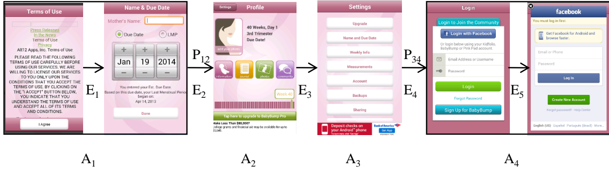
Figure 1: Activity sequences of com.alt12.babybumpfree that invoke Facebook single sign-on window in the fourth activity (A 4 ): Clicking “I Agree” (E 1 ) then clicking “Done” (E 2 ) opens up A 2 with the parameter, fromLoader : tru (P 12 ). Clicking “Settings” (E 3 ) in A 2 opens up the settings activity, A 3 and then clicking “Account” (E 4 ) opens up the login activity, A 4 with the parameter, WHICHCLASS : com.alt12.babybumpcore.activity.settings.Settings . Finally, clicking “Login with Facebook” (E 5 ) opens up the sign-on window within the same activity, A 4 .
