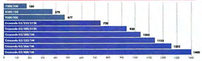
(MacBench 4.0 scores)
