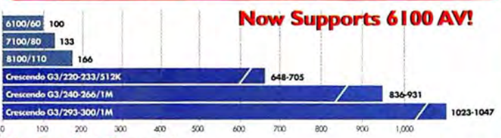
(MacBench 4.0 scores)
