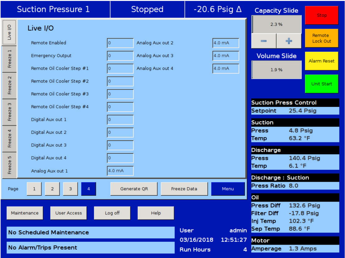
Figure 17-6. Input/Output Screen - Page 4 (Remote Oil Cooler Enabled)
