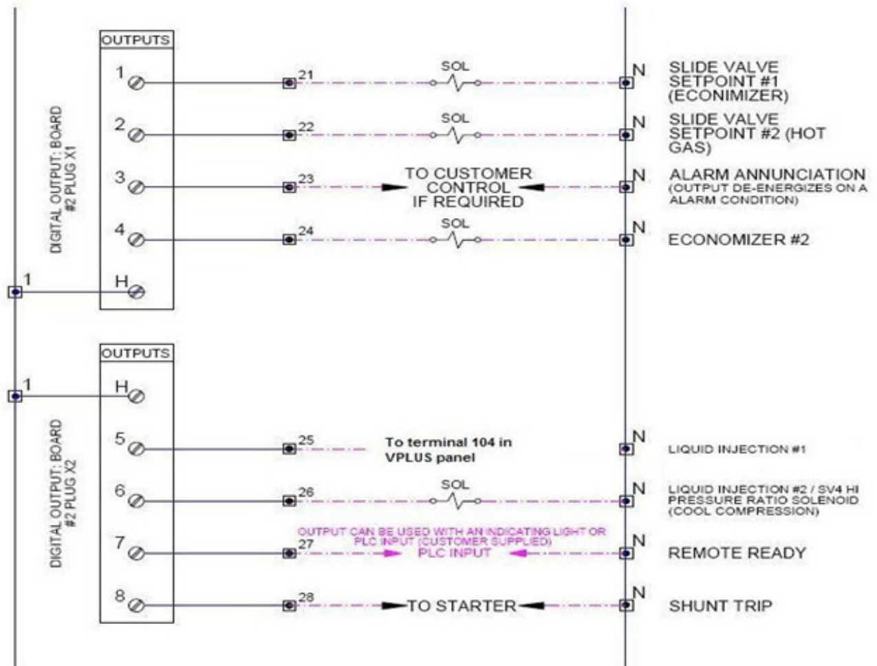
Figure B-31. Digital Output Card Wiring to VPLUS CRV Relay Terminal 104
