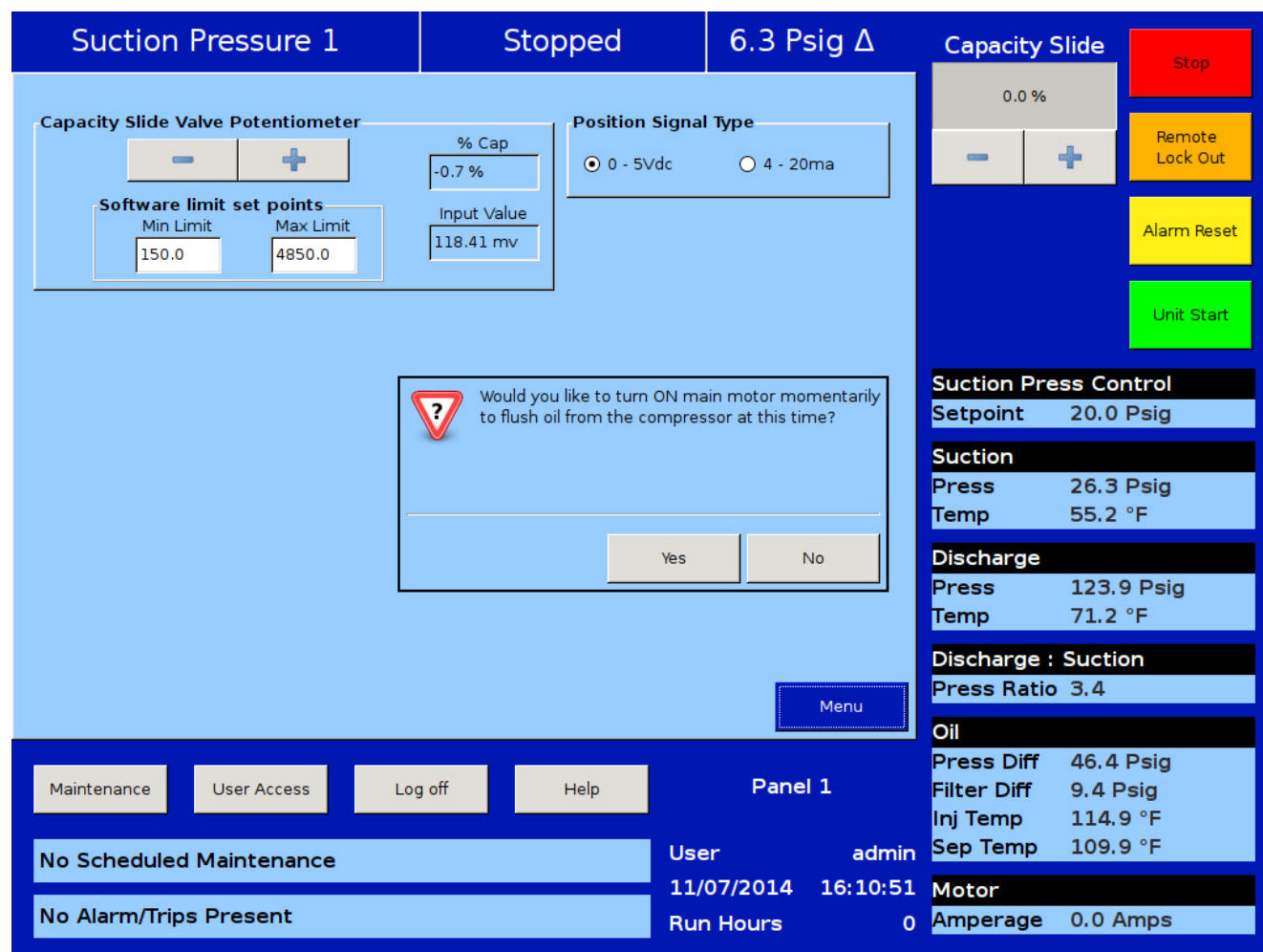
Figure 24-5. Slide Calibration - Twin Screw Bump Pop-up Window
