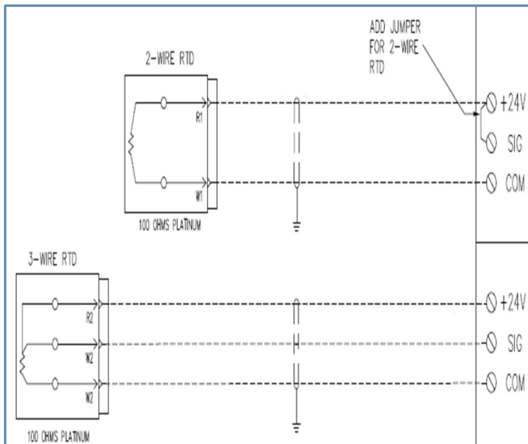
Figure 3-9. 2-Wire and 3-Wire RTD Connection Diagram
