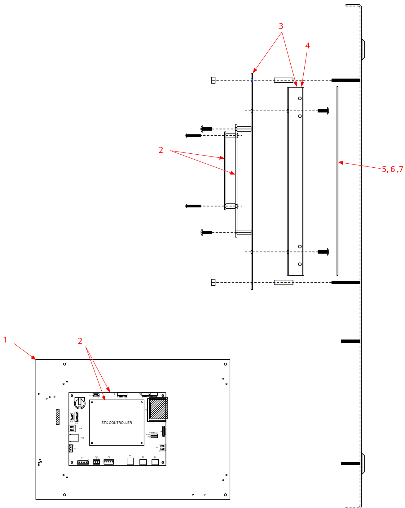
Figure 27-3. Vission 20/20 - SBC Assembly
