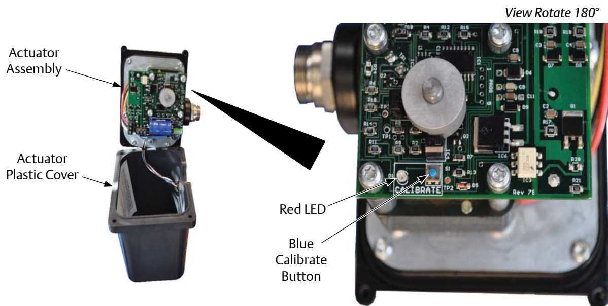
Figure 14-2. Actuator Assembly
