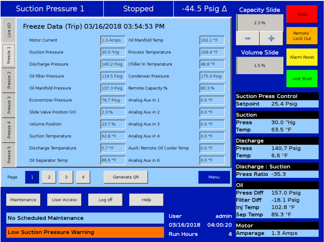
Figure 17-7. Input/Output Screen - Freeze Data Page
