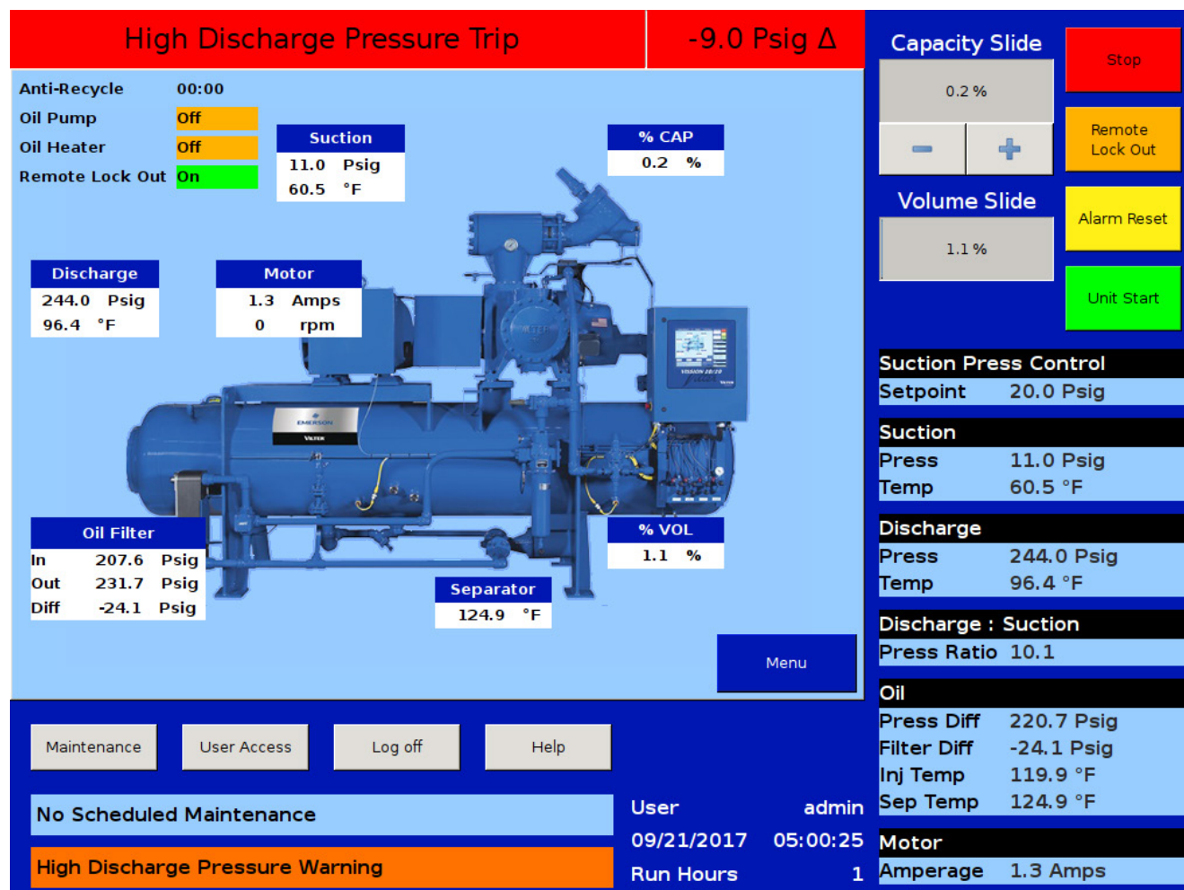
Figure 7-1 - Typical Status Banner Message Display
