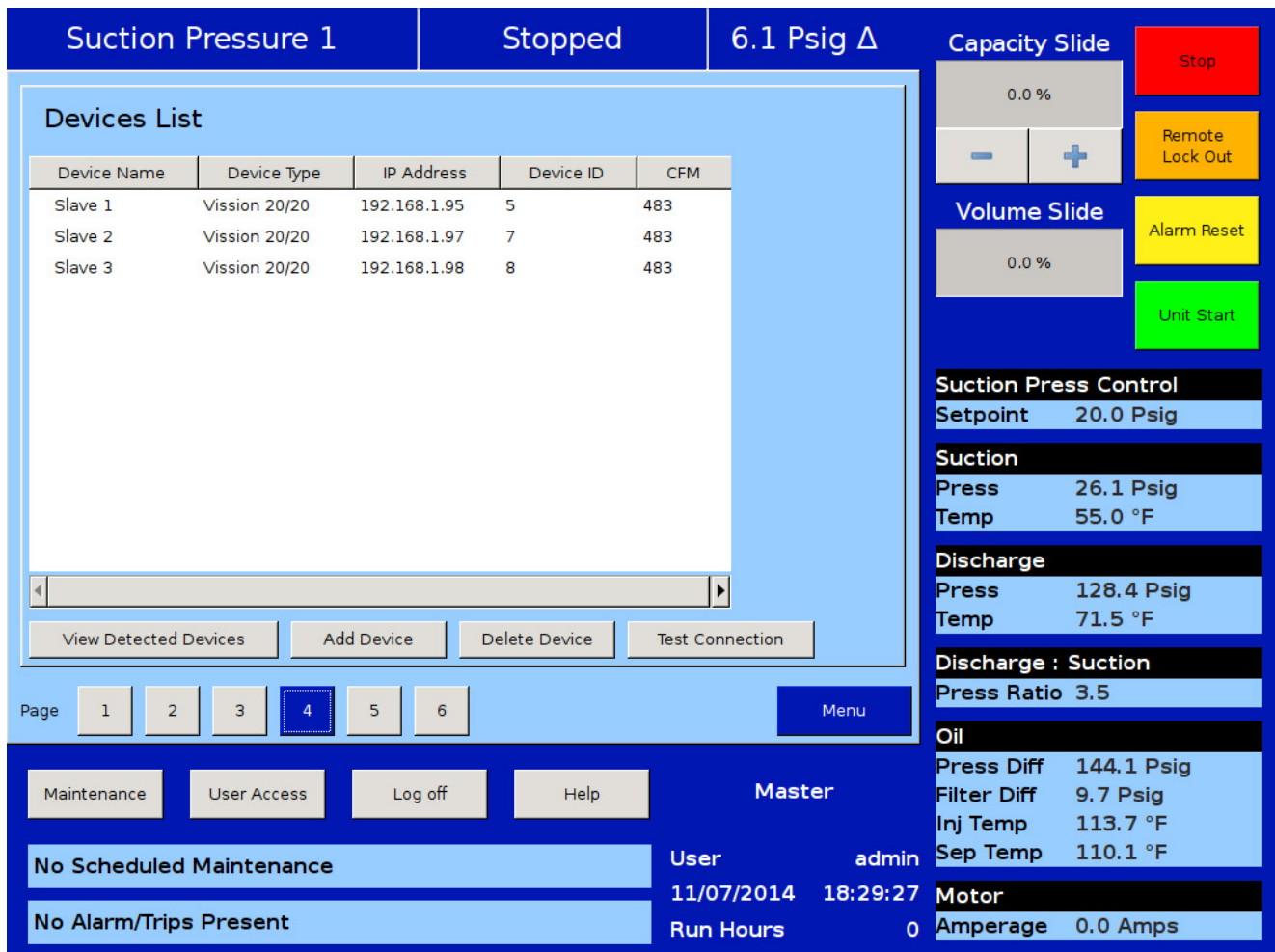
Figure 10-6. Compressor Sequencing Screen - Device List (Page 4)
