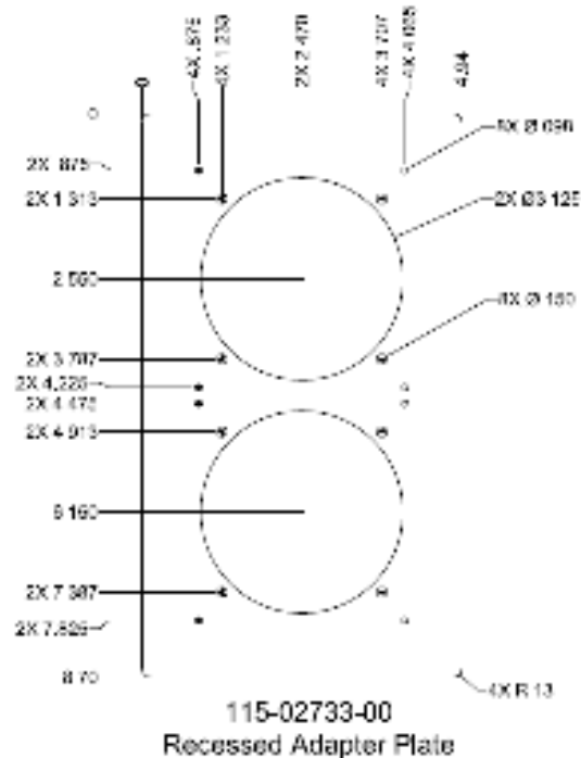
Figure 4-15 Recessed Adapter Plate
