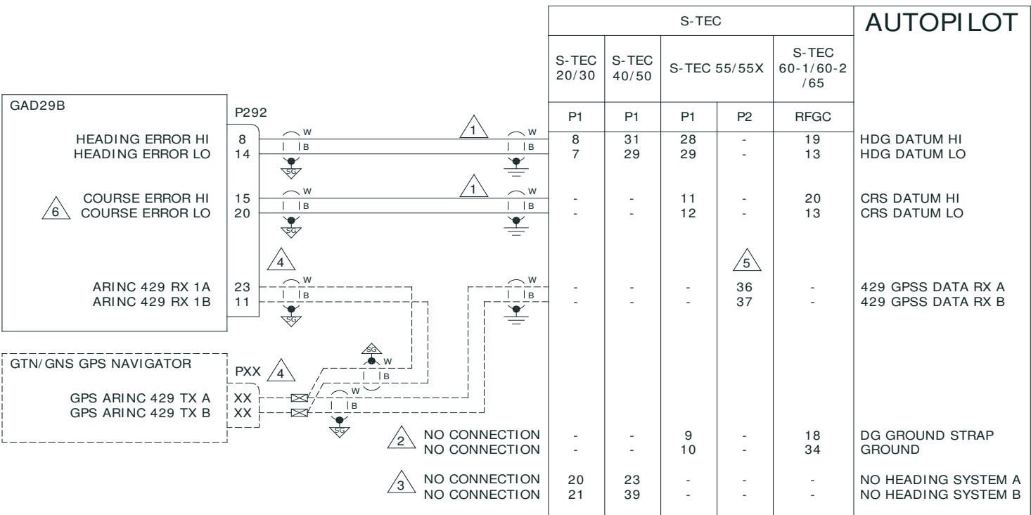
Figure 5-31 GAD 29B Interface to S-TEC Autopilots
