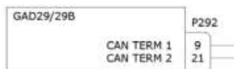
Figure 3-5 CAN Bus Termination for GAD 29/29B
