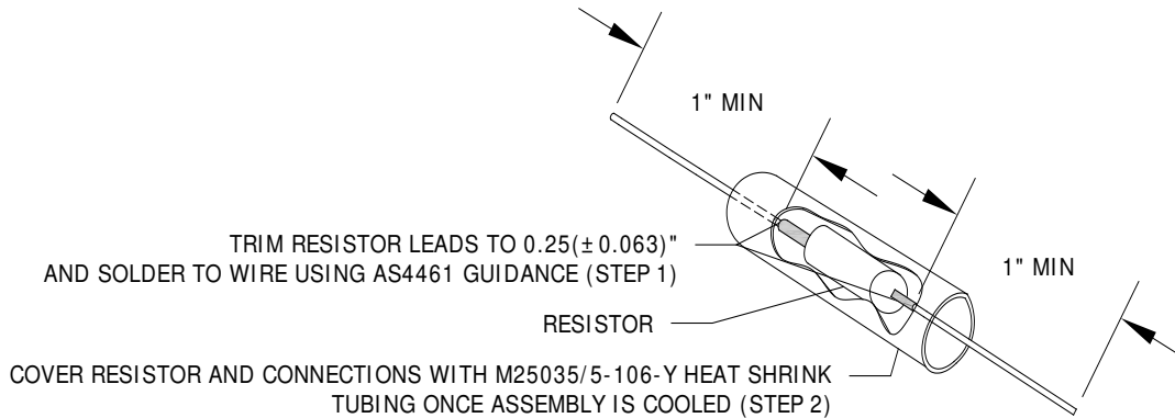
Figure 3-11 G5 Resistor Buildup Using MIL-C-27500 Wire
