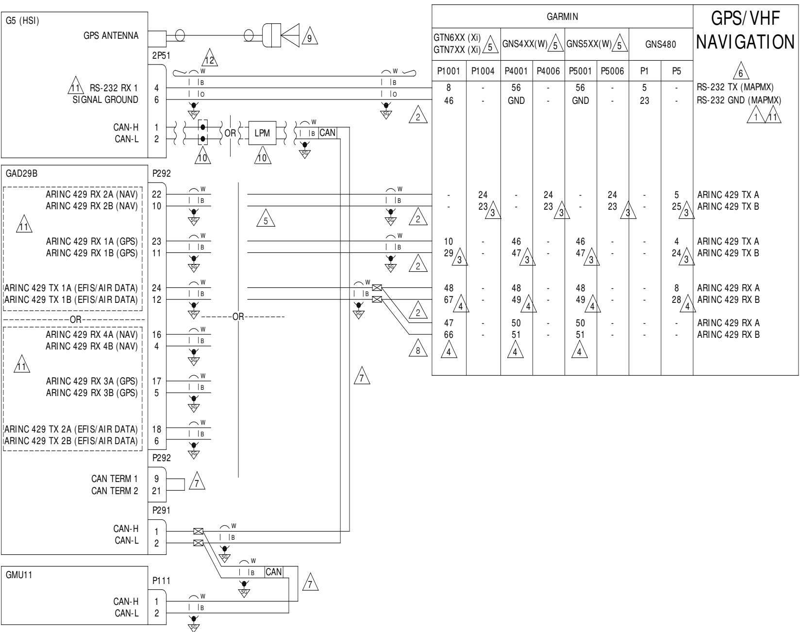
Figure 5-8 G5 (HSI) with GPS/VHF Navigator
