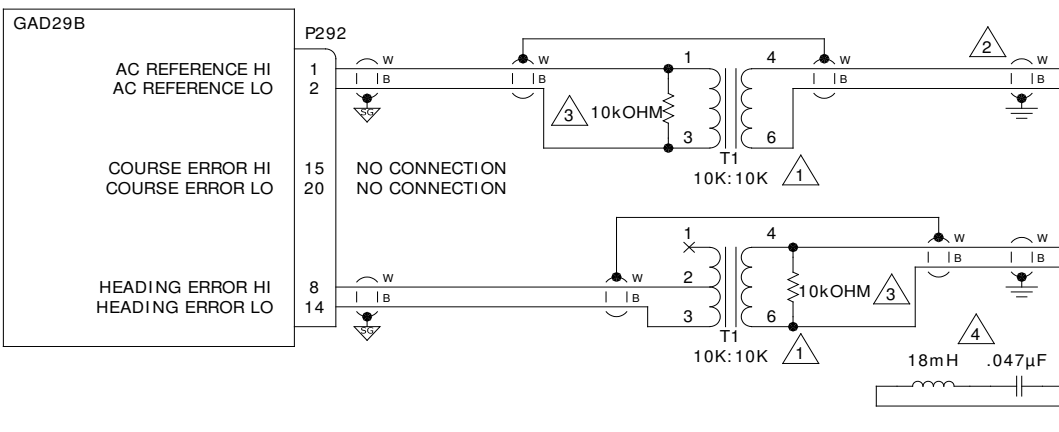
Figure 5-27 GAD 29B Interface to Century Autopilots, Sheet 1 of 2
