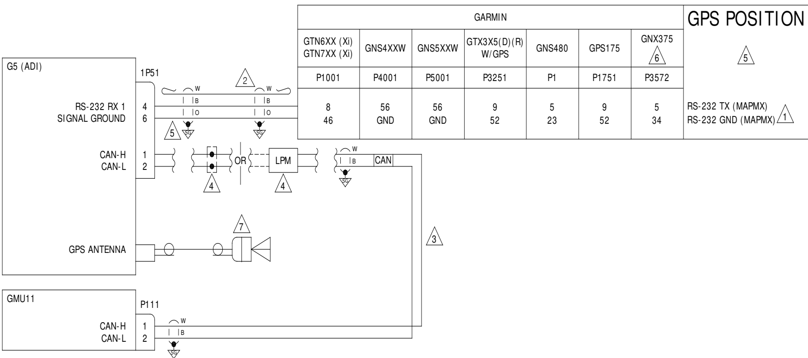
Figure 5-5 G5 (ADI) and GMU 11 with GPS Position Input
