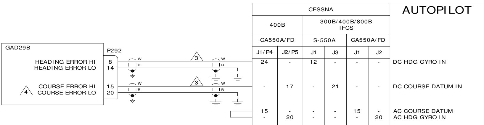
Figure 5-29 GAD 29B Interface to Cessna Autopilots
