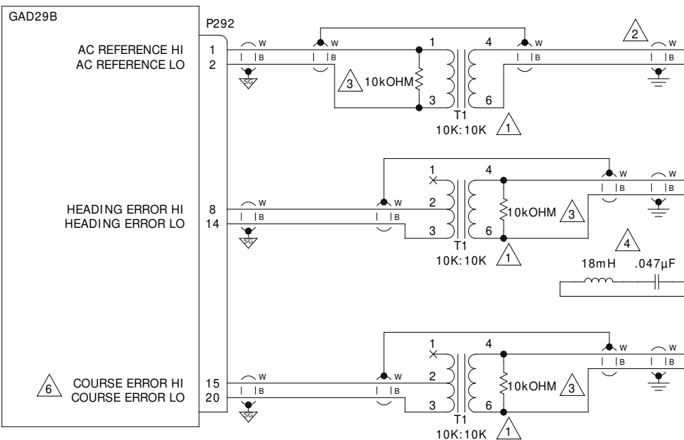
Figure 5-32 GAD 29B Interface To Piper Autopilots
