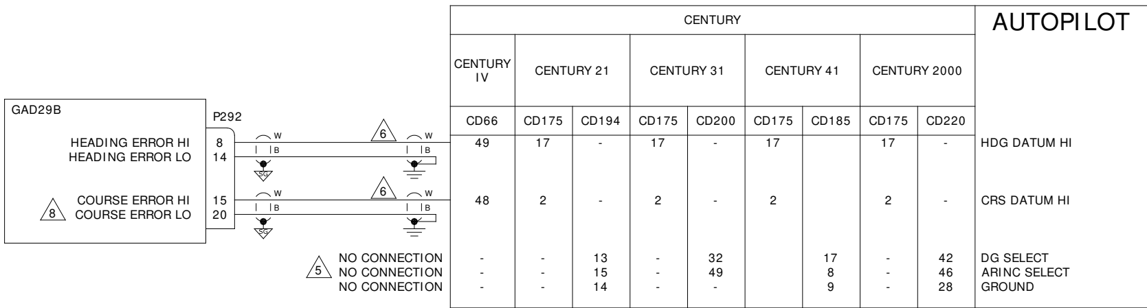
Figure 5-28 GAD 29B Interface to Century Autopilots, Sheet 2 of 2
