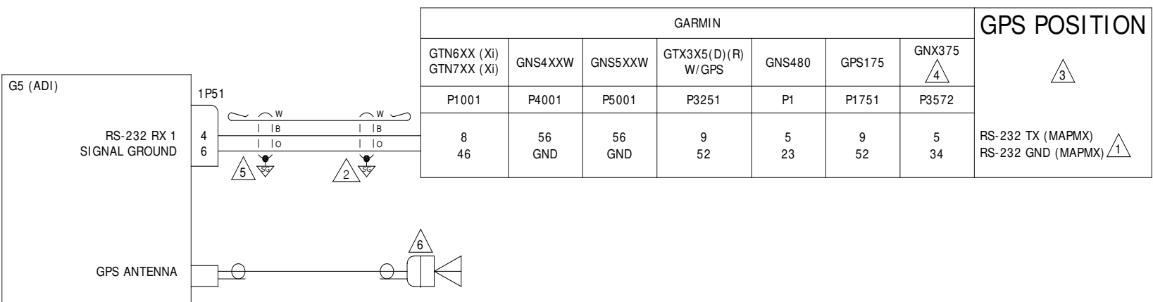
Figure 5-4 G5 (ADI) with GPS Position Input ADI Configuration
