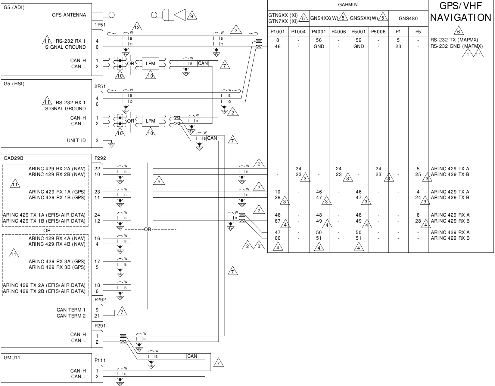
Figure 5-12 Dual G5 with GPS/VHF Navigator
