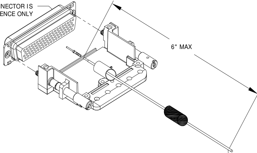
Figure 3-15 Placement of G5 Power Diode Using MIL-C-27500 Wire
