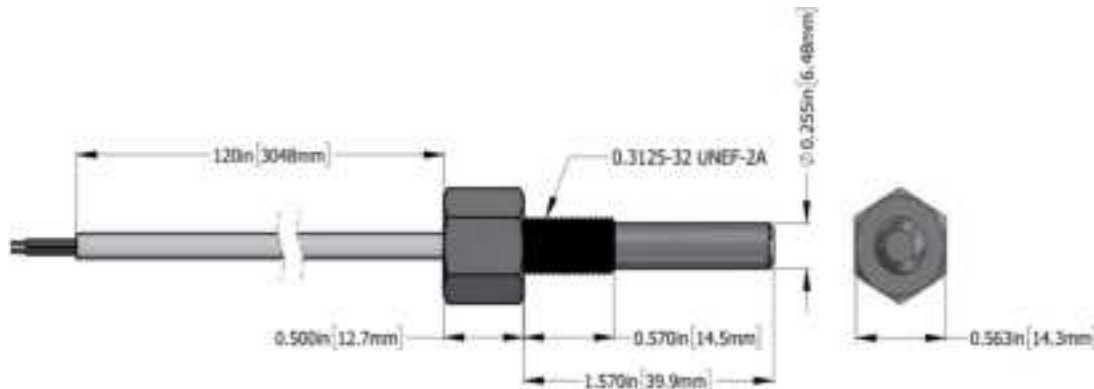
Figure 4-45 GTP 59 OAT Probe Dimensions
