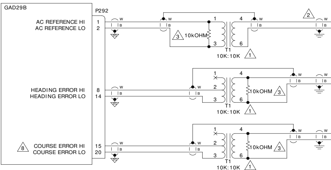
Figure 5-27 GAD 29B Interface to Century Autopilots, Sheet 1 of 2
