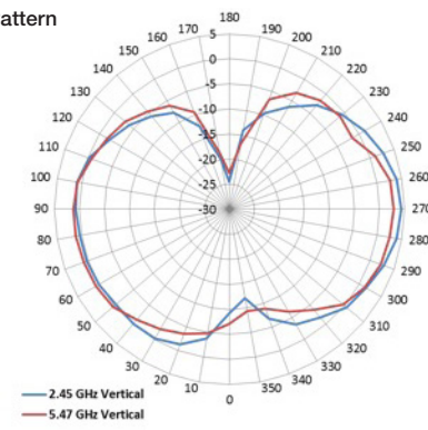
E-Plane Pattern
