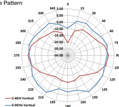
E-Plane Pattern
