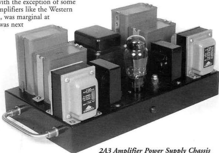
2A3 Amplifier Power Supply Chassis
