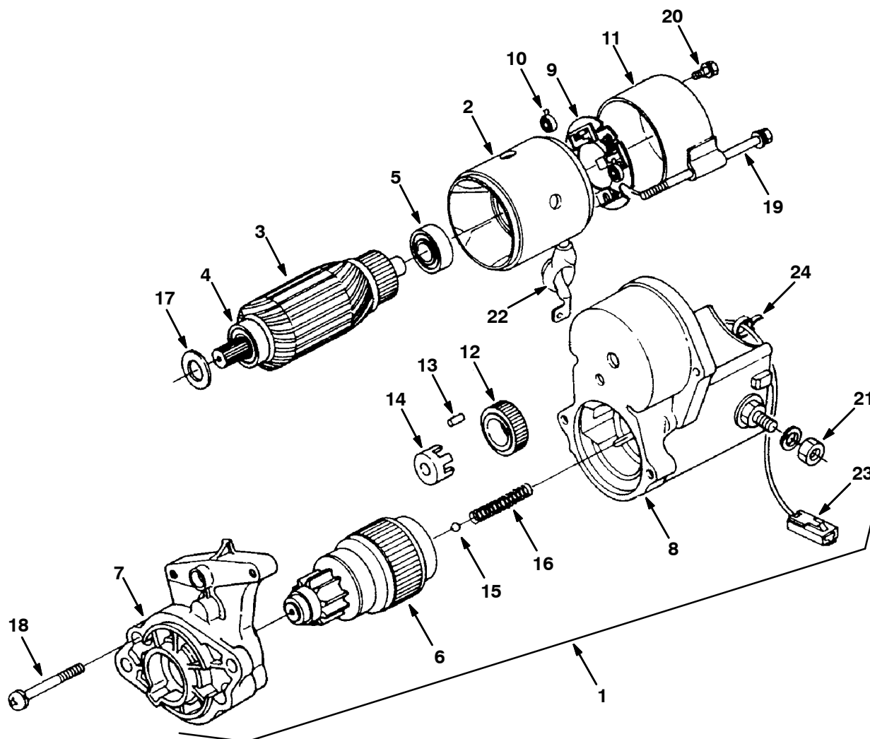
Fig. 24 - Starter Breakdown
