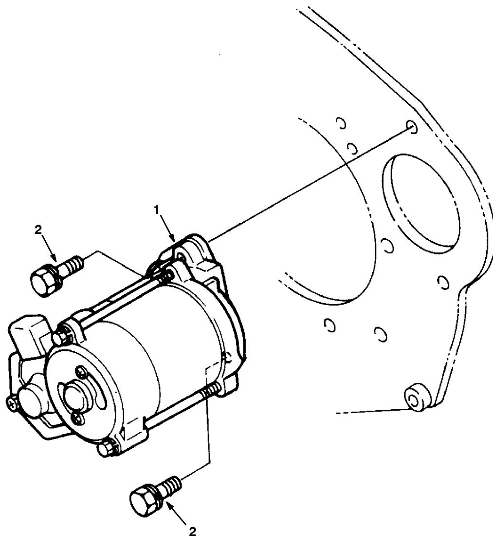
Fig. 23 - Starter Group
