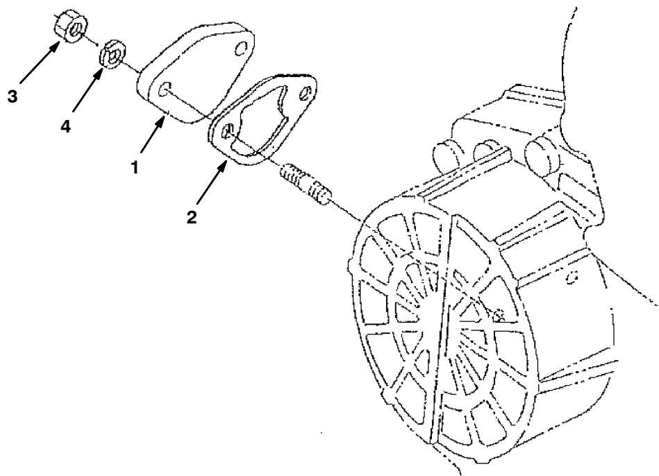
Fig. 12 - Cover Group
