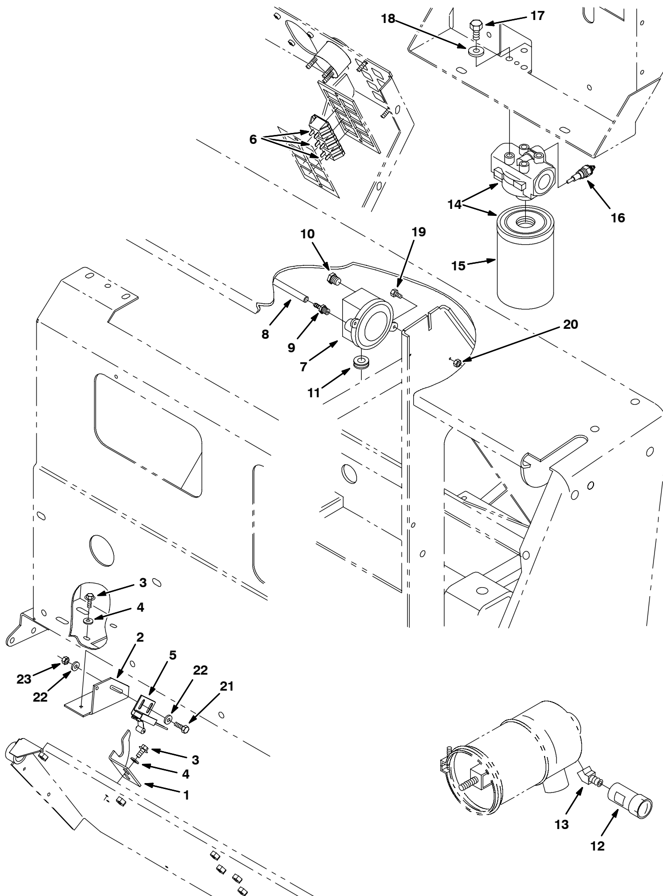
Fig. 6 - Severe Environment Indicator Kit
