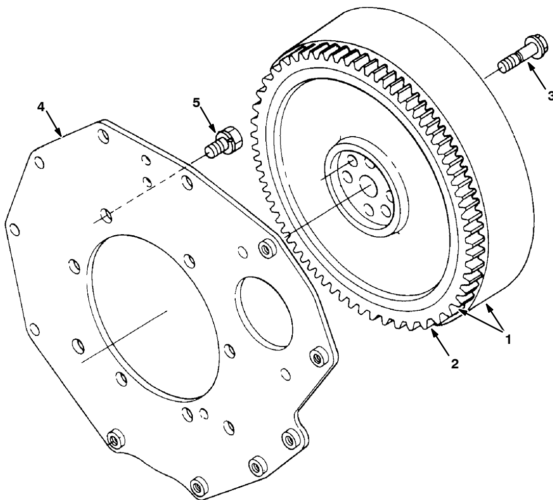
Fig. 16 - Flywheel Group
