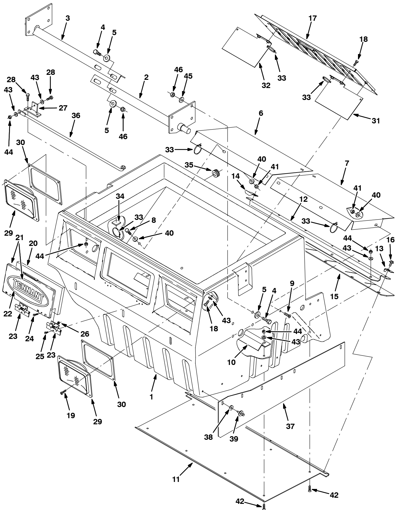
Fig. 28 - Hopper Group
