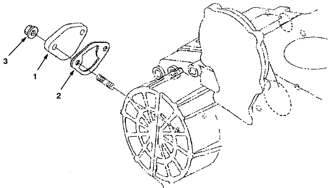
Fig. 10 - Cover Group
