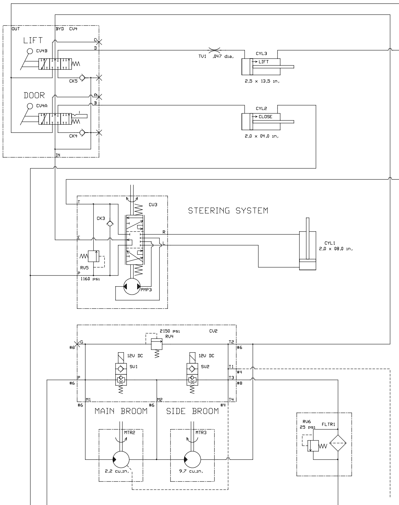
Fig. 38 - Hydraulic Schematic
