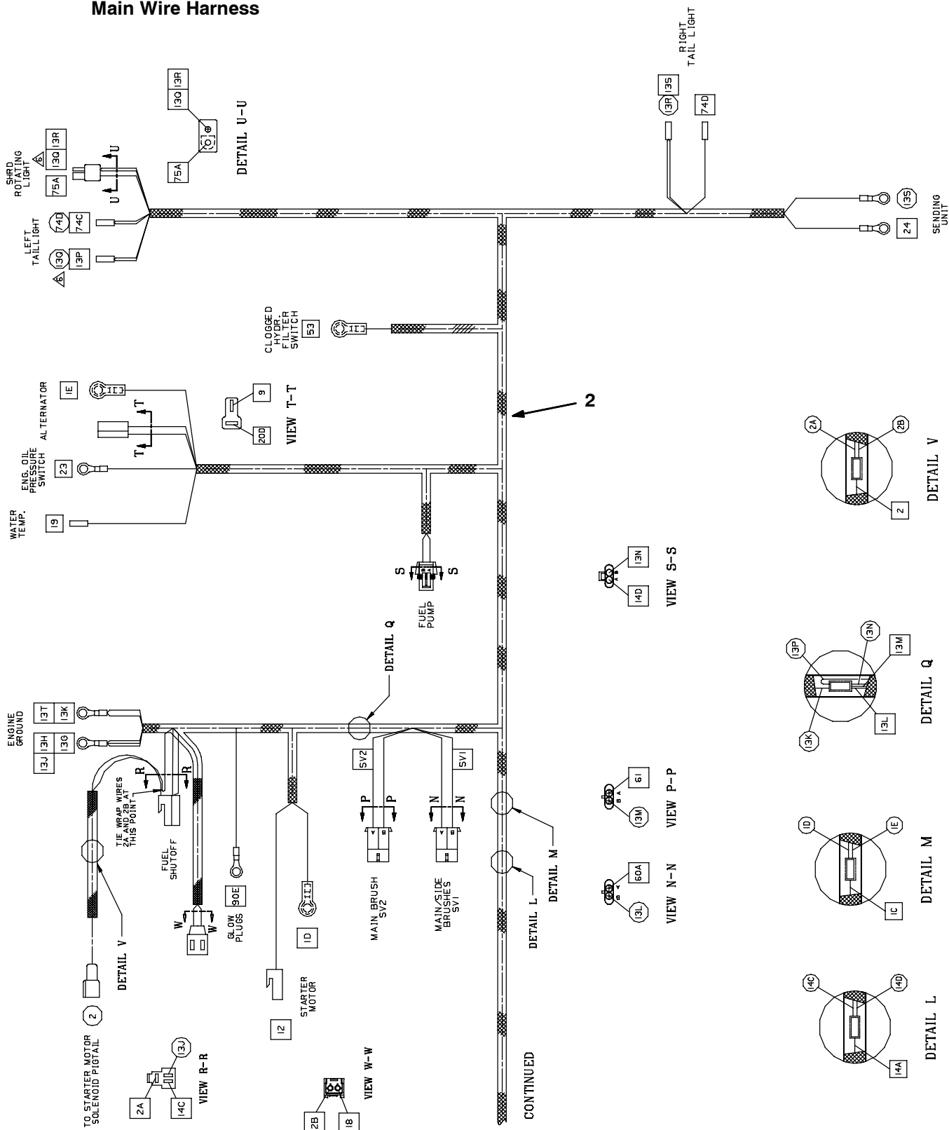
Fig. 42 - Electrical Wire Harnesses Group, Diesel
