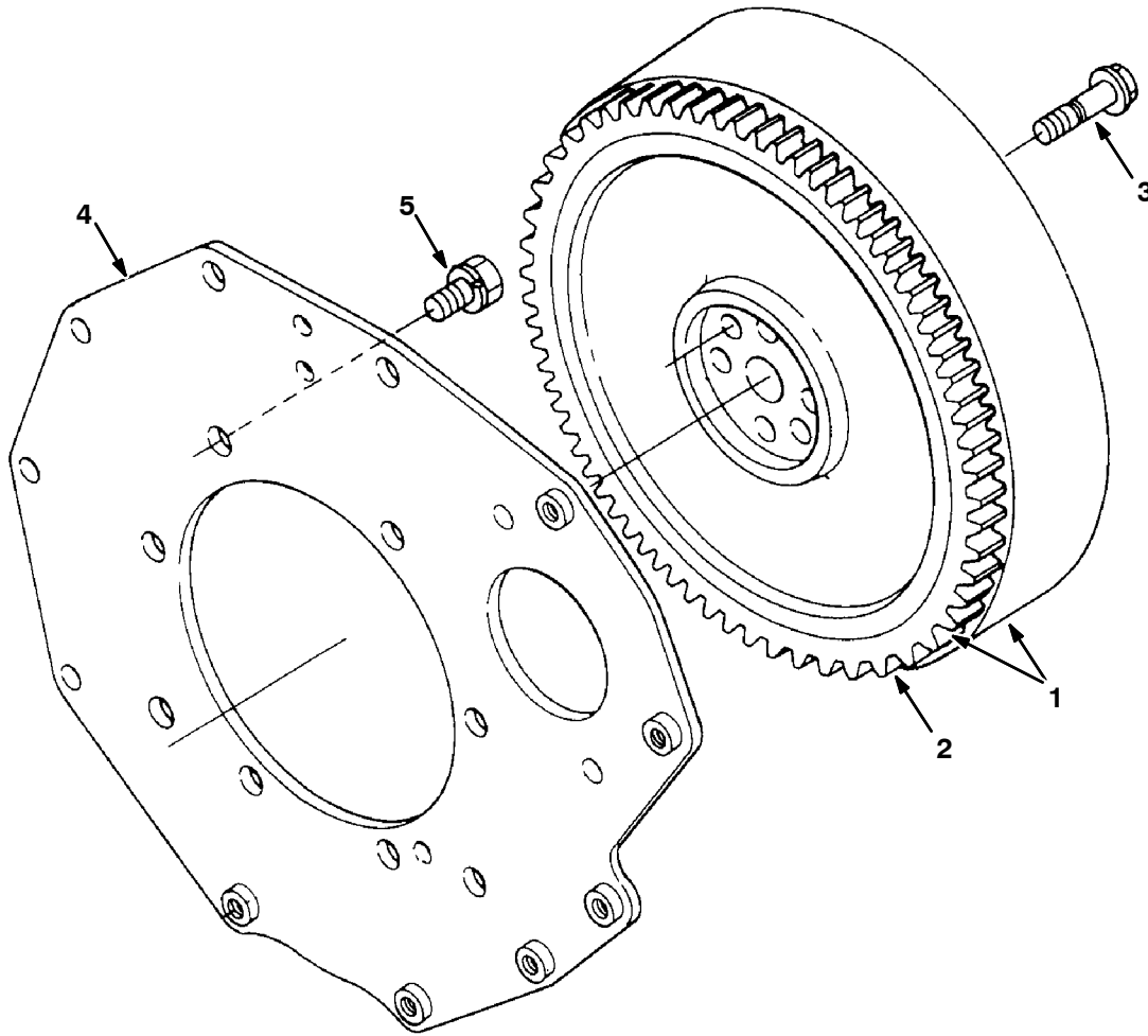
Fig. 14 - Flywheel Group
