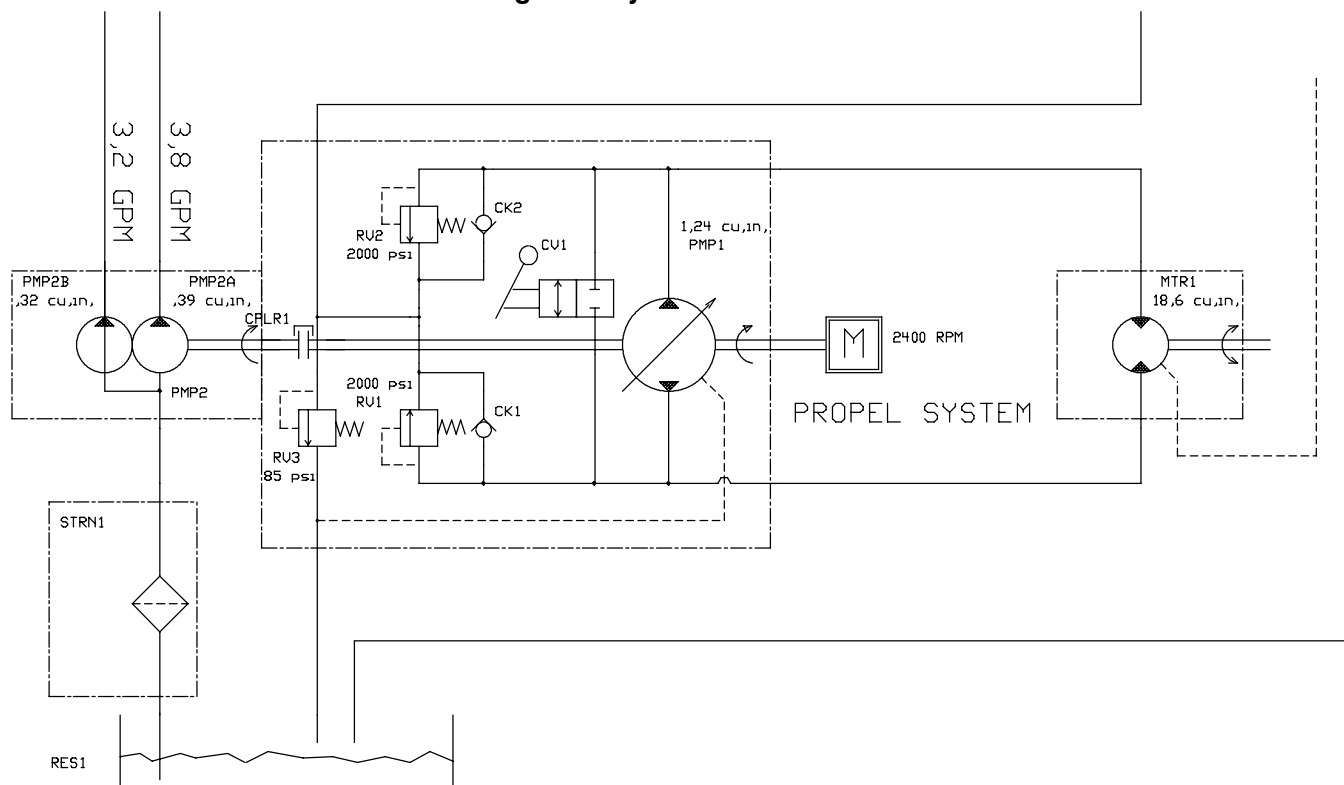
Fig. 38 - Hydraulic Schematic
