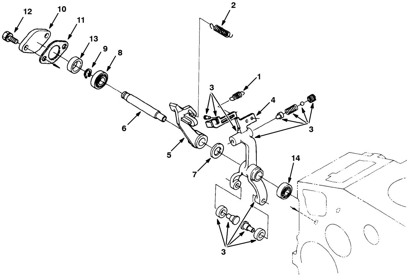
Fig. 20 - Governor Group
