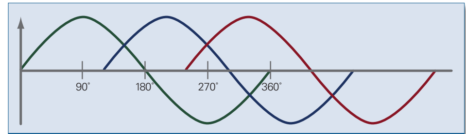
Figure 1. Three-phase power
