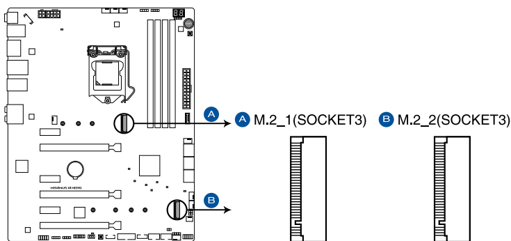
ROG MAXIMUS XI HERO M.2 sockets
