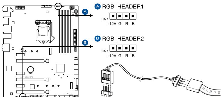
ROG MAXIMUS XI HERO RGB_HEADER connectors
