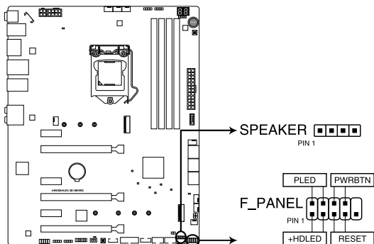
ROG MAXIMUS XI HERO SPEAKER & F_PANEL connectors
