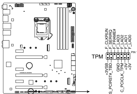
ROG MAXIMUS XI HERO TPM connector
