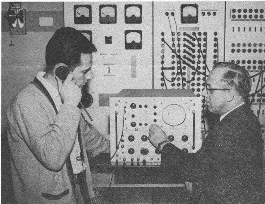
A PARTIAL GRANT to Vancouver's Clark college physics department is this Tektronix Type RM45 oscilloscope. John Walker (left), sophomore from Vancouver, and physics instructor Ted Klump check John's frequency limit on the new instrument.
