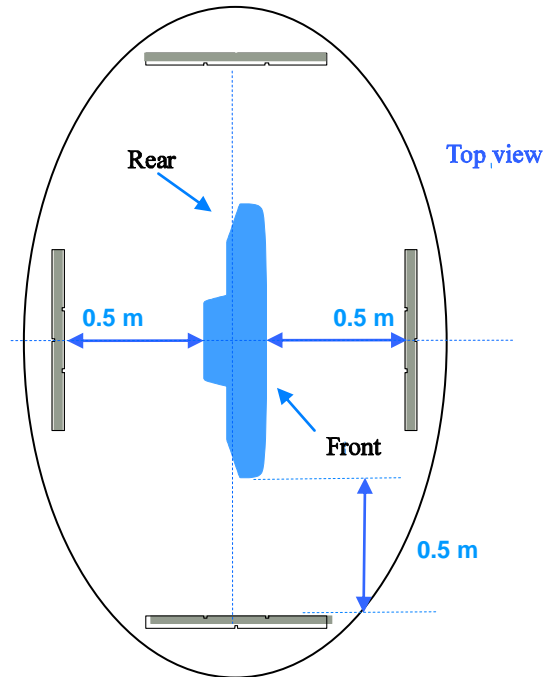
Figure B.4.1.3.1. Measurement geometry for band I and band II.
