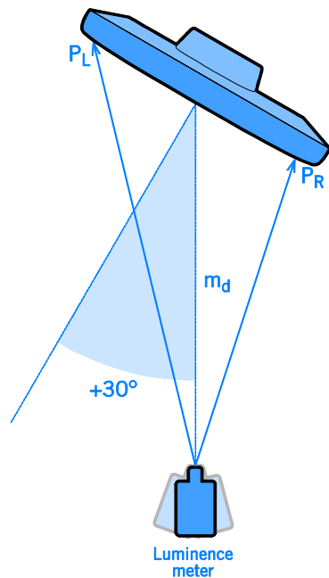
Figure B.2.2.4.2. Top view of test set-up when the All-in-one PC is rotated \pm 30 degrees. The + rotation is defined clockwise.
