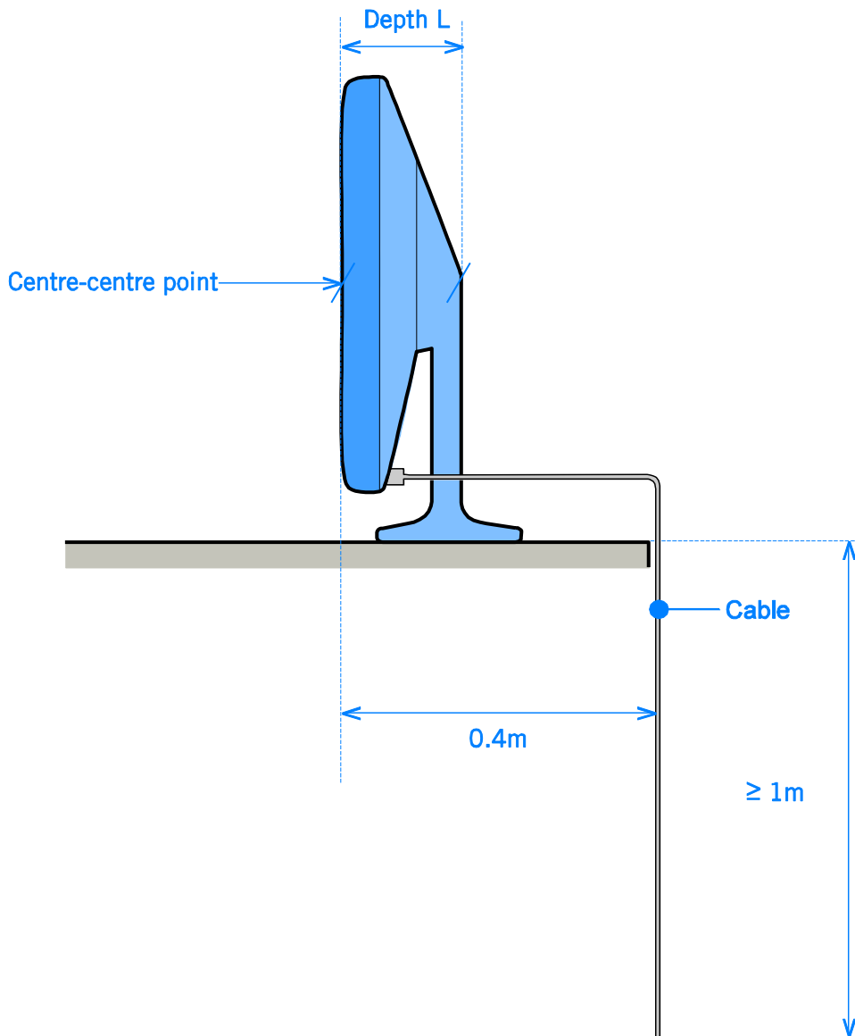
Figure B.4.0.2.1 All-in-one PC without external power supply unit.
