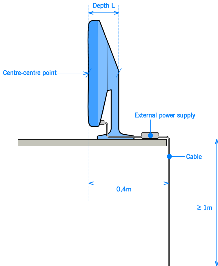
Figure B.4.0.2.2 All-in-one PC with external power supply units.
