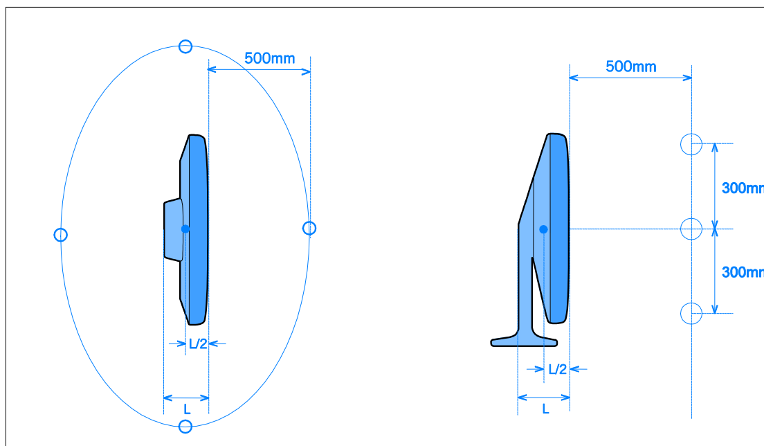
Figure B.4.2.3.1. Measurement geometry for the test object.
