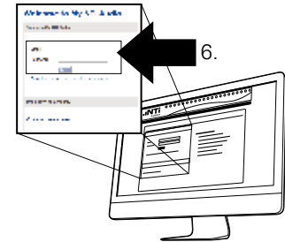
Login ( https://my.nti-audio.com )
