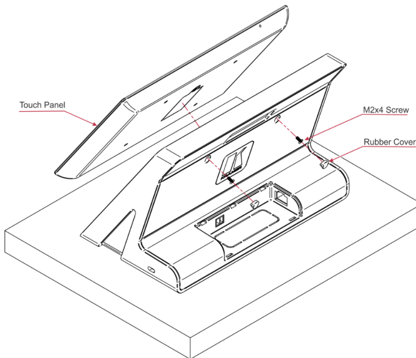
Figure 8: Connecting to the KT-107S Rear Panel
