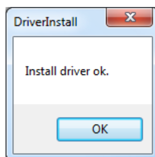
Figure 34: Successful Installation
