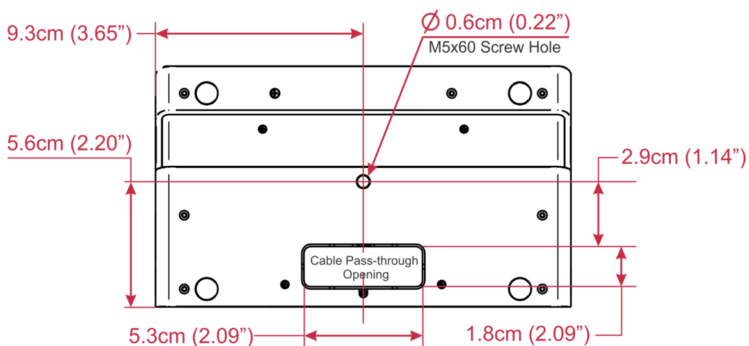
Figure 5: Cut-Out Dimensions (image not to scale)
