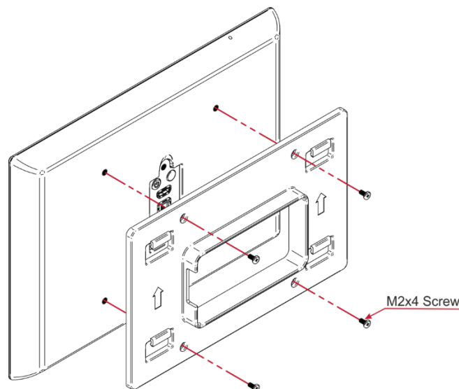
Figure 12: Attaching the Panel Mount Plate to the Rear Side of the KT-107S
