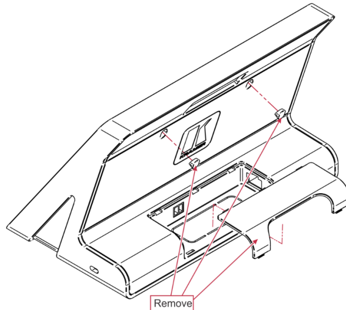
Figure 6: Removing Cable Cover and Rubber Screw Cover
