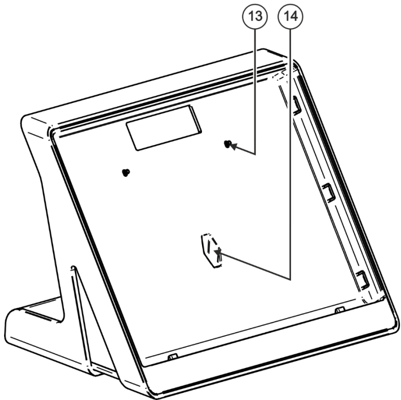
Figure 2: Tabletop Mount Front View
