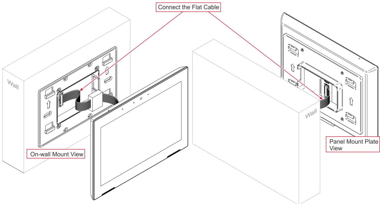
Figure 13: Connecting the On-wall Mount Flat Cable
