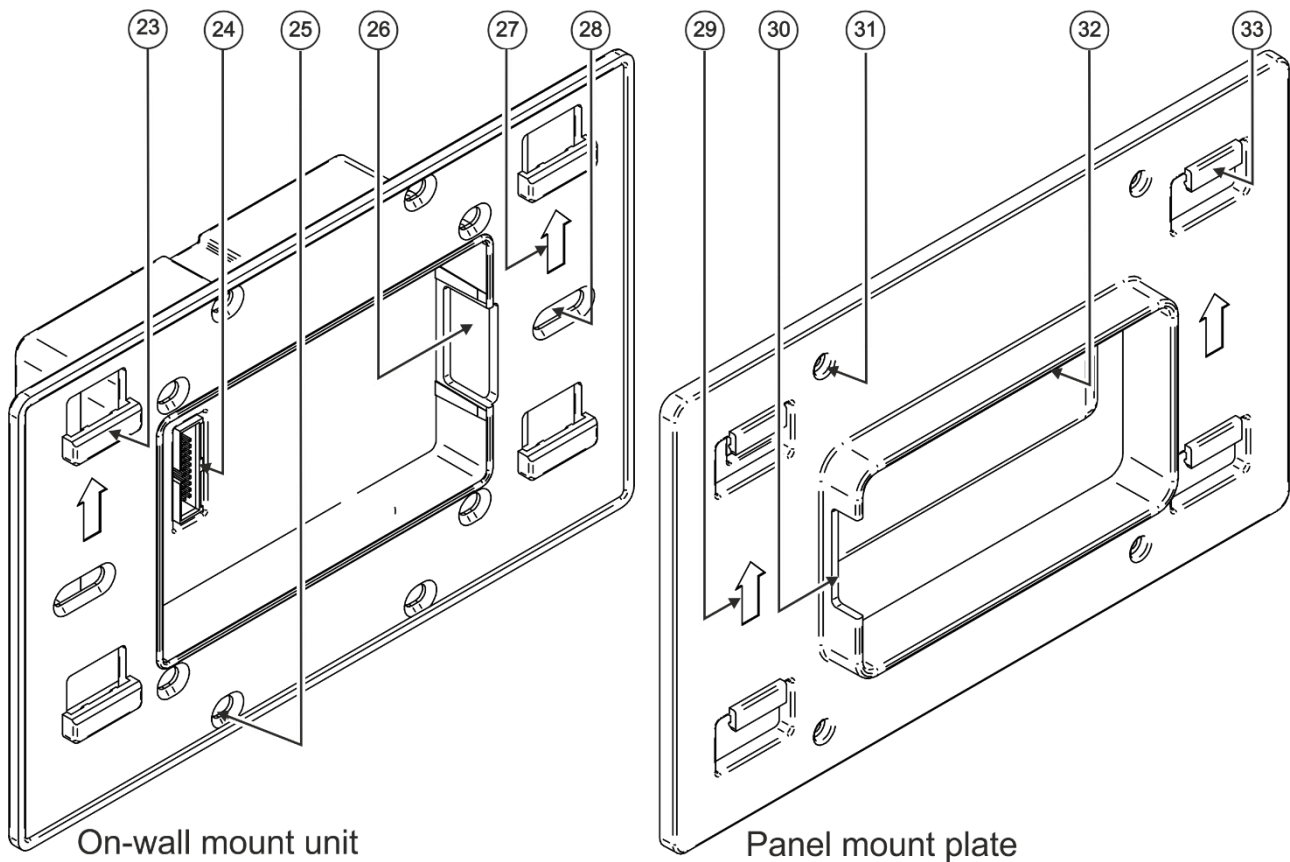
Figure 4: KT-107S Touch Panel Front Panel
