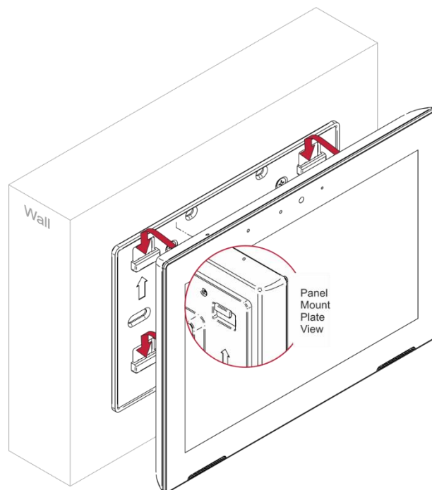
Figure 14: Hanging KT-107S on the Wall
