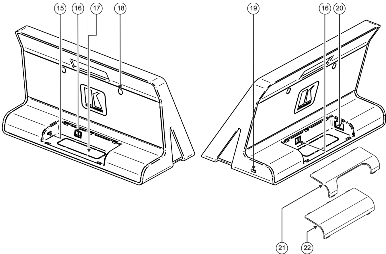
Figure 3: Tabletop Mount Rear View
