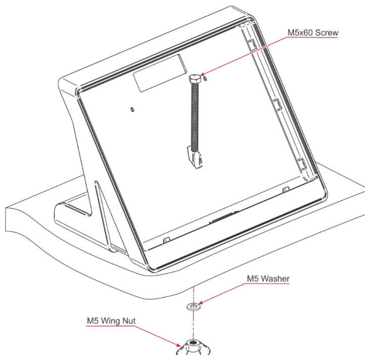
Figure 7: Securing Tabletop Mount
