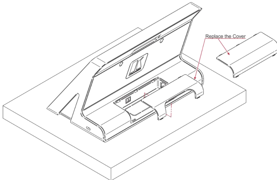
Figure 9: Replace the Cover
