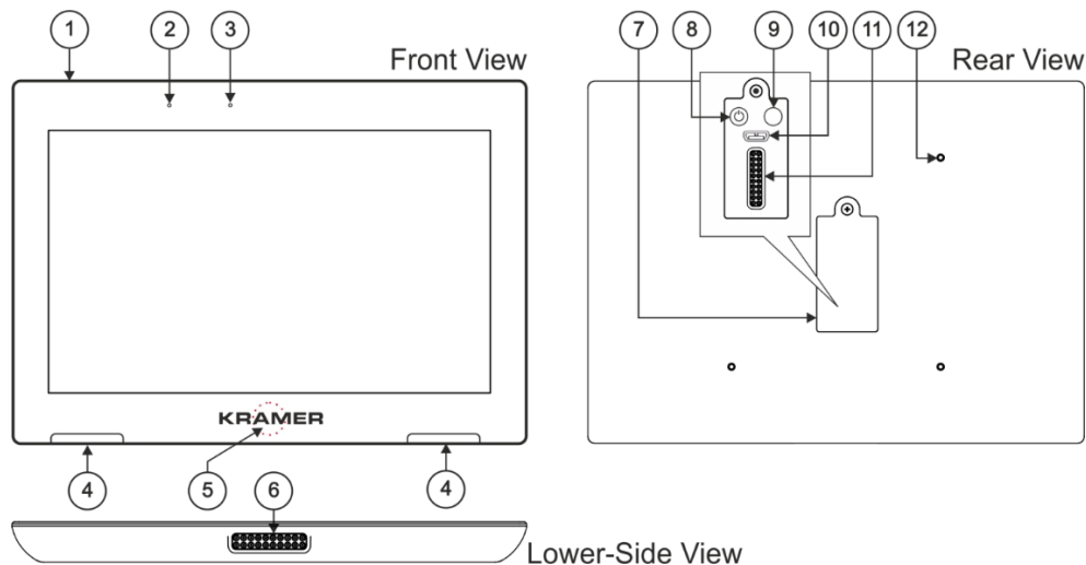
Figure 1: KT-107S Touch Panel Front, Rear, and Lower Side view
