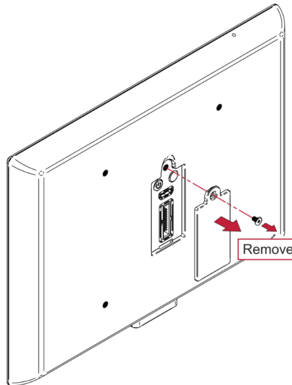
Figure 11: Removing the Cover on the KT-107S Rear Side
