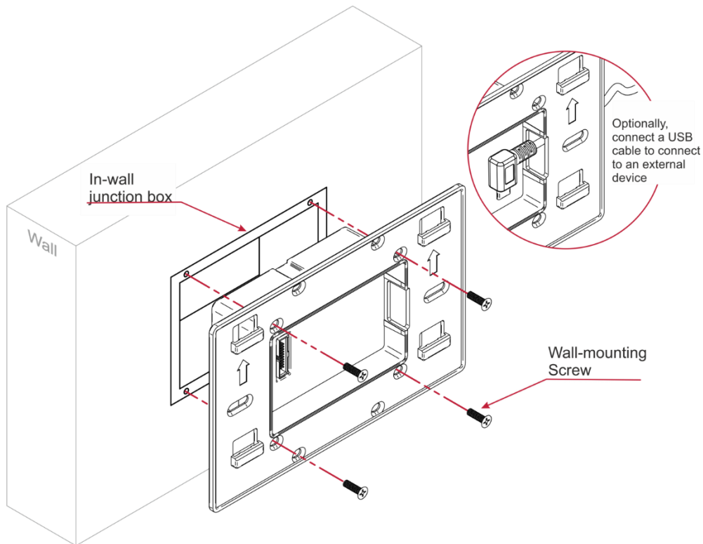
Figure 10: Installing the On-Wall Mount Unit
