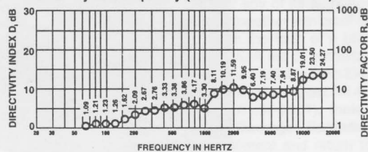
FIGURE 5 — Directivity vs. Frequency (anechoic environment)
