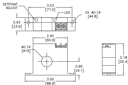
ACTR Series, Up to 200 Amp Fixed Core
