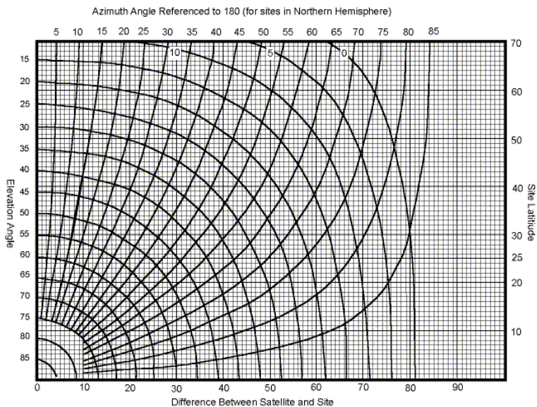
Figure 12-71 Polarization angle compensation curve
