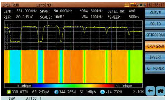
Figure 12-159 Snapshot: Curve - Spectrogram Display Mode
