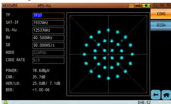
Figure 12-61 DVB-S2 32APSK Constellation
