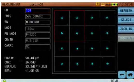
Figure 12-43 DTMB Constellation
