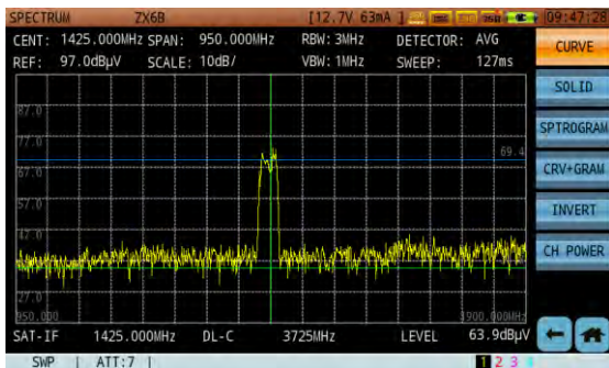
Figure 14-61 UB-2 Channel is Opened
