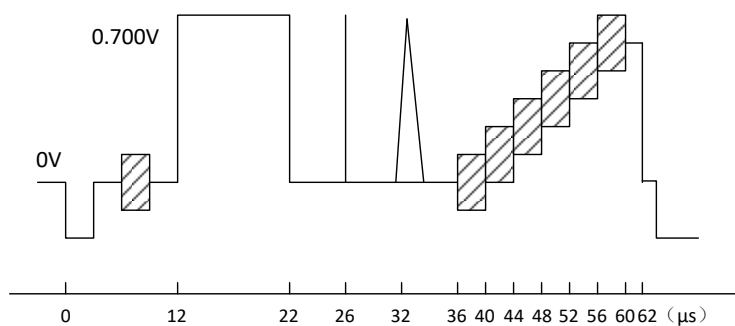
Figure 13-19 GB19
