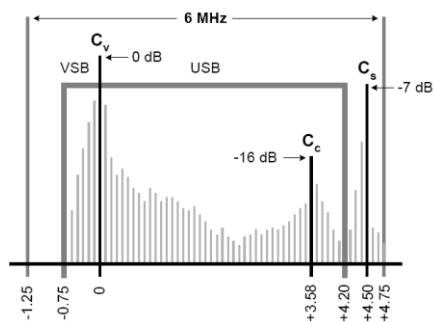
Figure 13-1 TV Standard - M, N
