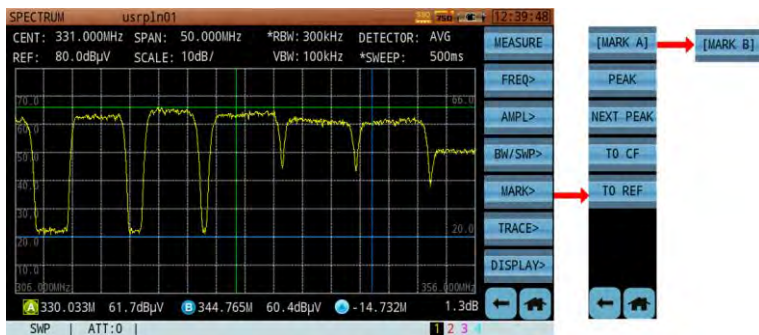
Figure 12-148 Marker Settings Menu
