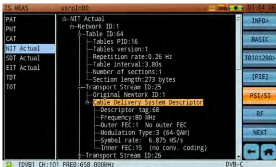
Figure 12-87 PSI/SI Analysis-NIT Table
