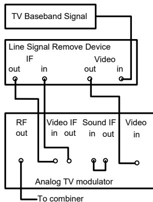
Figure 13-14 CTB quit line removing equipment connection Quiet line inserter in this example: TVMS4200.
