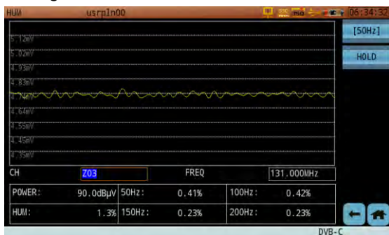
Figure 12-2 Digital Hum Measurement
