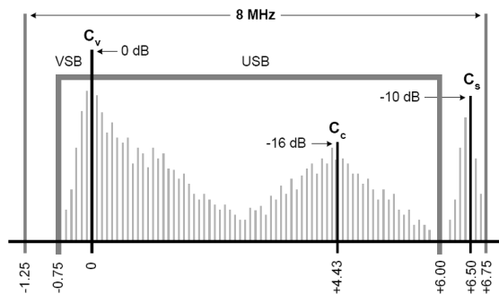
Figure 13-3 TV Standard - D, K
