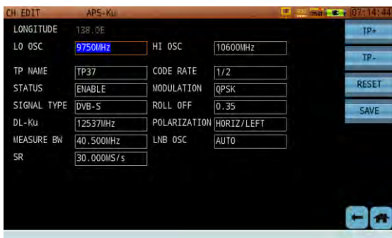
Figure 12-64 Satellite Transponder Setup Interface
