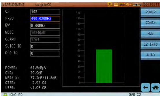
Figure 12-16 DVB-C2 Power Measurement
