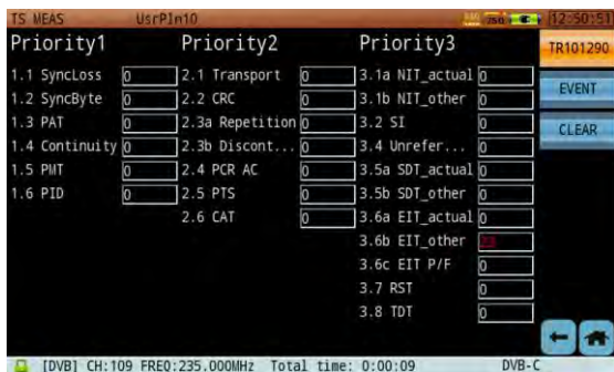
Figure 12-77 TR 101 290 Priority 1, 2 and 3 Tests
