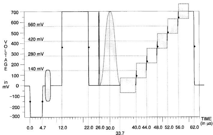
Figure 13-21 UK ITS1
