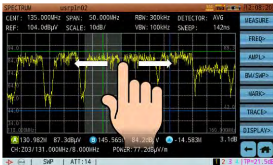
Figure 9-12 Change center frequency
