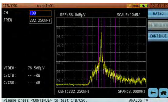
Figure 11-20 CSO/CTB Measurement-1
