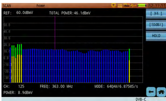
Figure 11-9 Channel SCAN
