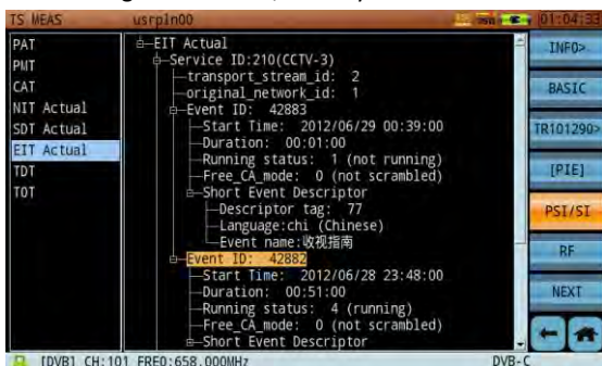
Figure 12-89 PSI/SI Analysis-EIT Table
