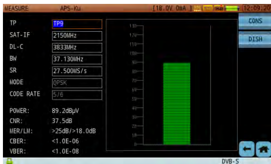
Figure 12-56 DVB-S Average Power Measurement
