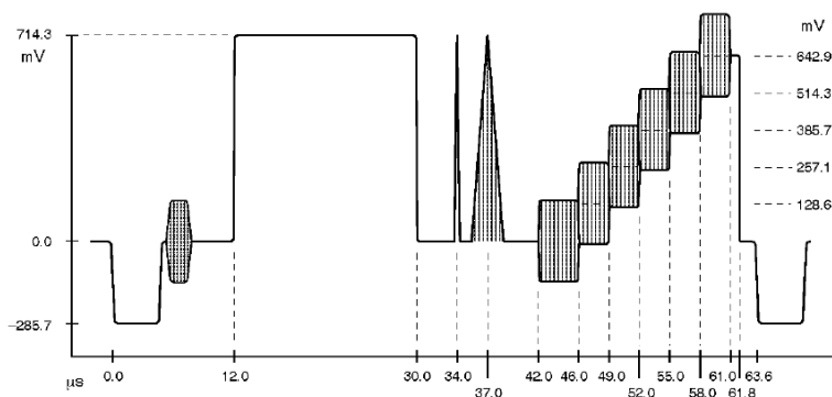
Figure 13-20 NTC-7 Composite
