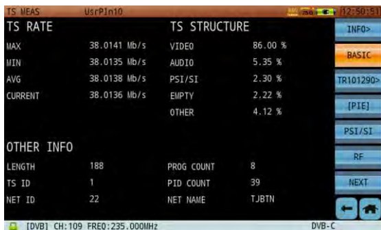
Figure 12-76 Transport Stream Basic Information
