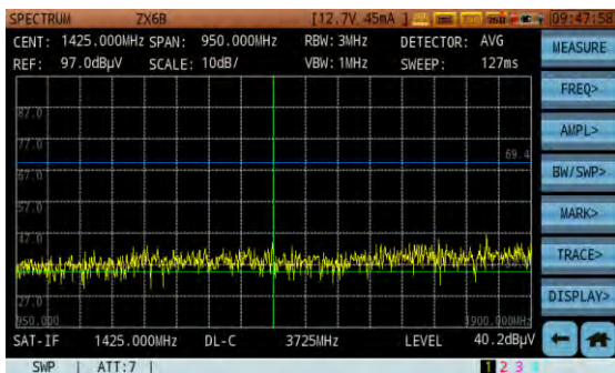
Figure 14-62 UB-2 Channel is Closed
