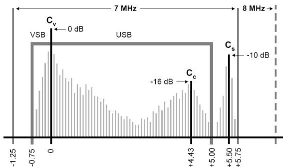
Figure 13-2 TV Standard - B, G
