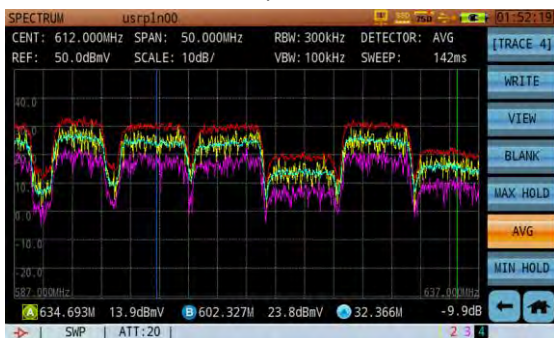
Figure 12-154 Snapshot : Four Traces Display Simultaneously
