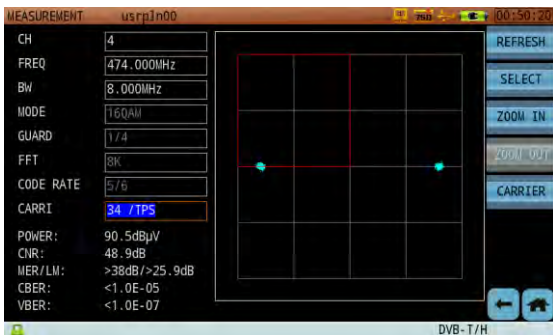
Figure 12-24 DVB-T/H Sub-Carrier Constellation - TPS
