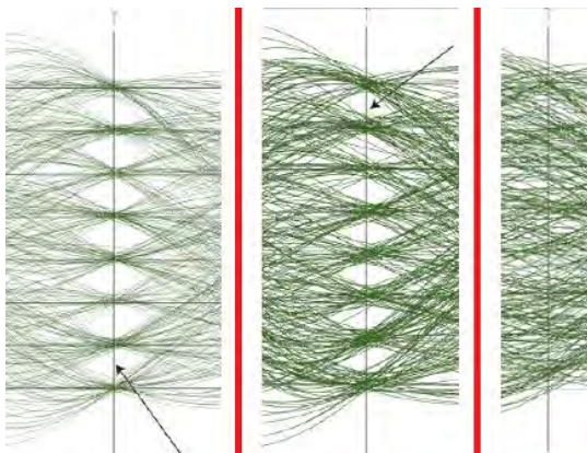
Figure 12-11 Decreased signal quality, eye diagram gradually closed
