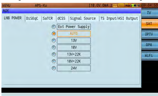
Figure 12-55 LNB Power Supply Control
