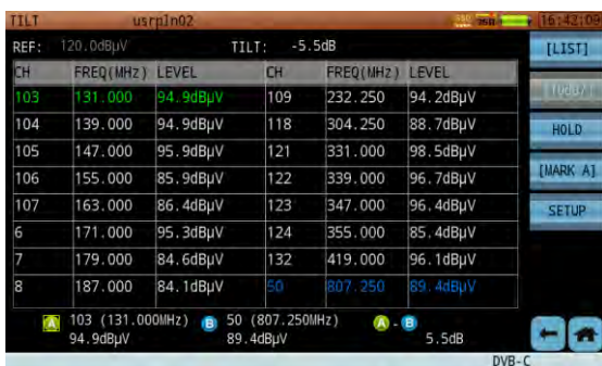
Figure 11-14 Tilt Measurement – Channel Listing Display
