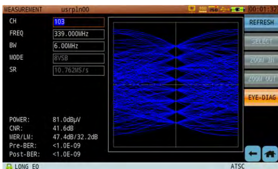
Figure 12-10 8VSB Diagram
