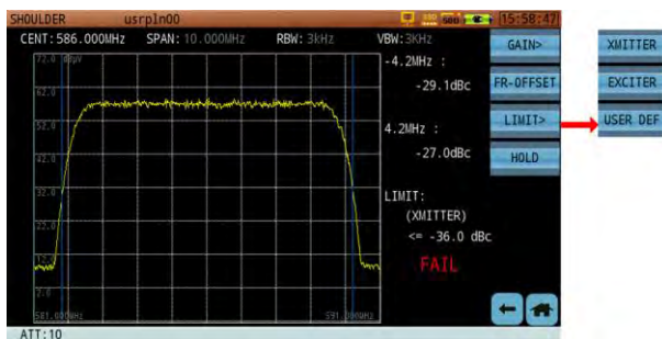
Figure 12-50 Limit Setting
