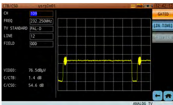
Figure 11-23 Gated CSO/CTB Measurement – Time Domain Waveform
