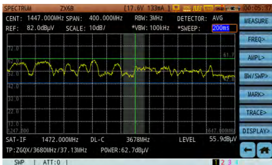
Figure 12-62 Satellite Signal IF Spectrum
