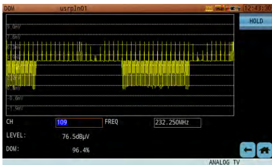
Figure 11-16 Snapshot: Depth of Modulation Measurement
