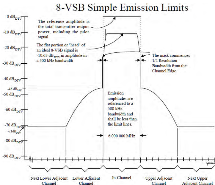
Figure 12-12 Simple Emissions Mask requirements for low power 8-VSB LPTV transmitters and translators
