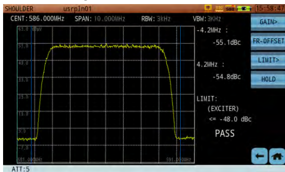
Figure 12-48 Actuator band shoulder test
