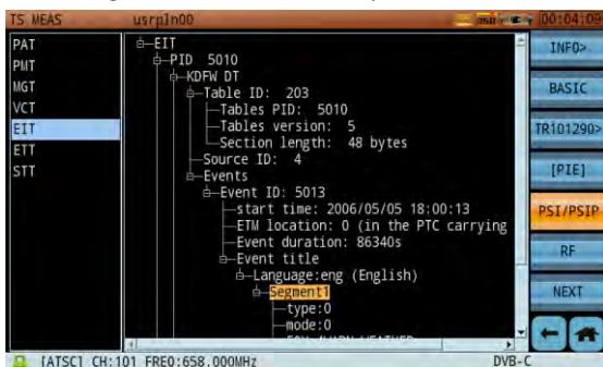
Figure 12-99 PSI/PSIP Analysis-EIT Table
