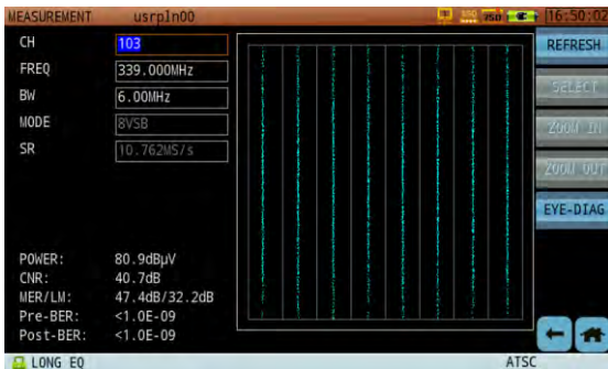
Figure 12-9 8VSB Constellation
