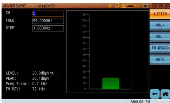
Figure 14-49 Opening Antenna Test
