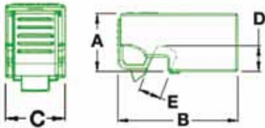
Snap-On
