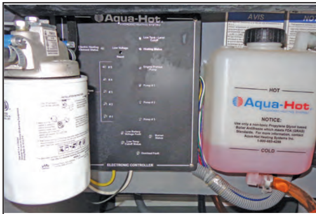
Figure 13-15: Surge tank
