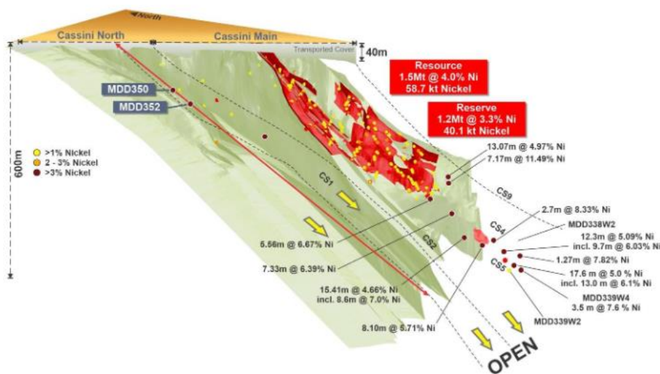
Figure 45. Cassini 3D image showing basalt surface and resource shapes with significant intersections
