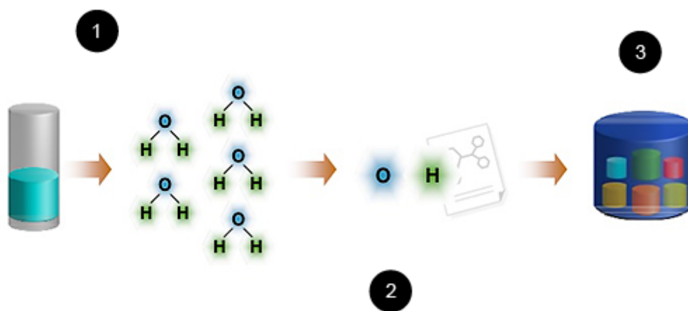
Figure 4. Data deduplication
