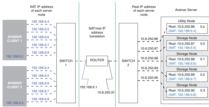
Figure 14. Multi-node server configuration with NAT
