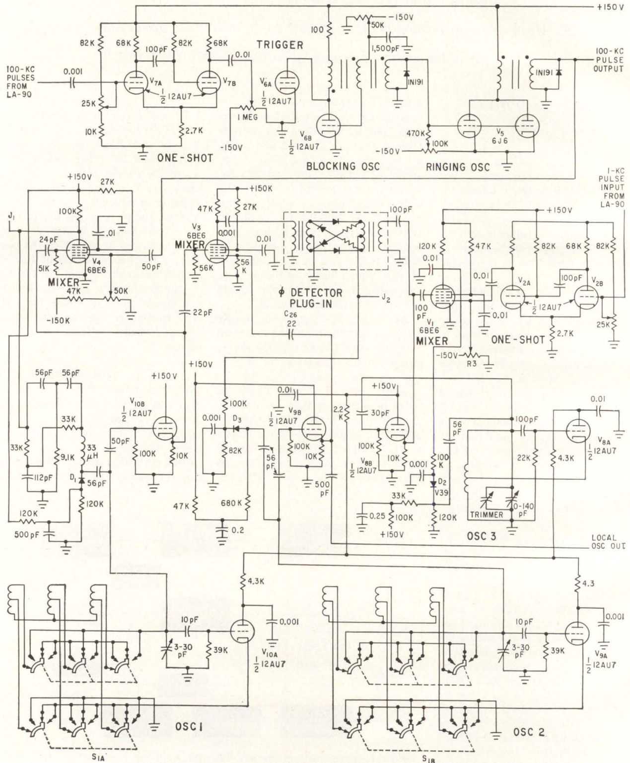
FIG. 2—Frequency controller requires extremely sharp pulses, so extensive shielding is necessary
