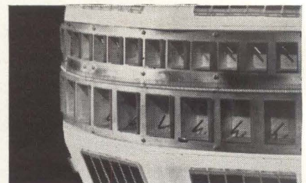
Section of satellite shows equatorial antenna slots. Upper row transmits, lower row receives microwave signals.
