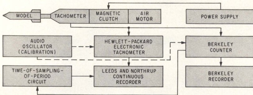
FIG. 2—Test setup for taking data on roll damping. Pulse-count data is fed to a computer (not shown), which calculates roll-damping coefficient
