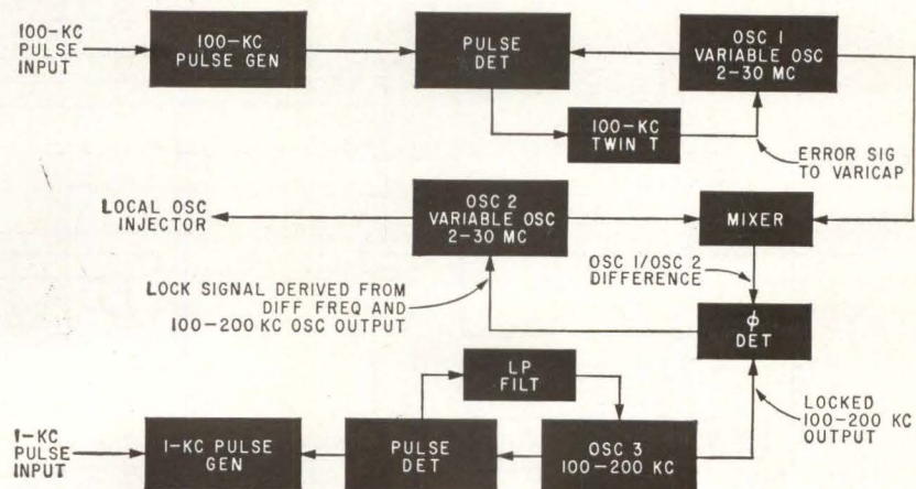
FIG. 1—Frequency controller. The 100-Kc pulse generator consists of a one-shot, trigger, blocking oscillator and ringing oscillator. Oscillator 2 is adjusted to 100 Kc from oscillator 1 frequency
