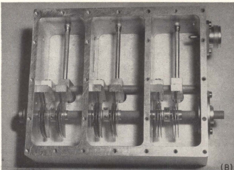
FIG. 4—Tuner uses epitaxial transistors to cover uhf/shf bands, operates up to 5,000 Mc (A); physical construction of the tuner (B). Table II gives test results
