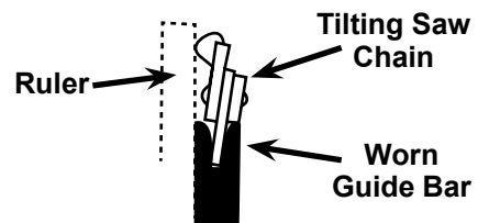
Figure U: Worn Guide Bar
