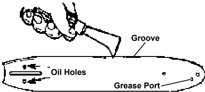
Figure S: Cleaning and Lubricating Guide Bar
