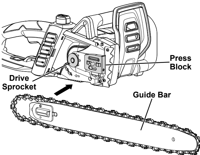
Figure F: Installing Chain Guide Bar
