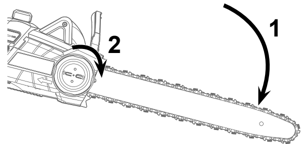
Figure H: Apply Pressure to Guide Bar Before Final Tightening
