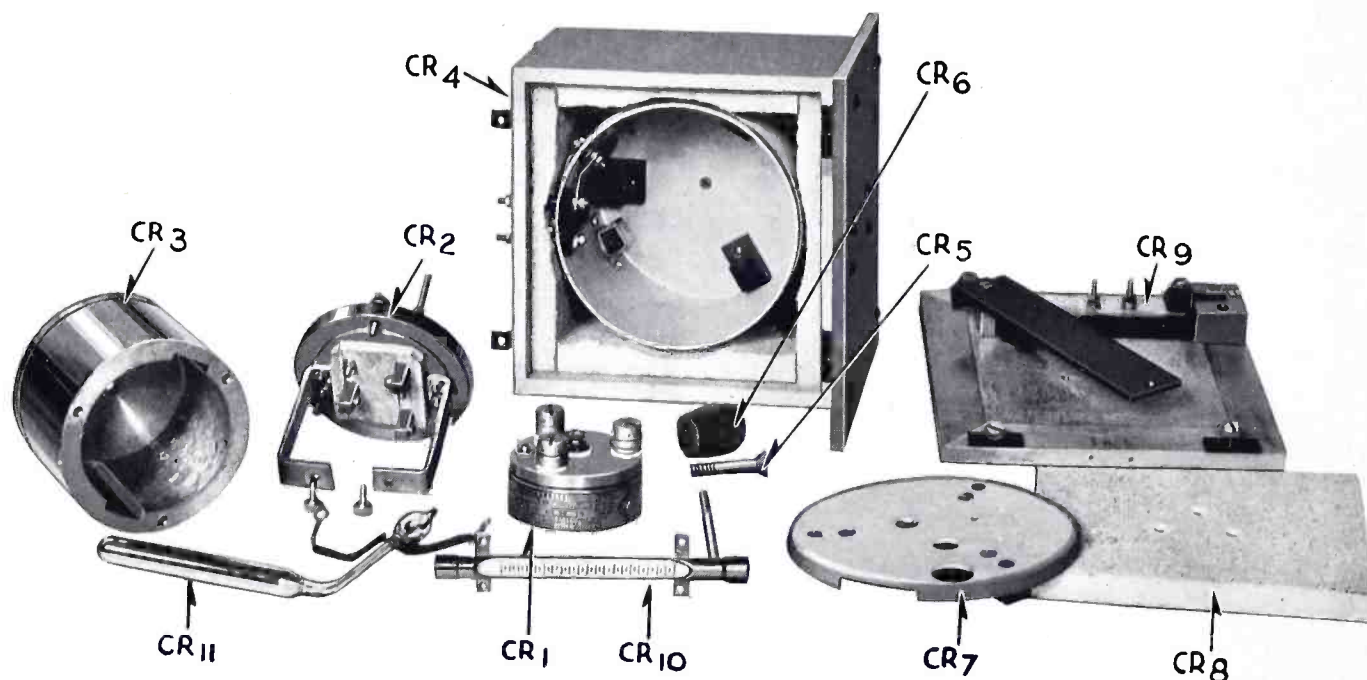
FIG. 1—PARTS COMPRISING CRYSTAL BOX ASSEMBLY
