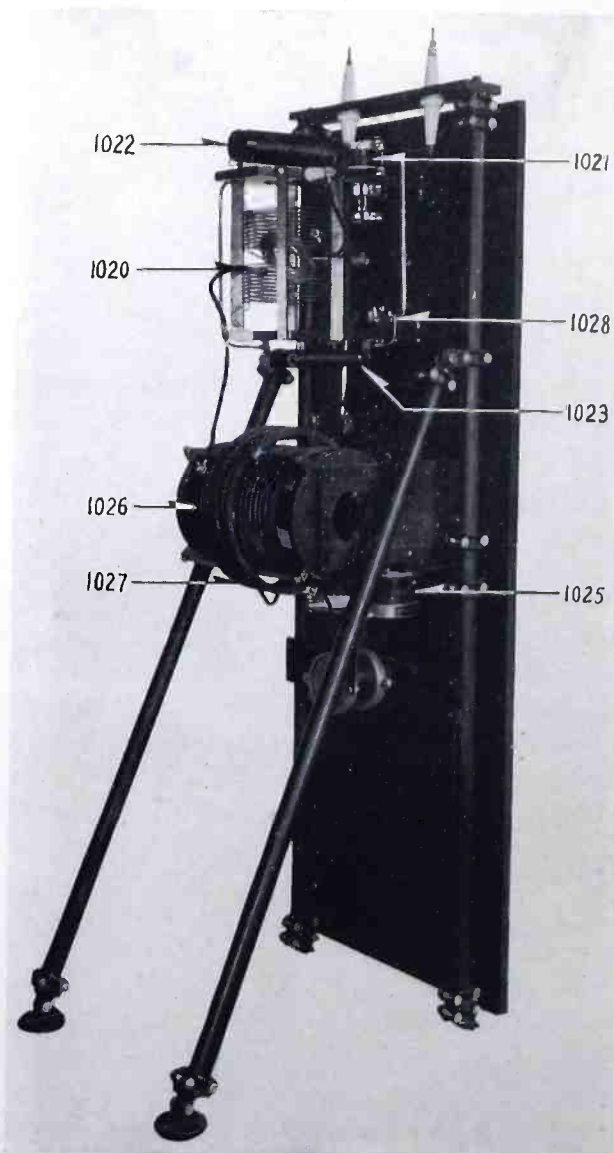
FIG. 17—ANTENNA TUNING AND COUPLING UNIT (Rear View)
