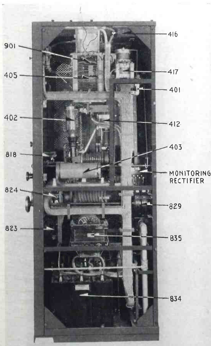
FIG. 14—POWER AMPLIFIER AND CONTROL UNIT (Right Side)
