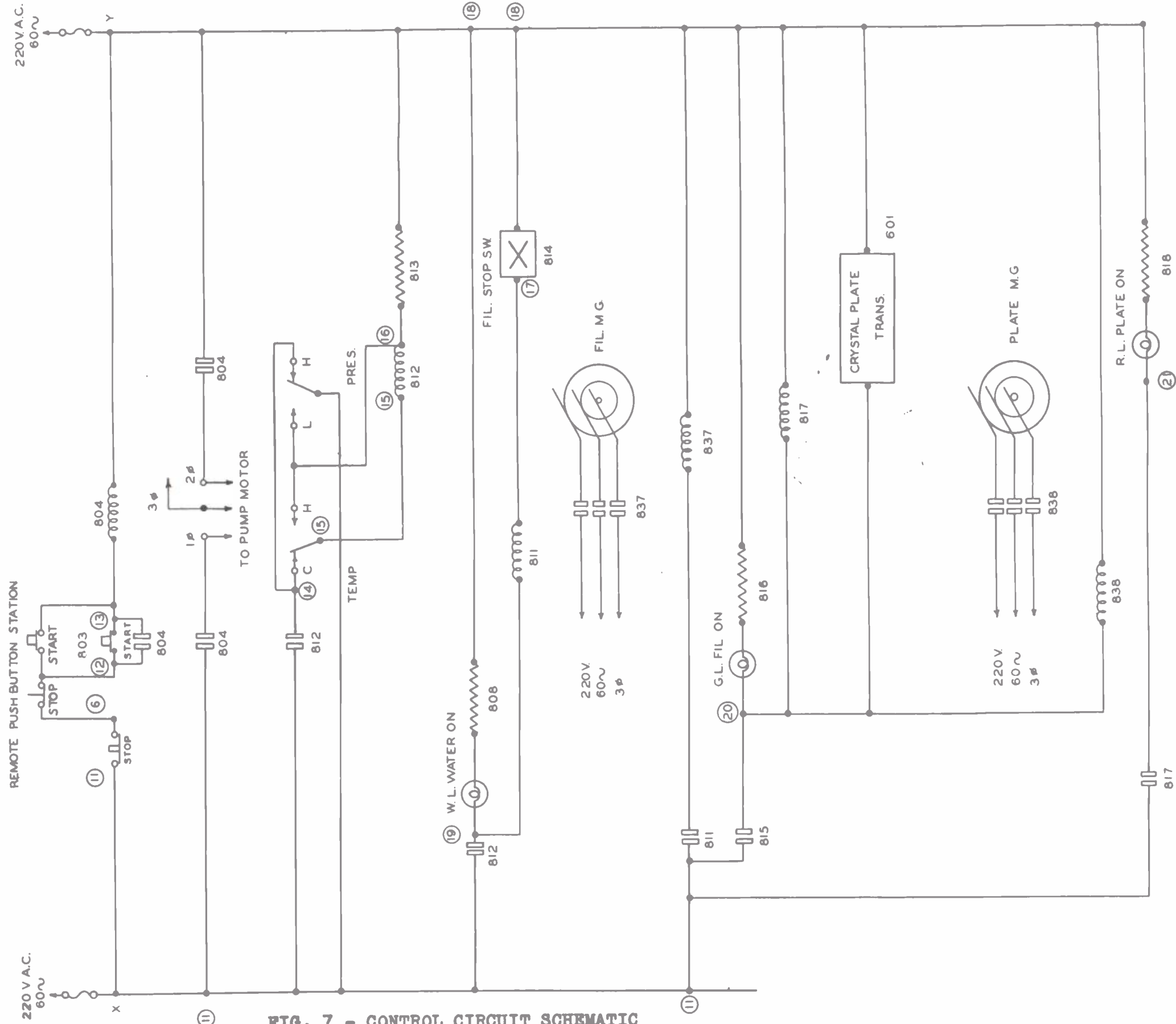
FIG. 7 - CONTROL CIRCUIT SCHEMATIC DWG. P-7703724
