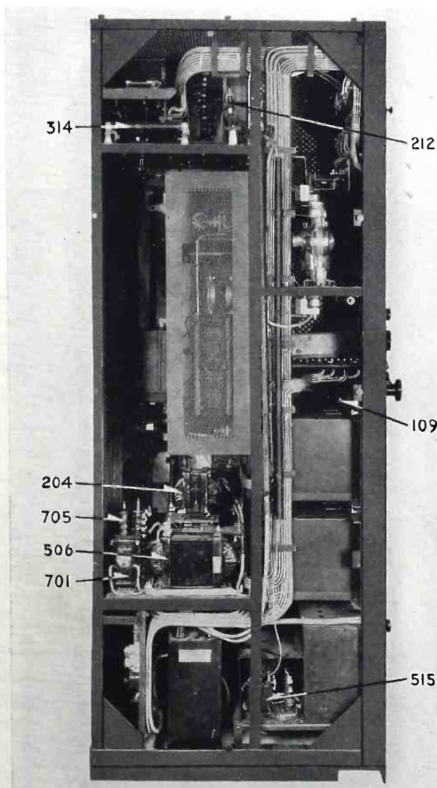
FIG. 10—MODULATOR EXCITER UNIT (Left Side View)
