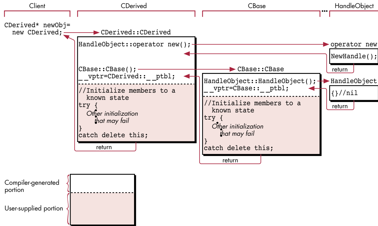
Figure 2 Flow of Control During C++ Object Instantiation
