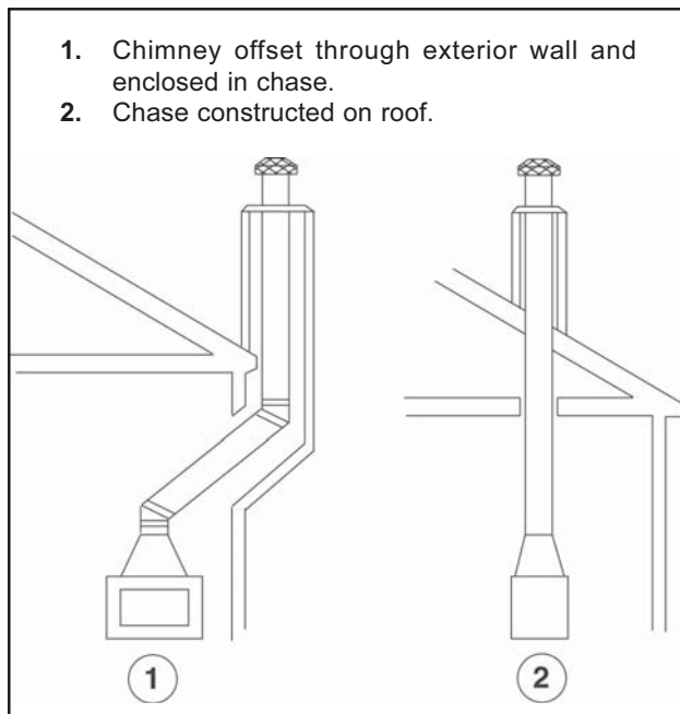
Figure 20 - Chase Constructions
