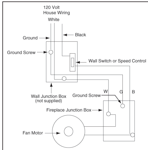
Figure 14 - Blower Wiring
