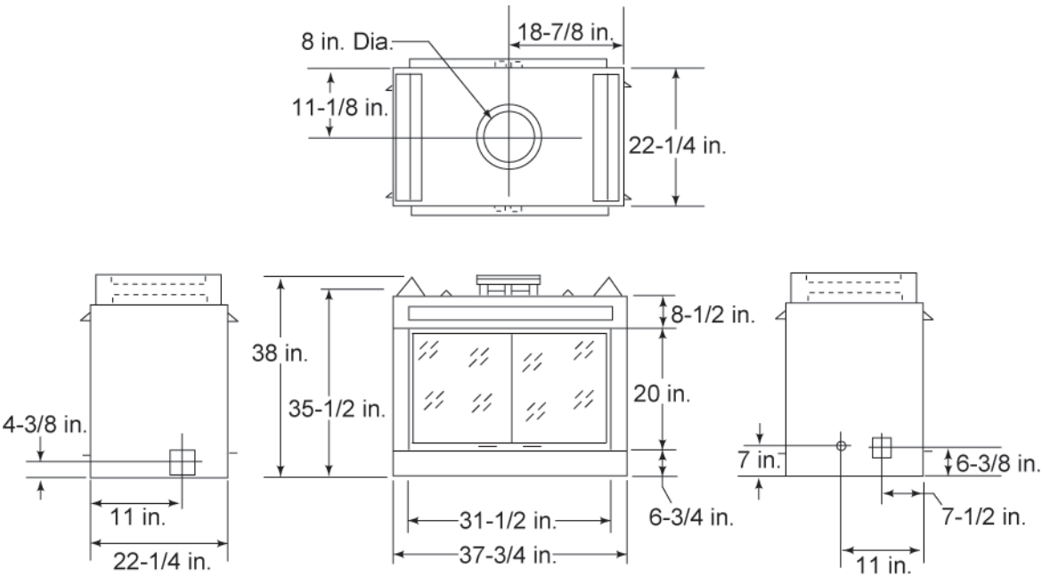
Fireplace Dimensions
