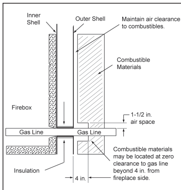
Figure 16 - Air Clearance Around Gas Line
