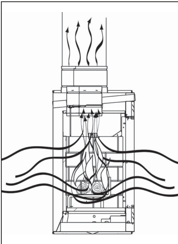
Figure 27 - Flue Draft
