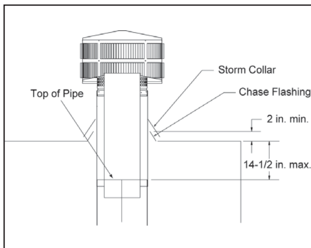
Figure 23 - Installing a TR342 Round Telescoping Termination Cap
