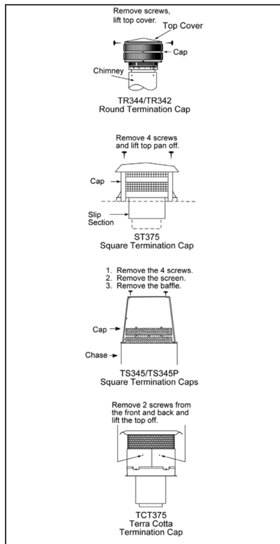
Figure 28 Chimney and Termination Cap Cleaning
