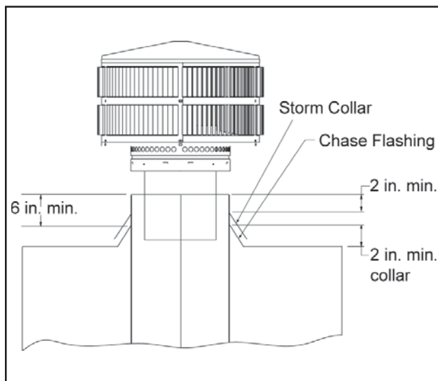
Figure 22 - Installing a TR344 Round Termination Cap
