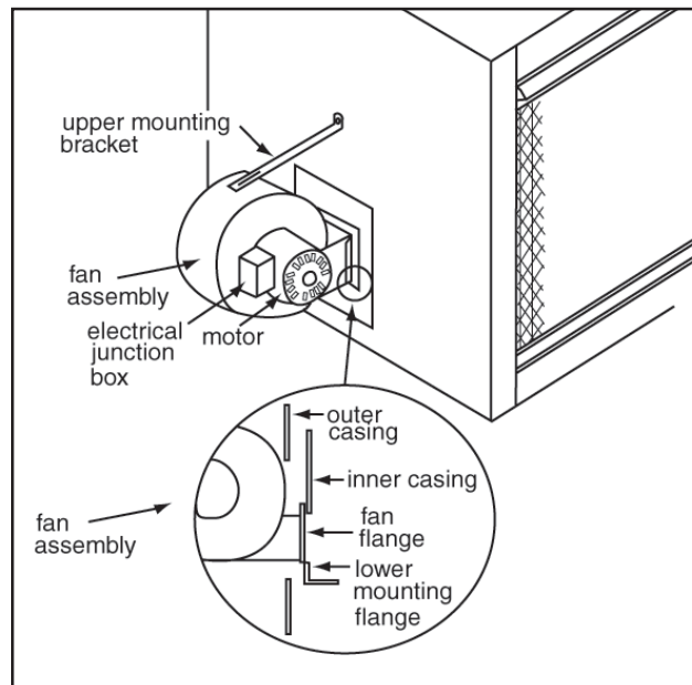
Figure 15 - Fan Mount
