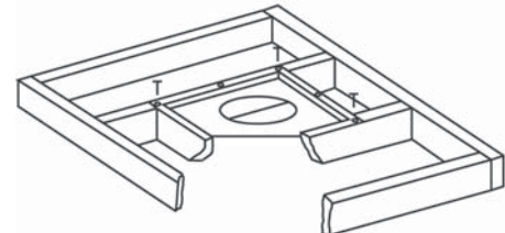
Figure 9 Installing the Firestop Spacer
