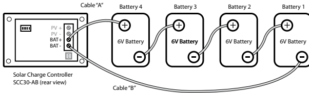
Fig. 3.2. Series Connection
