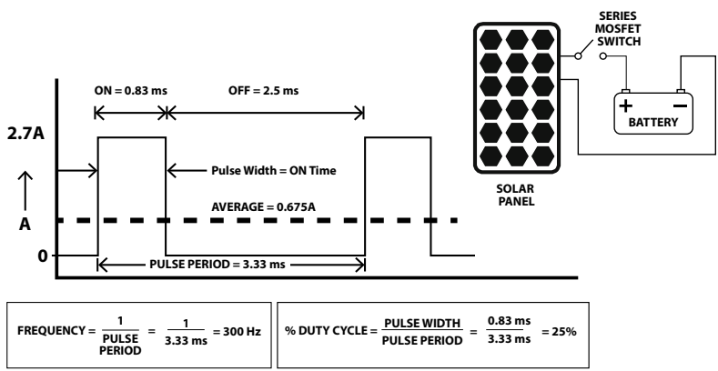
Fig. 4.1. Series Type PWM Control - PWM Frequency = 300 Hz
