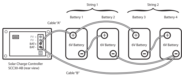
Fig. 3.4. Series-Parallel Connection
