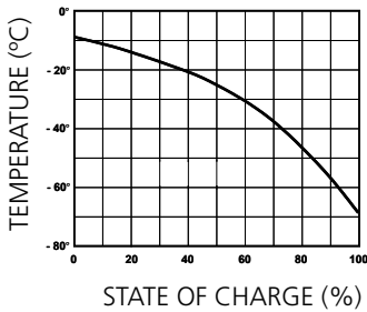
Fig 3.1. Temperature vs State of Charge
