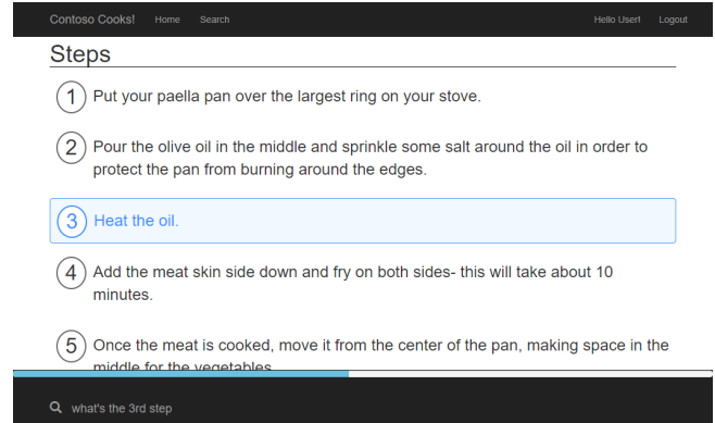
Figure 3: Screenshot of the AskChef application visual interface for first-party content (in this case an internal cooking website created for demonstration purposes). In this example, the system has highlighted the current step (Step 3) in response to a user voice request (“what’s the 3rd step?”).
