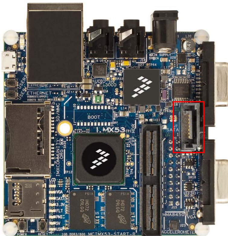
Figure 9. SATA Data Connector (J7)
