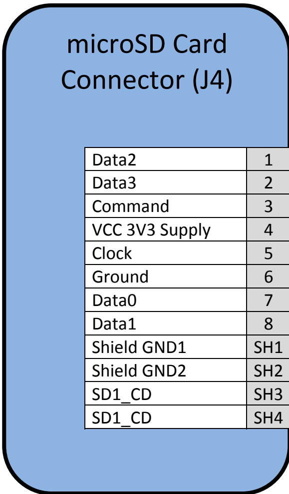
Figure 30. microSD Card Connector (J4)
