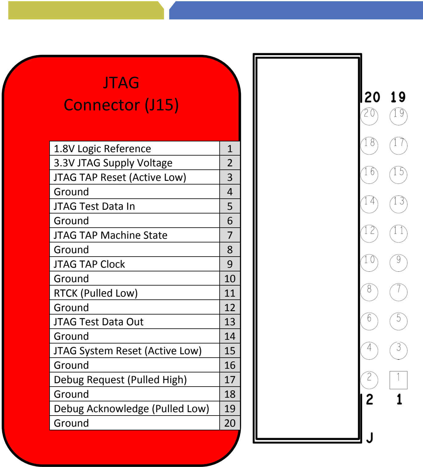
Figure 32. JTAG Connector (J15)
