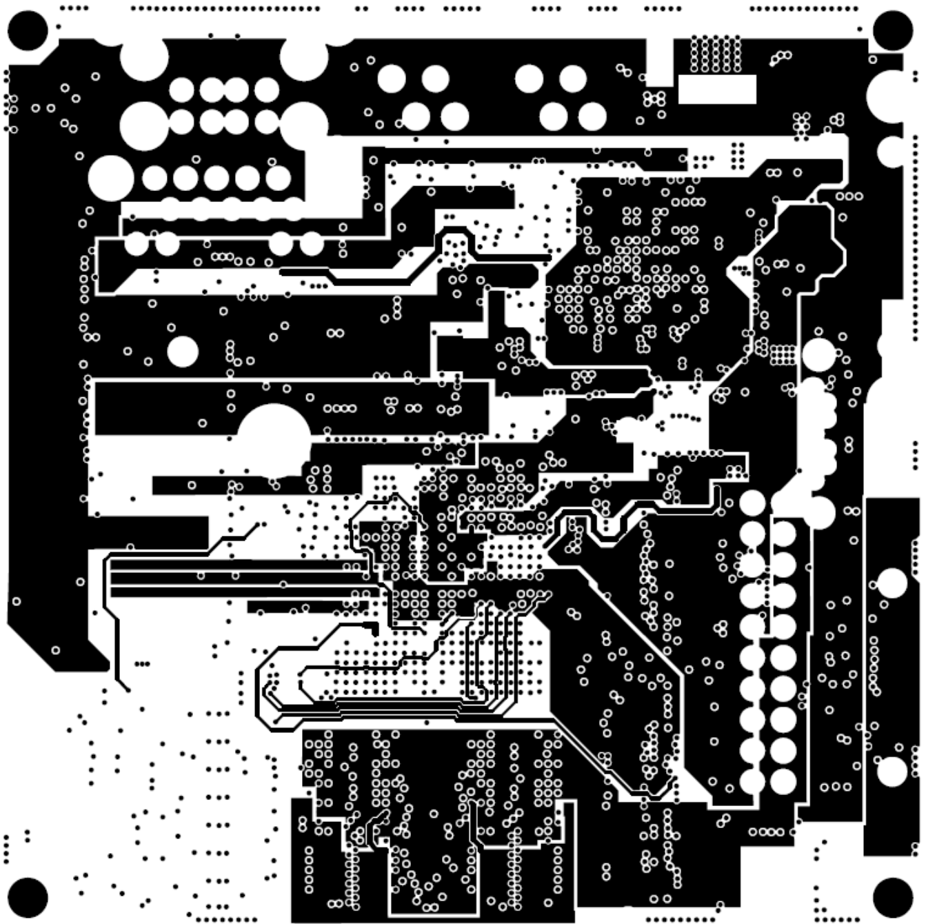
Figure 64. Fifth Etch Layer
