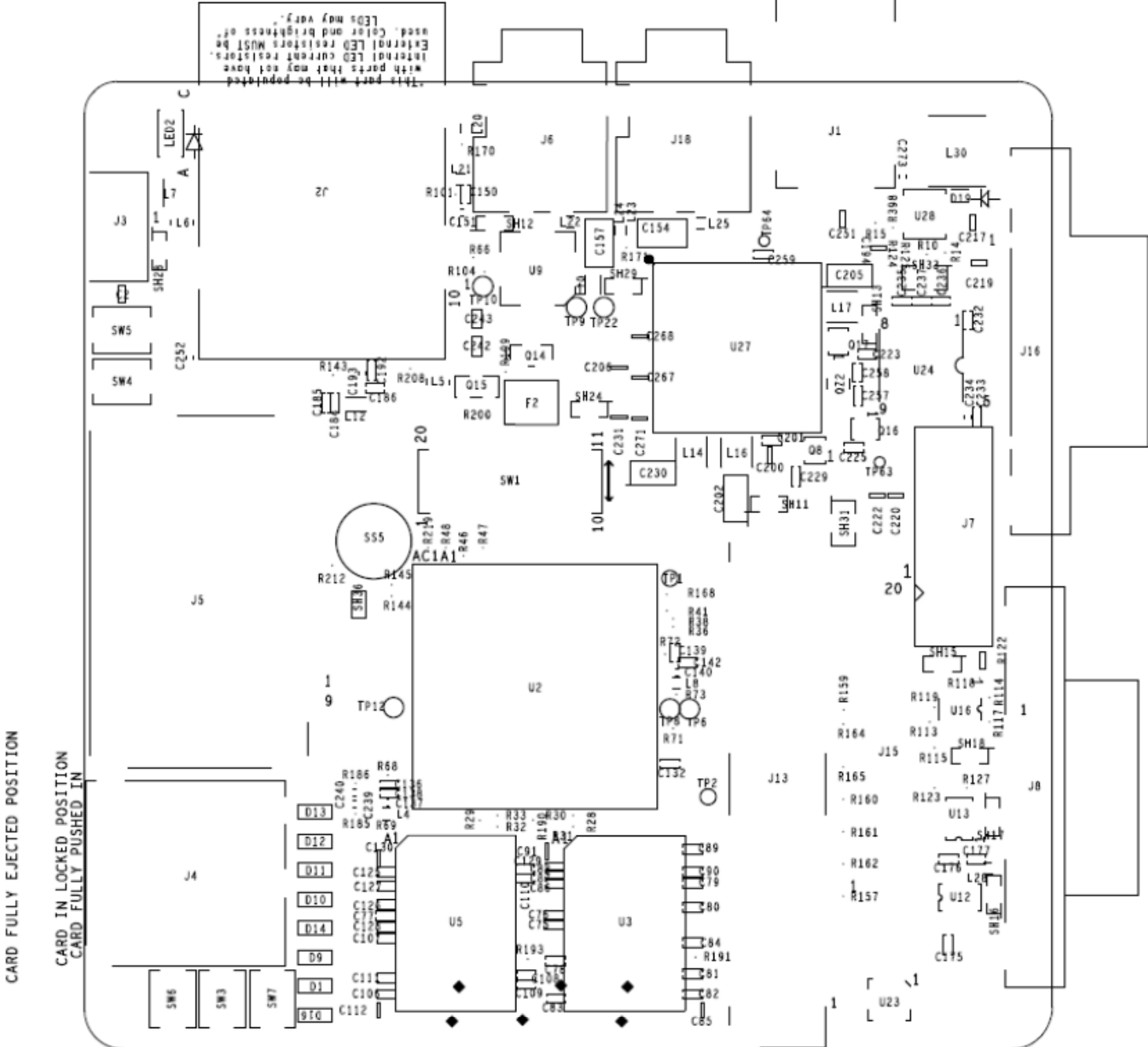
Figure 44. Assembly Drawing Top
