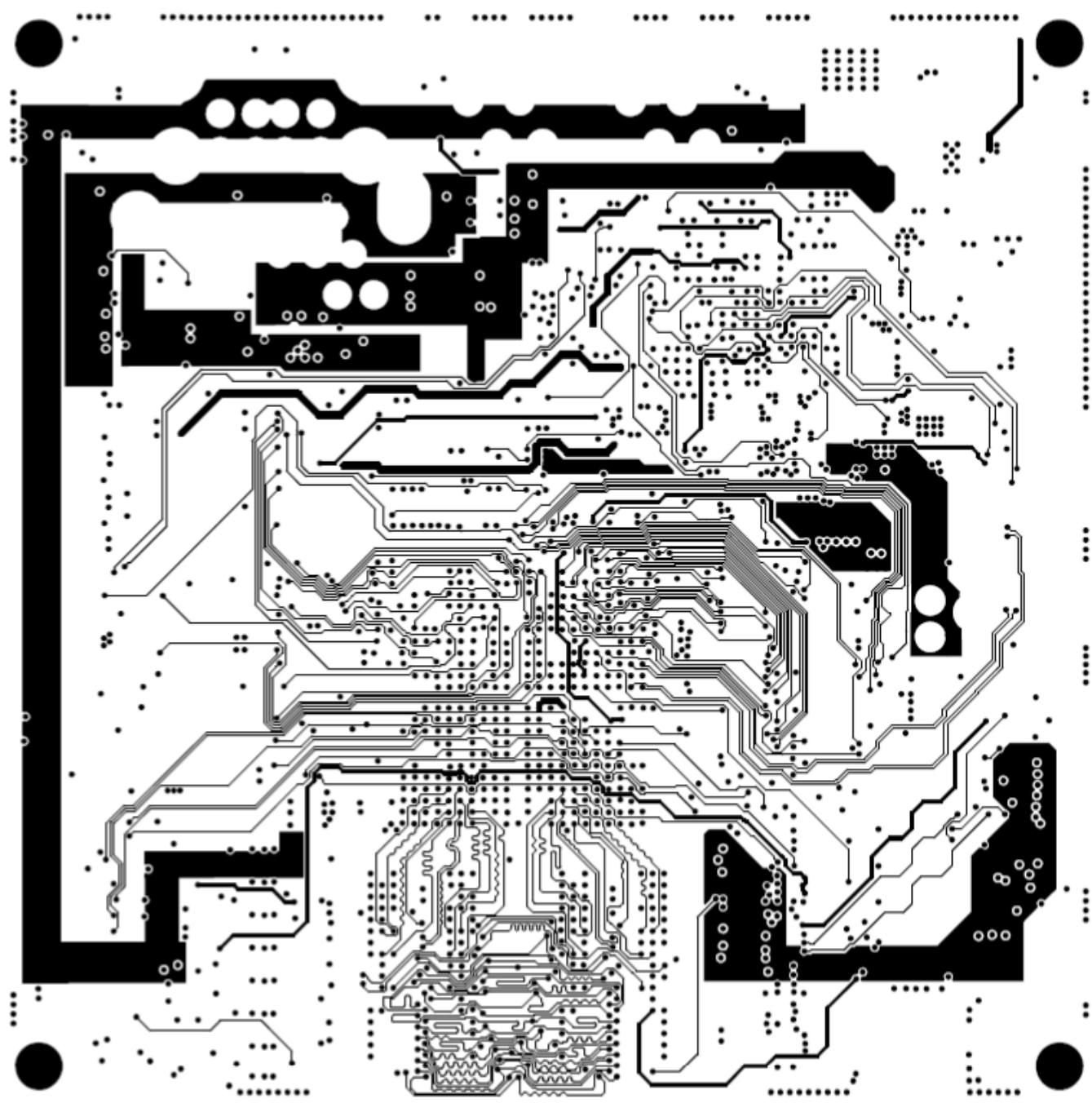
Figure 62. Third Etch Layer
