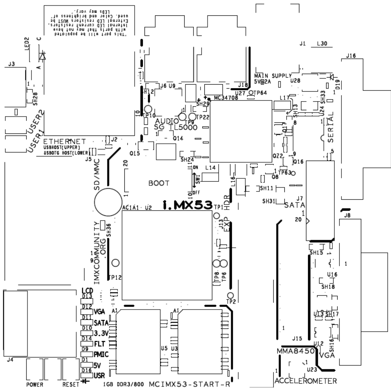
Figure 72. Silkscreen Top
