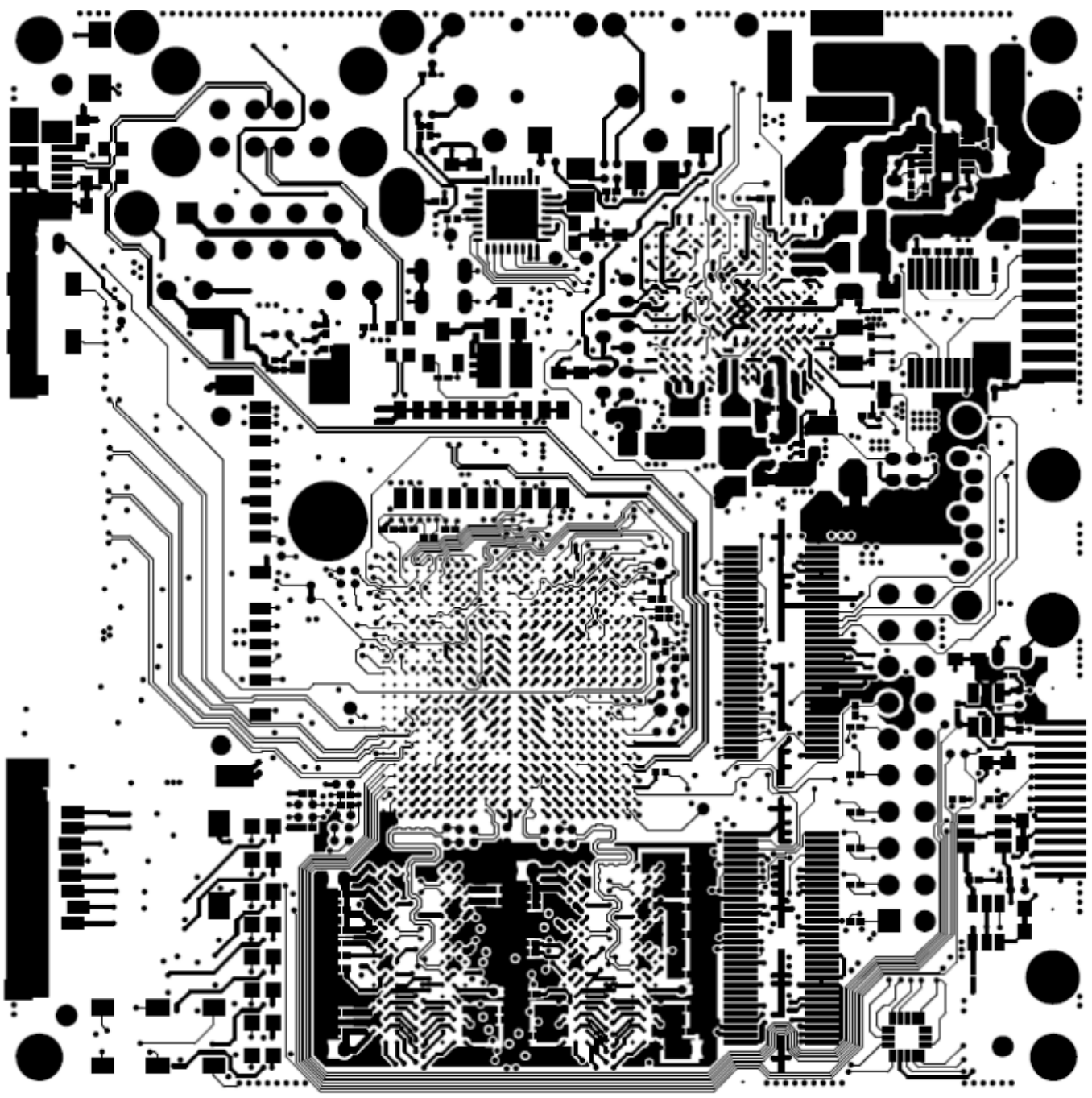
Figure 60. Top Etch Layer
