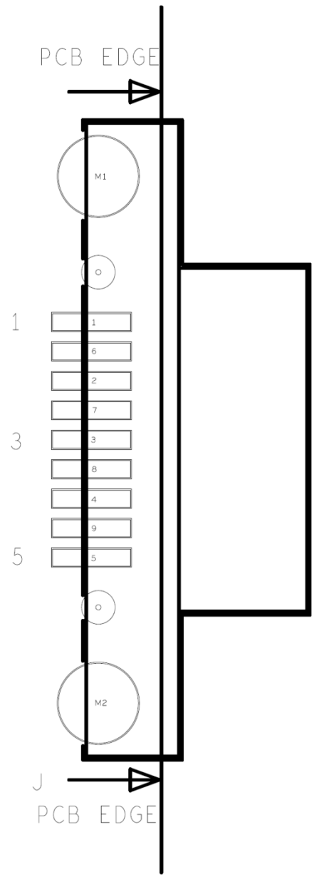
Figure 31. Debug UART Connector (J16)
