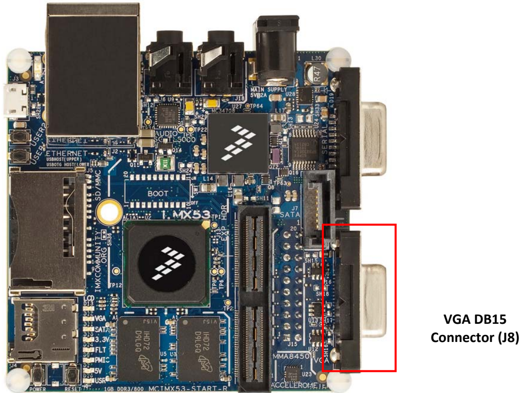
Figure 3. VGA Connector
