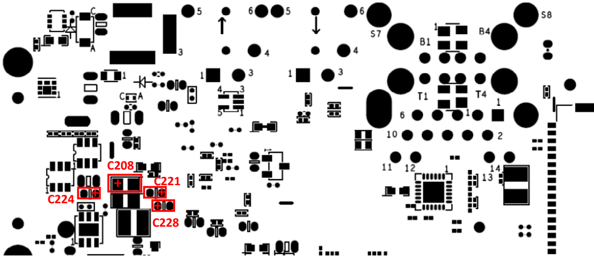
Figure 40. Regulator Output Capacitor Positions Bottom
