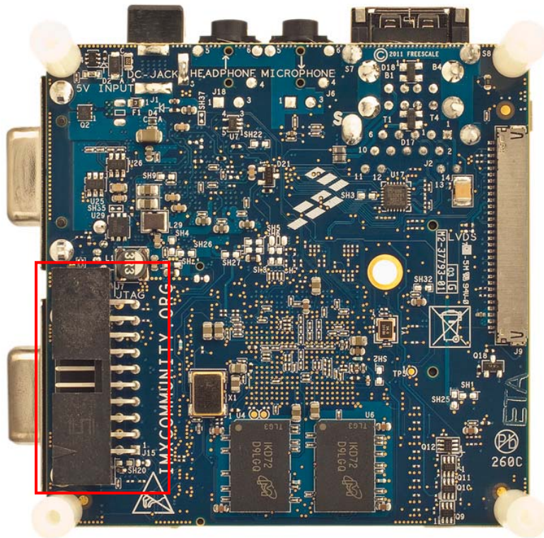
Figure 12. JTAG Connector (J15)
