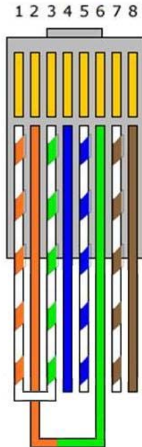
Figure 39. Ethernet Loopback Cable
