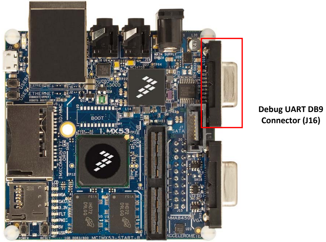
Figure 4. Debug UART Connector
