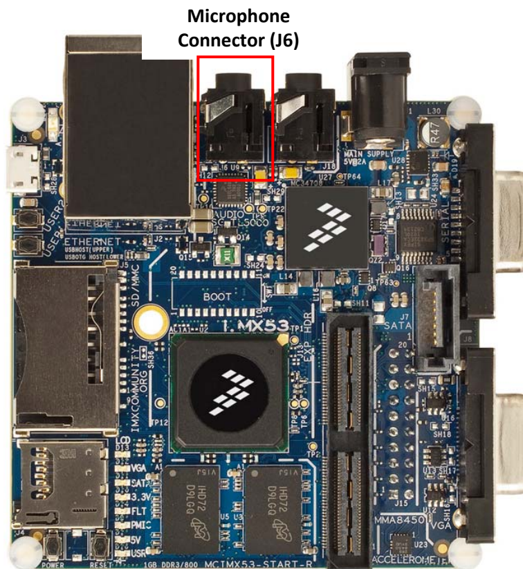
Figure 6. Microphone Connector (J6)
