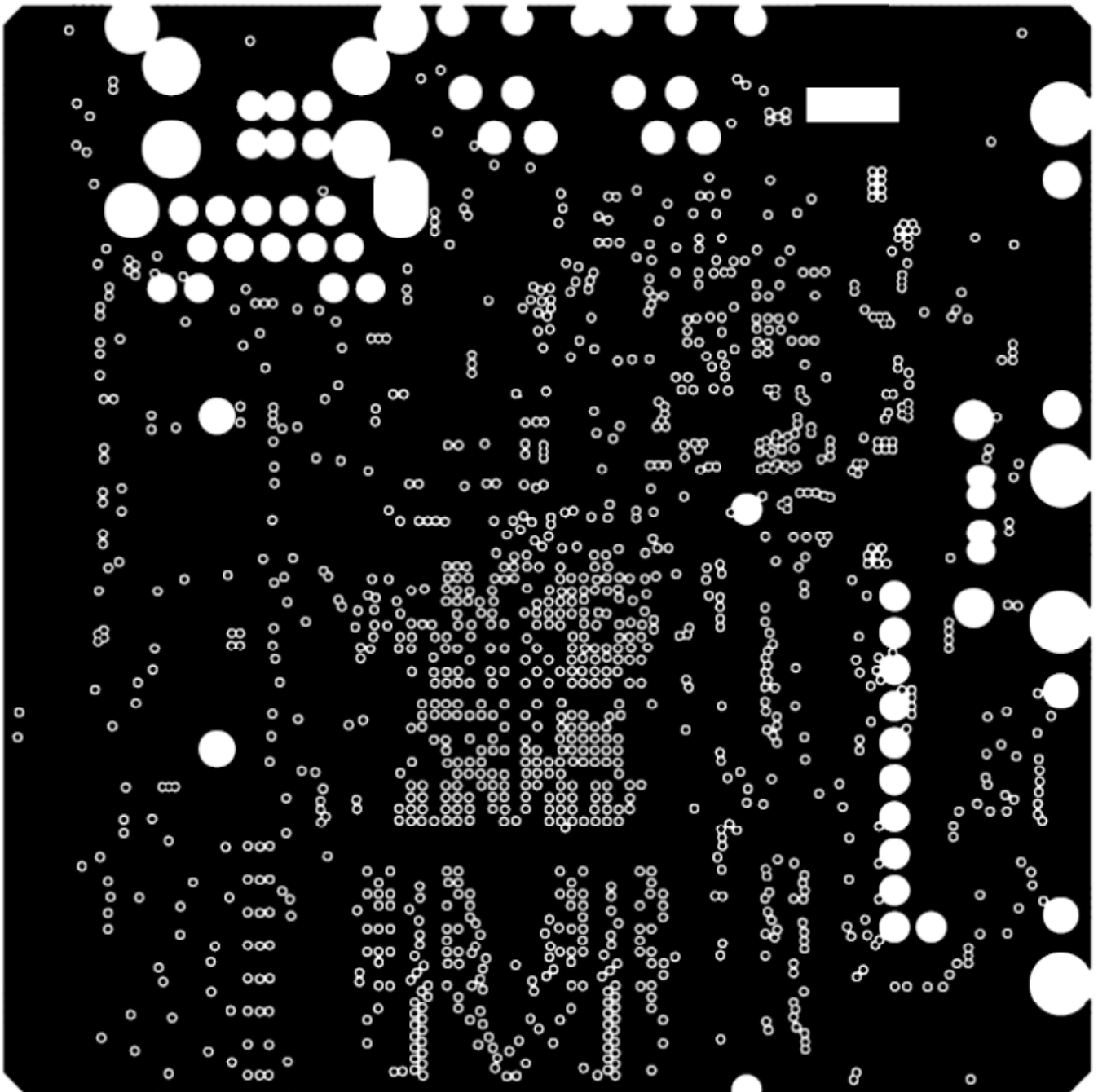
Figure 66. Seventh Etch Layer
