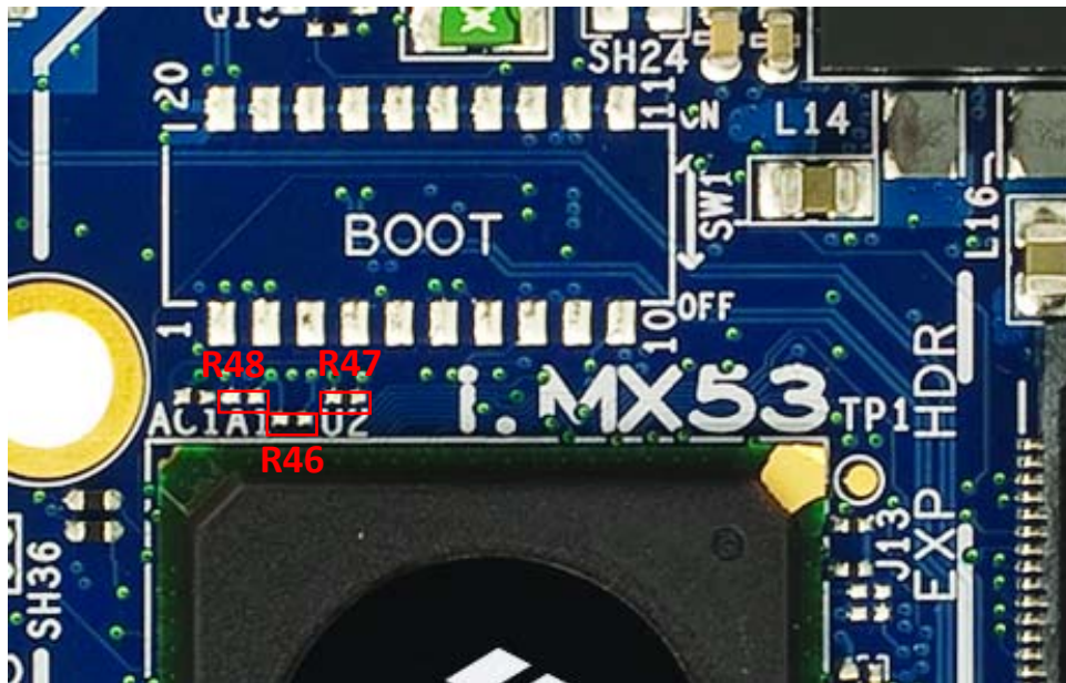
Figure 18. Boot Mode Resistor Locations TOP
