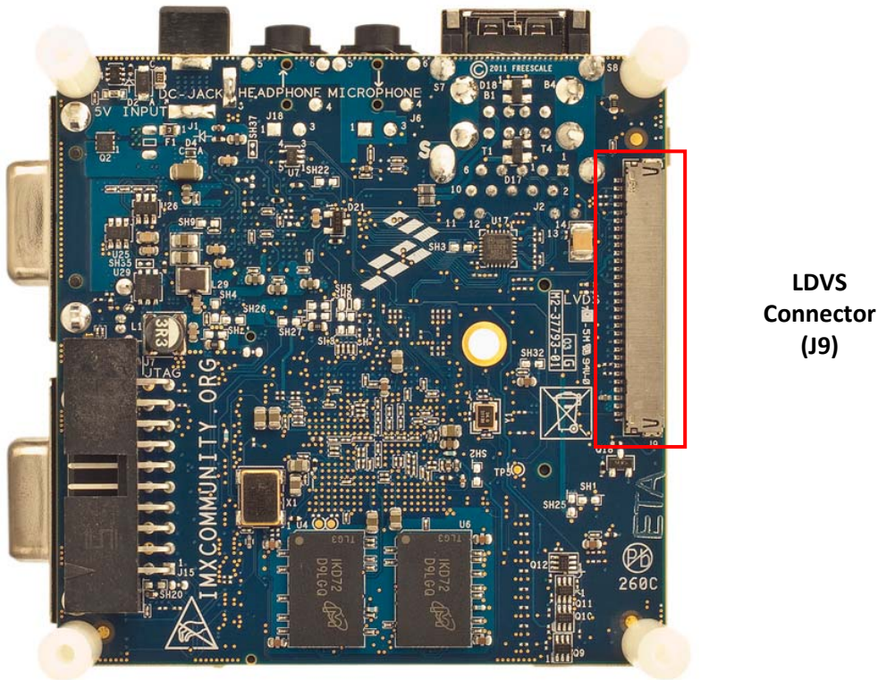
Figure 13. LVDS Connector (J9)
