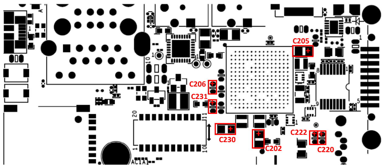
Figure 41. Regulator Output Capacitor Positions Top
