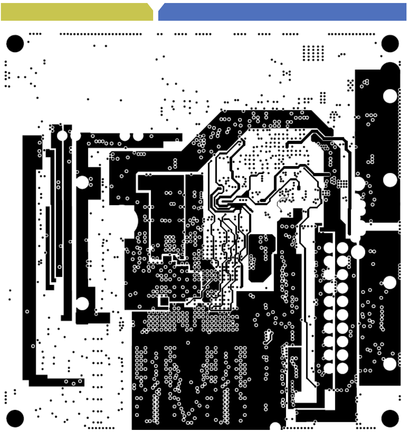
Figure 63. Fourth Etch Layer
