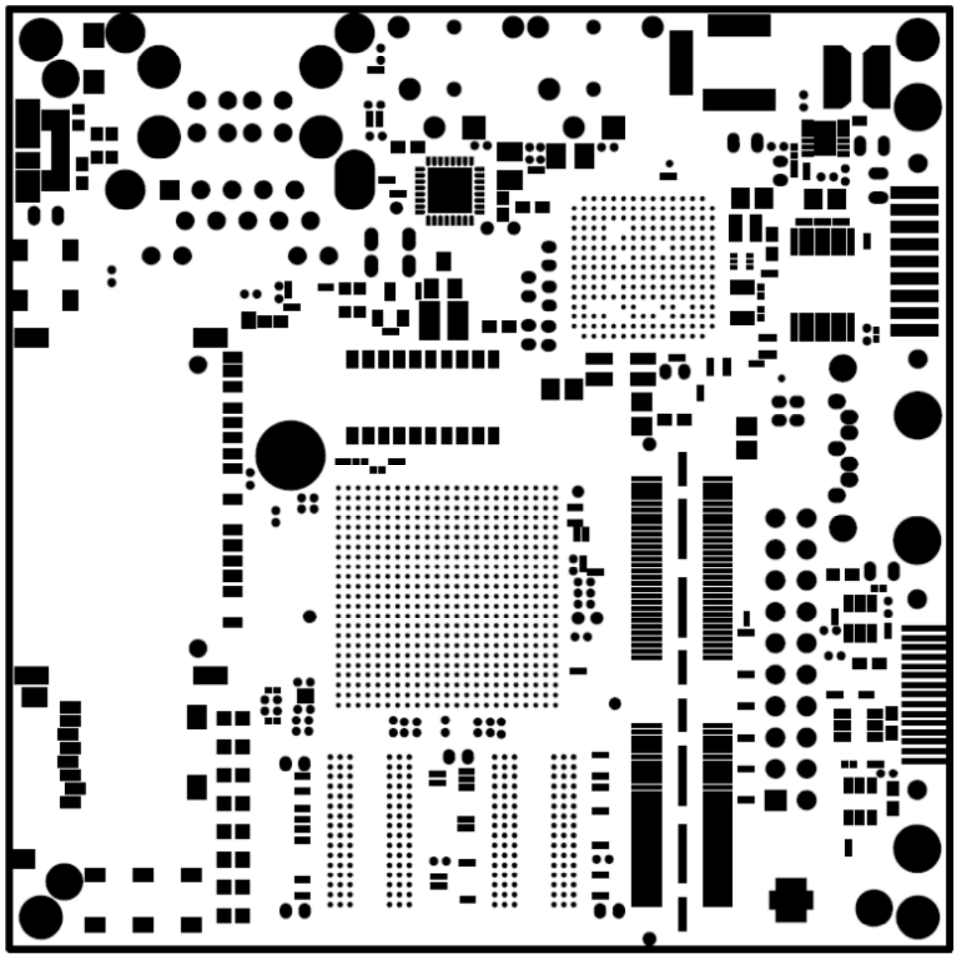
Figure 68. Soldermask Top
