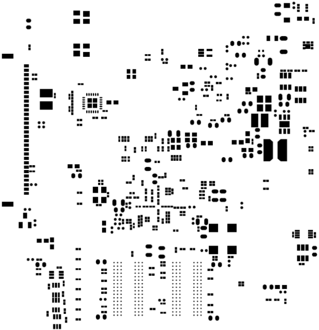
Figure 71. Pastemask Bottom
