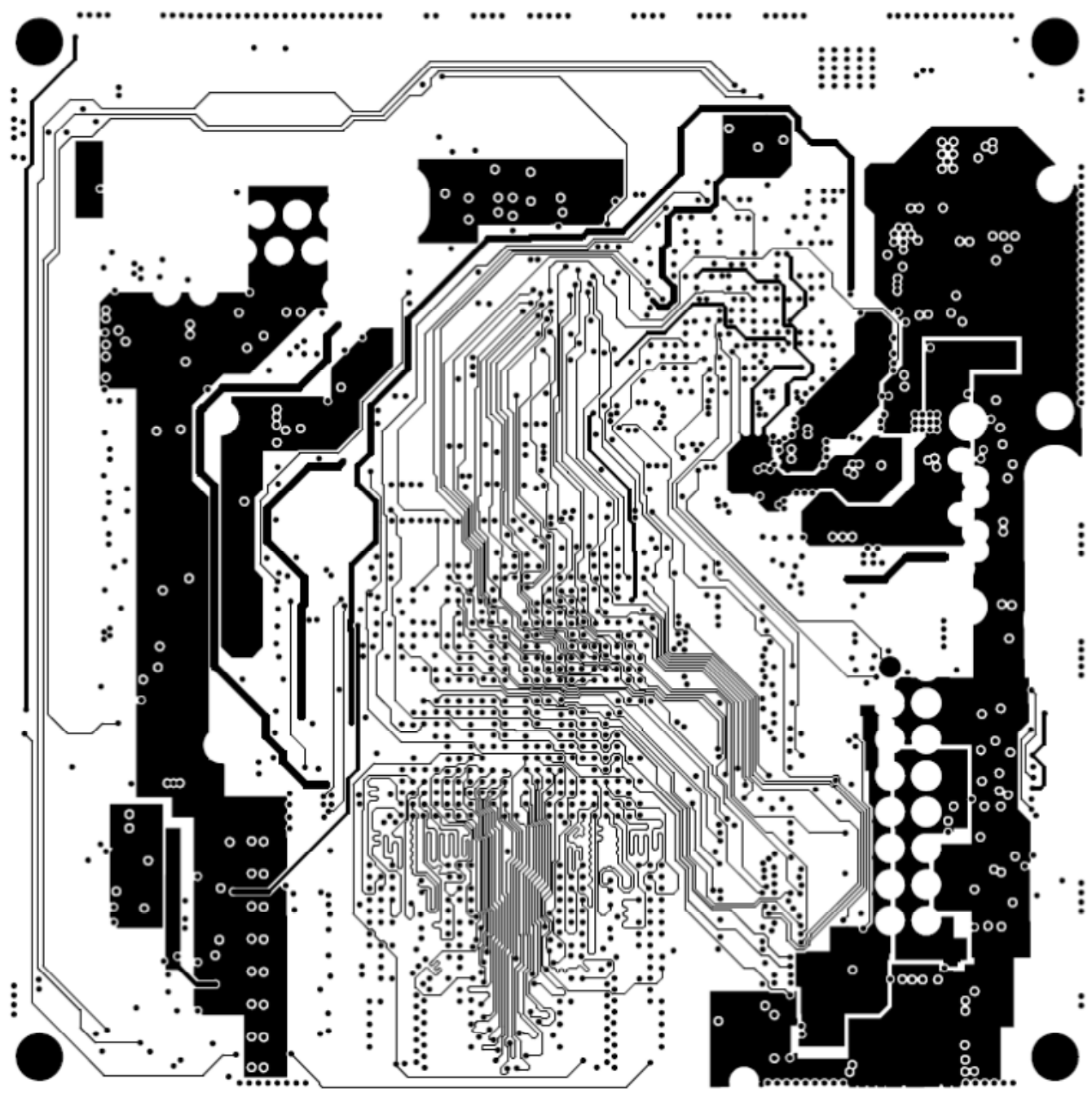
Figure 65. Sixth Etch Layer
