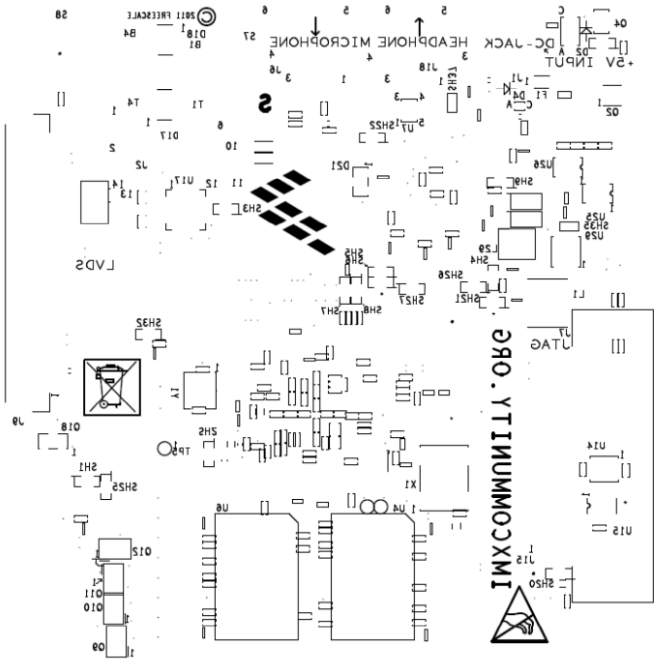
Figure 73. Silkscreen Bottom
