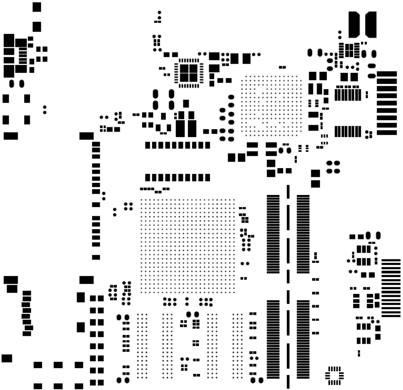
Figure 70. Pastemask Top
