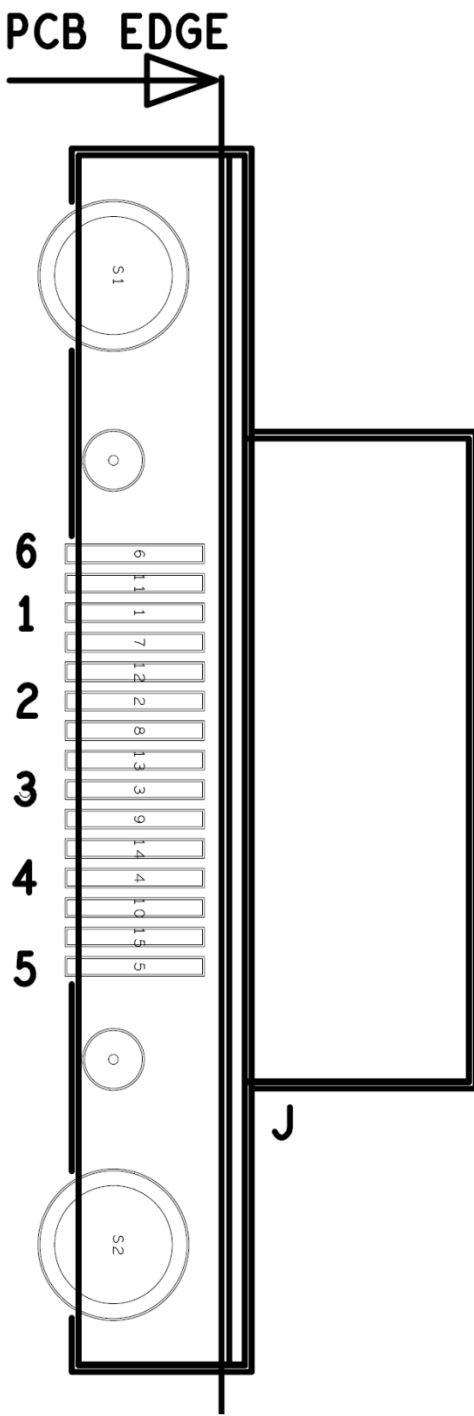
Figure 26. VGA DB15 Connector (J8)
