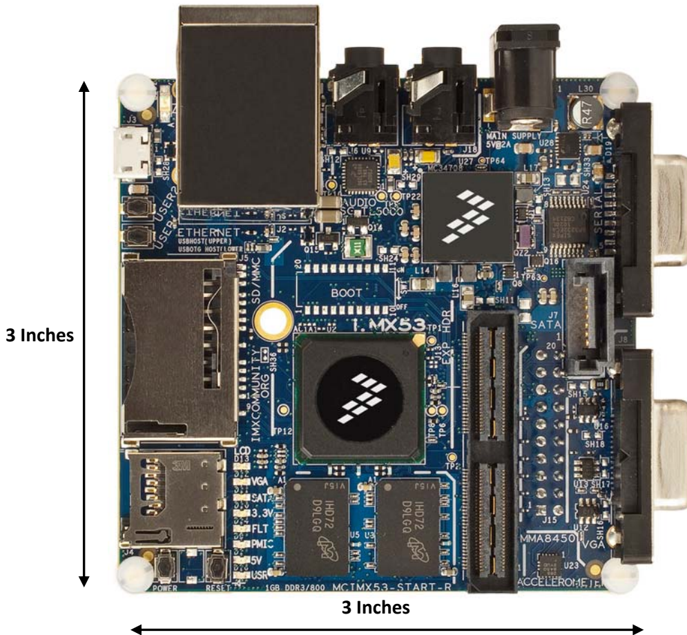
Figure 38. Quick Start Board Dimensions
