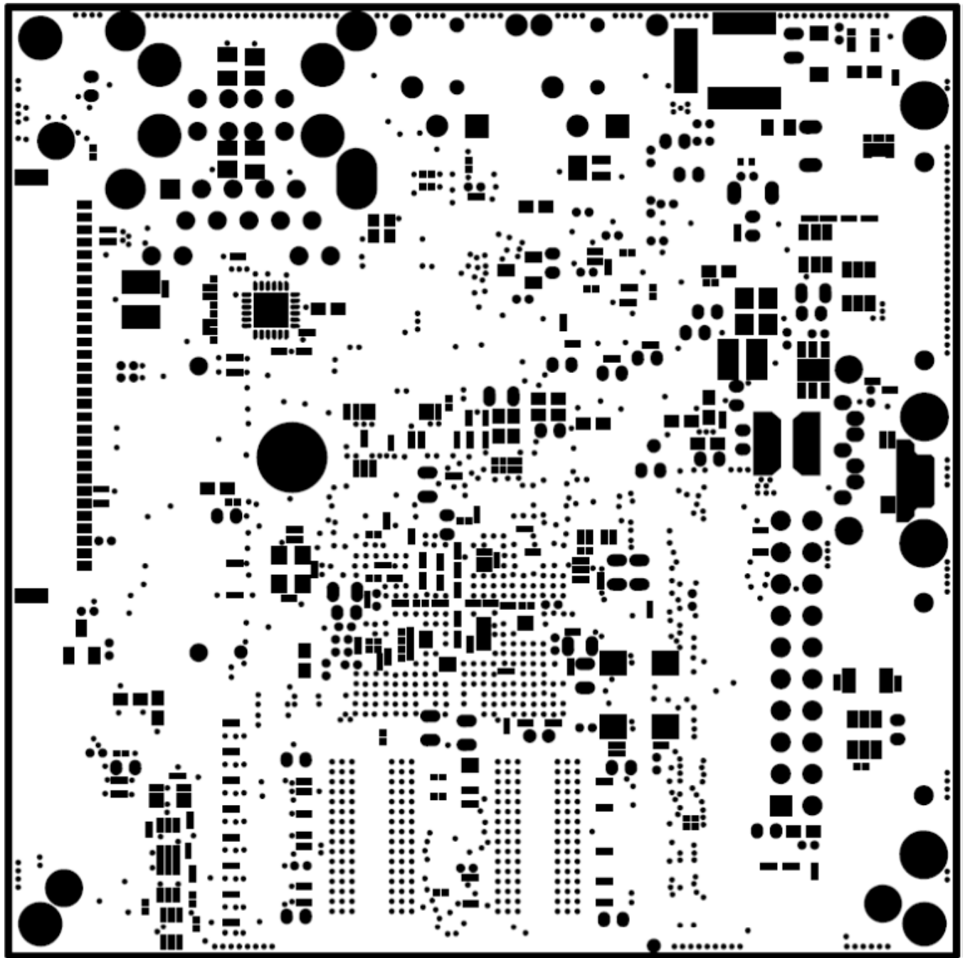
Figure 69. Soldermask Bottom
