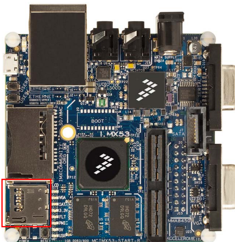
Figure 11. MicroSD Card Connector (J4)
