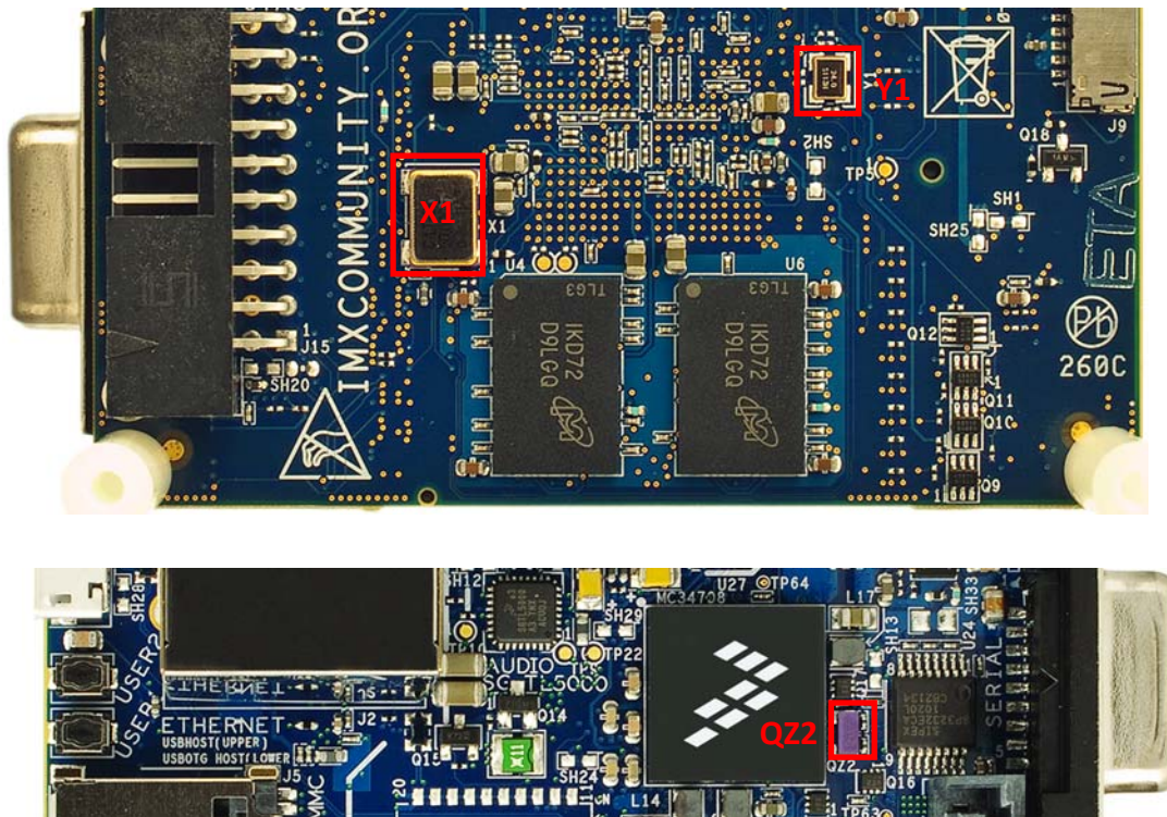
Figure 20. Clock Source Locations
