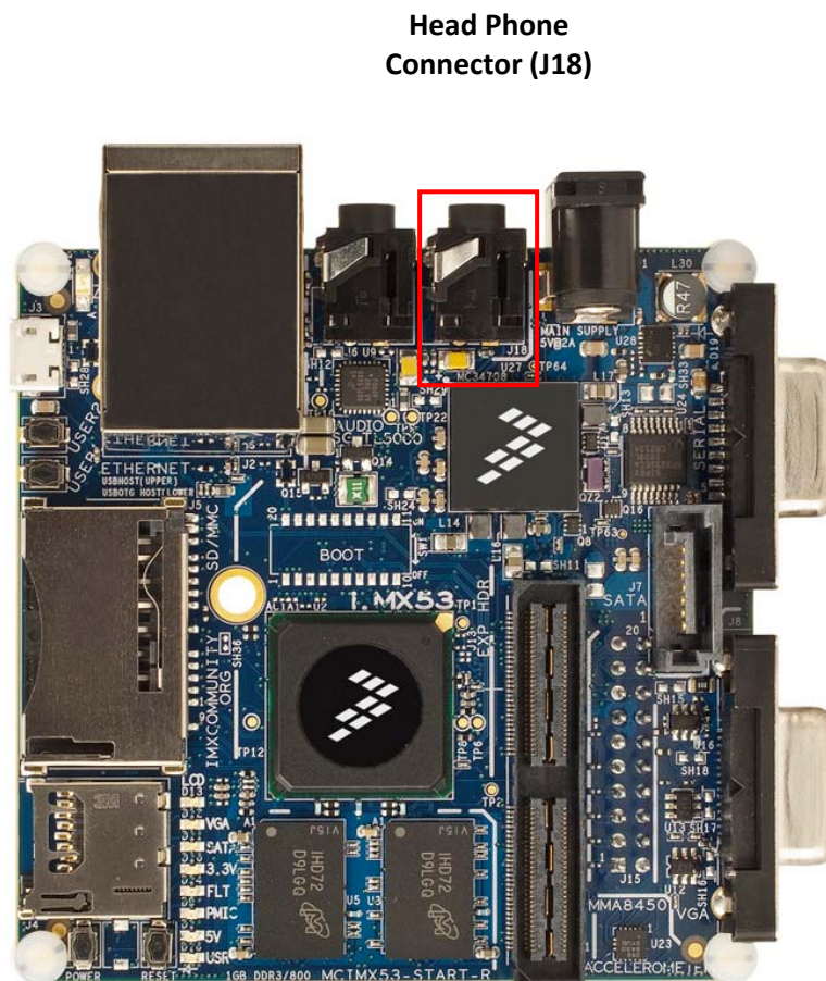
Figure 5. Headphone Output Connector
