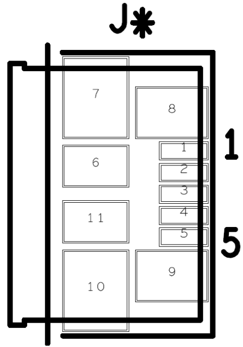
Figure 21. Power Jack (J1)
