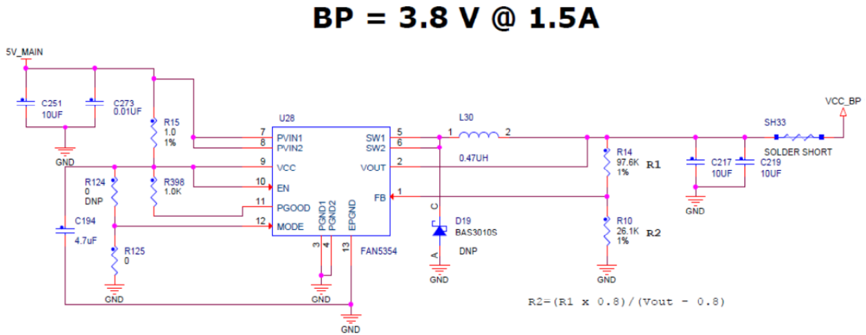
Figure 16. PMIC Main input Power Supply.
