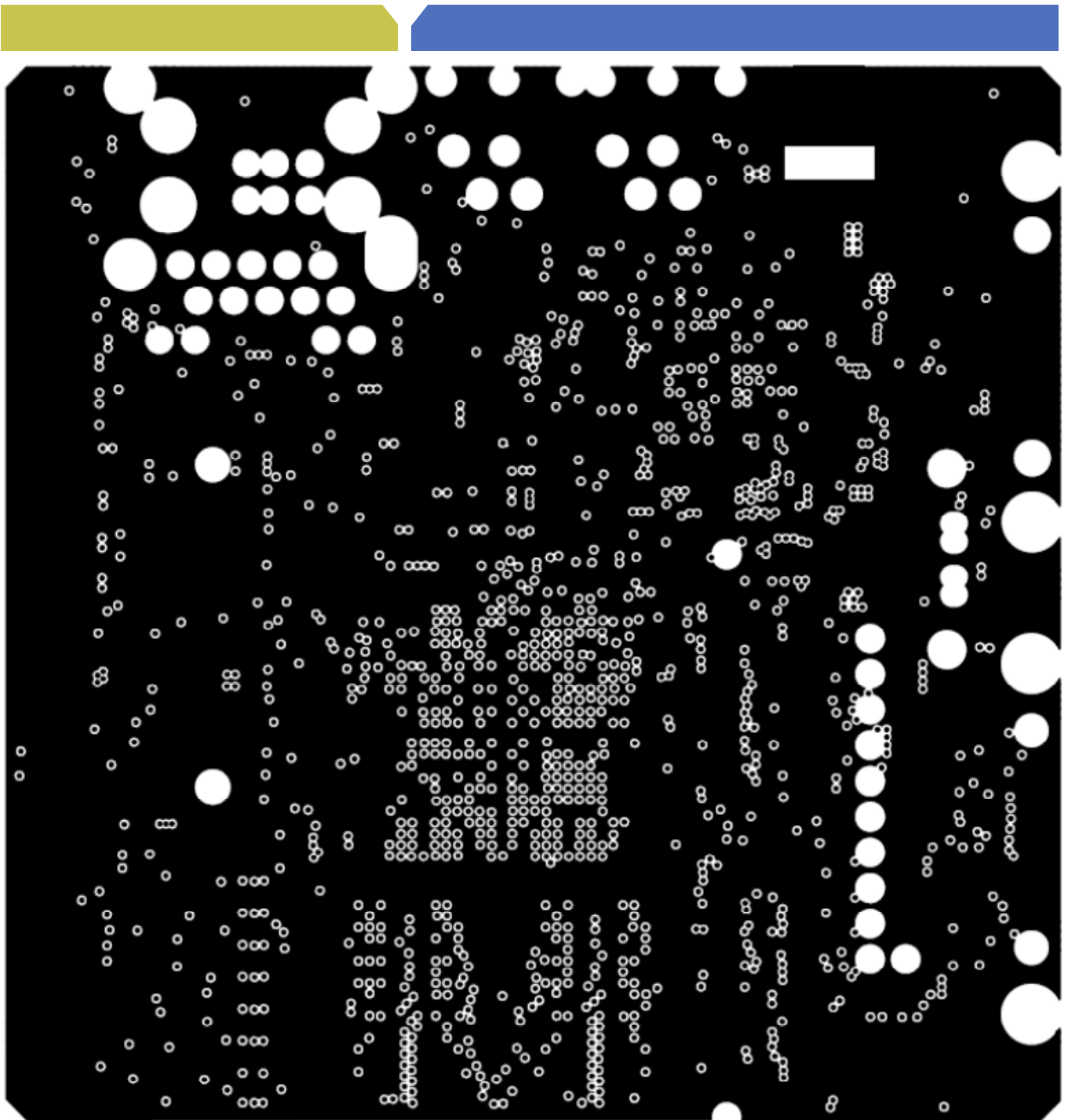
Figure 61. Second Etch Layer
