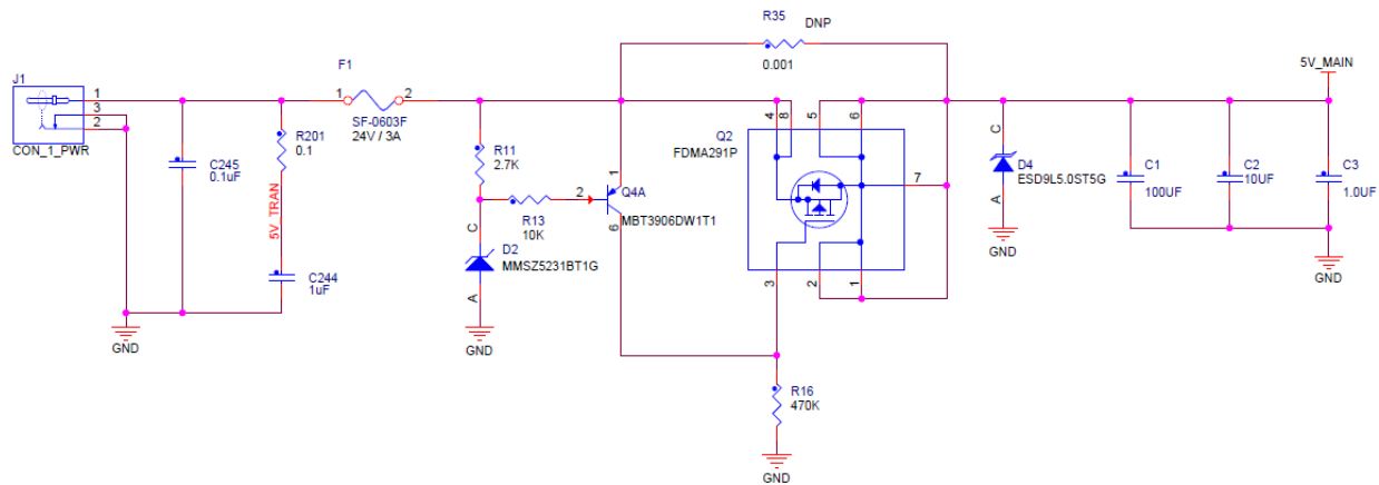
Figure 15. 5V Main input Power Circuit.
