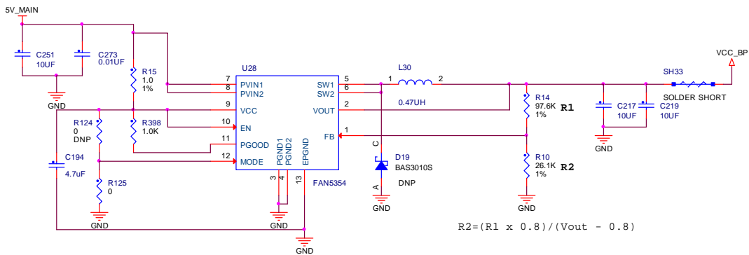
Figure 46. Main 5V INPUT
