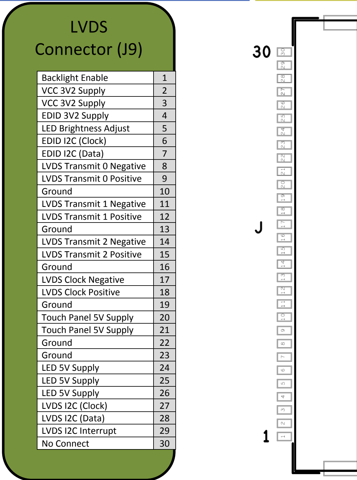
Figure 27. LVDS Connector (J9)
