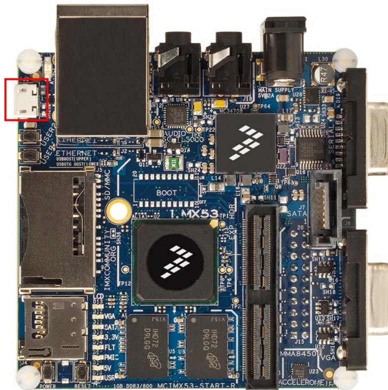
Figure 8. Micro-B USB Device Connector (J3)
