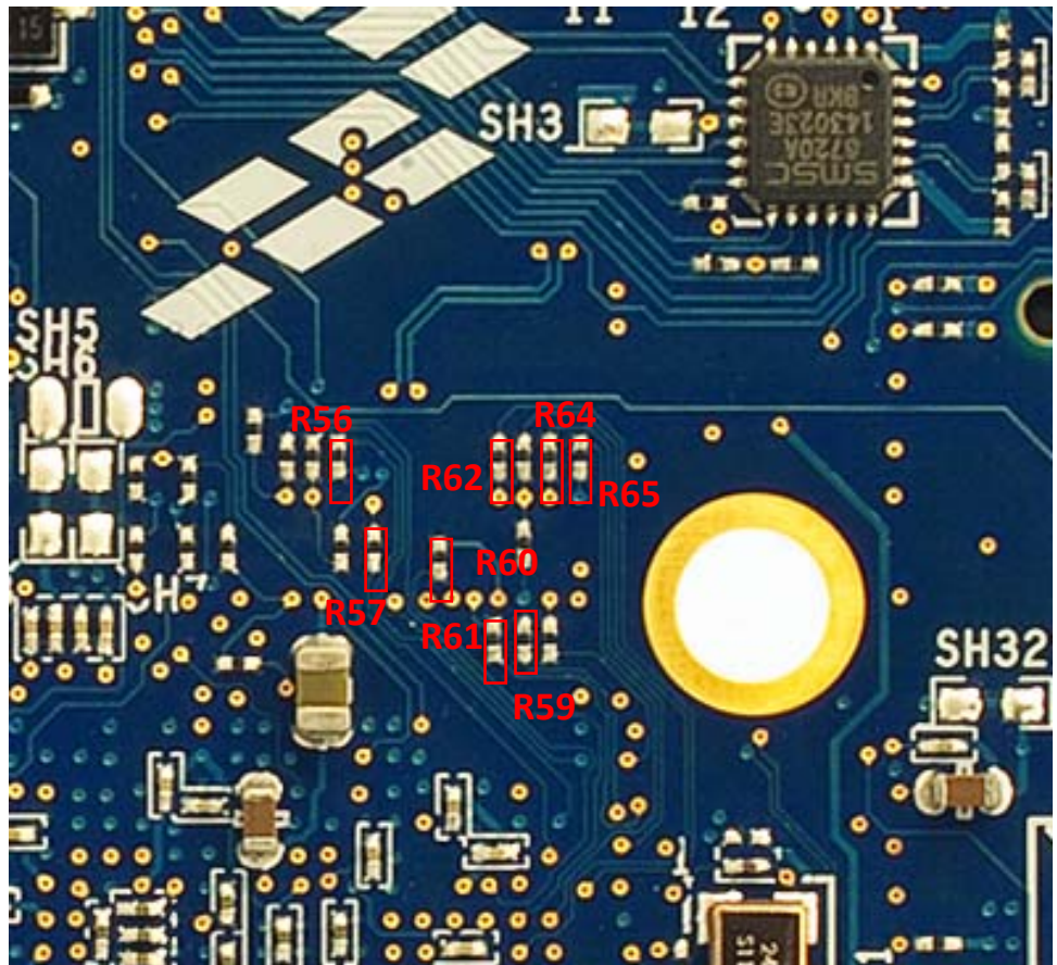
Figure 19. Boot Mode Resistor Locations BOTTOM
