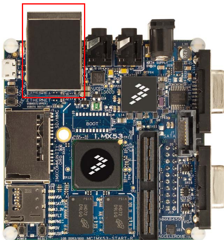
Ethernet/Dual USB Connector (J2)
