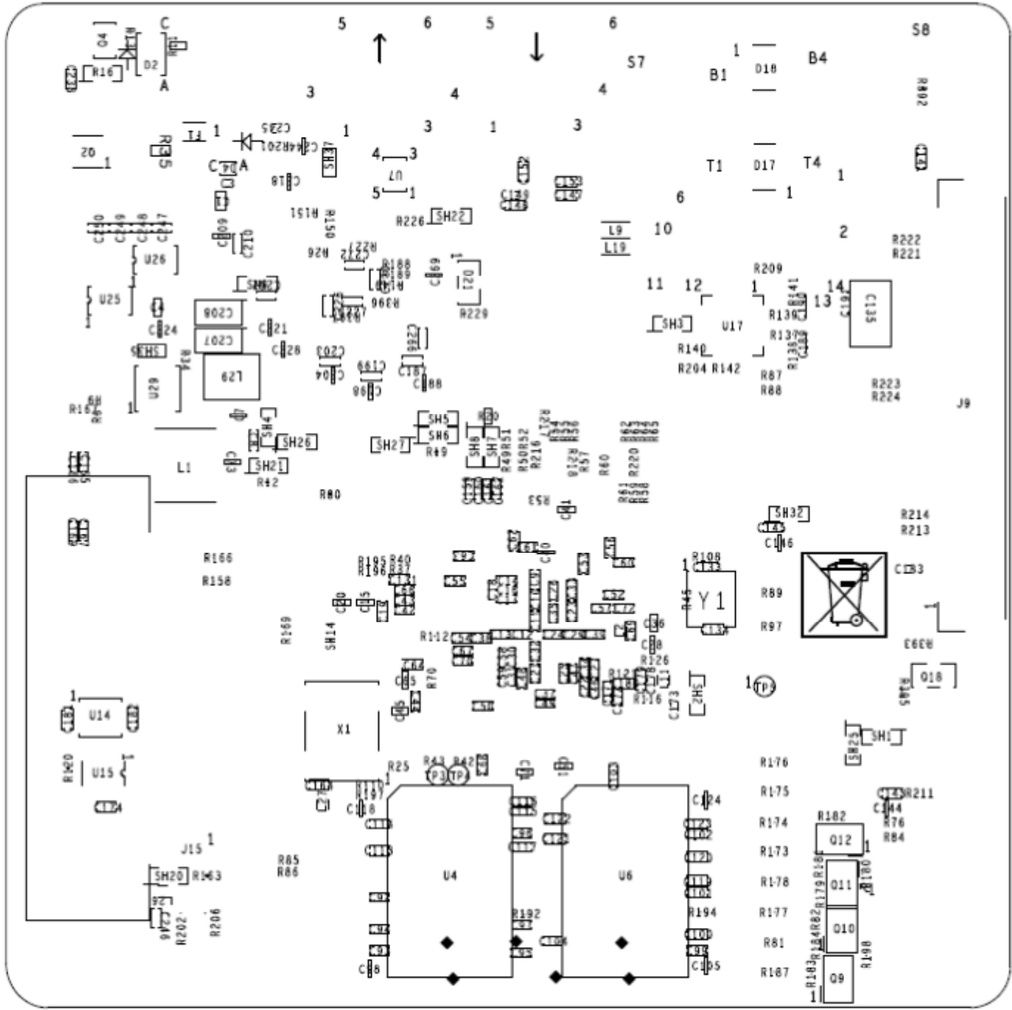
Figure 45. Assembly Drawing Bottom
