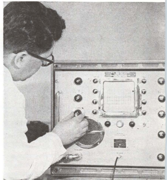
LOCATING a cable fault using pulse-echo technique
