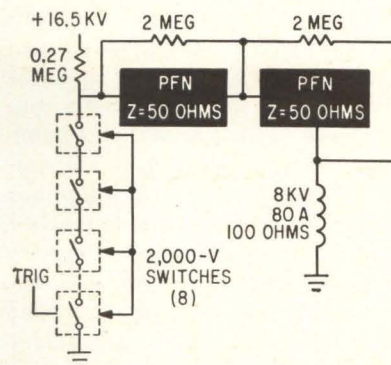
EXPERIMENTAL modulator switches 1.28 megawatts to provide 640-Kv output—Fig. 5
