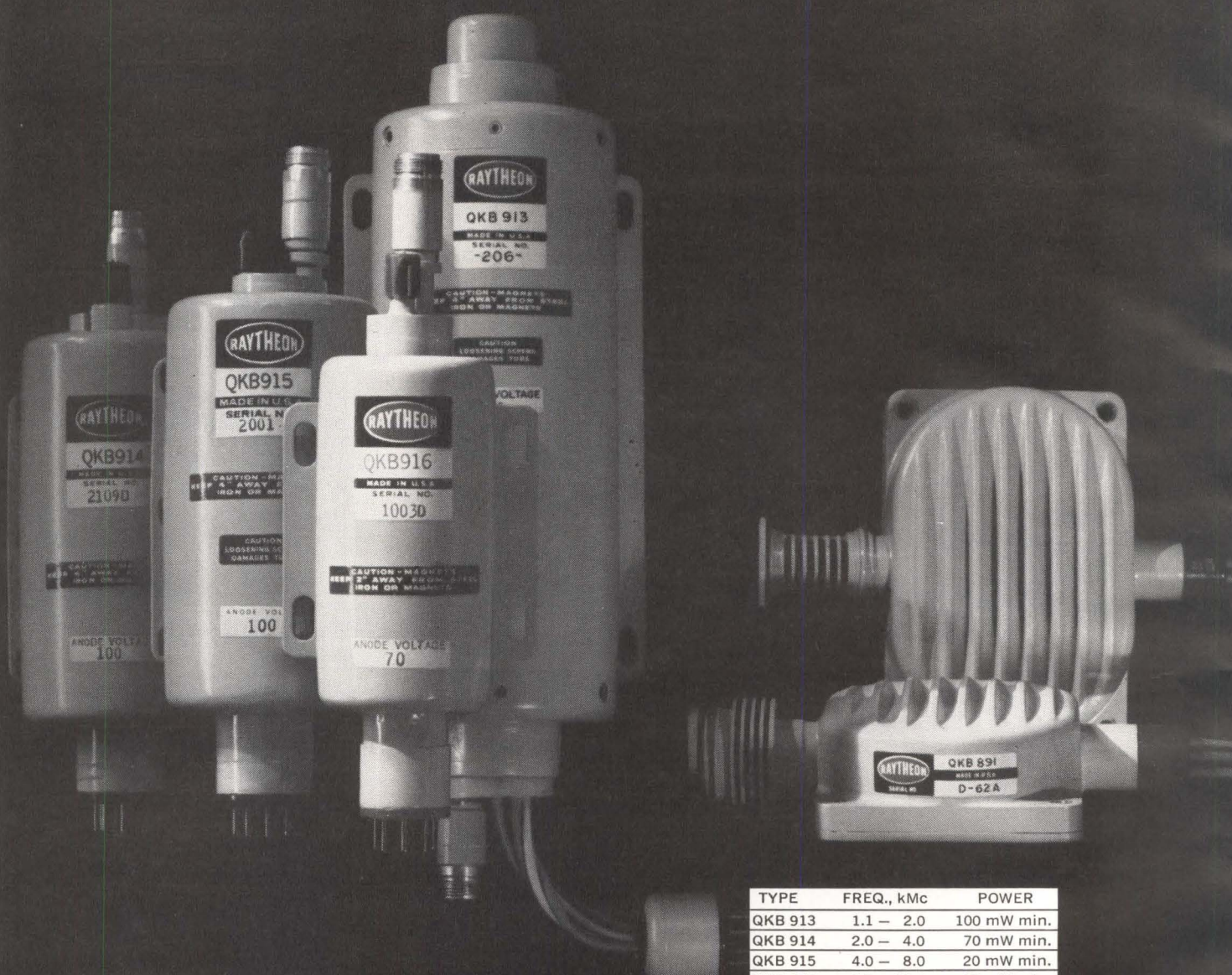
TYPICAL RAYTHEON O-TYPE BWO'S FOR LABORATORY INSTRUMENTS*
