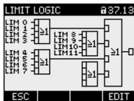
Figure 2-7 LIMIT LOGIC
