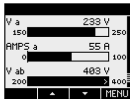
Figure 2-14 Example of a freely definable display (bar diagram)
