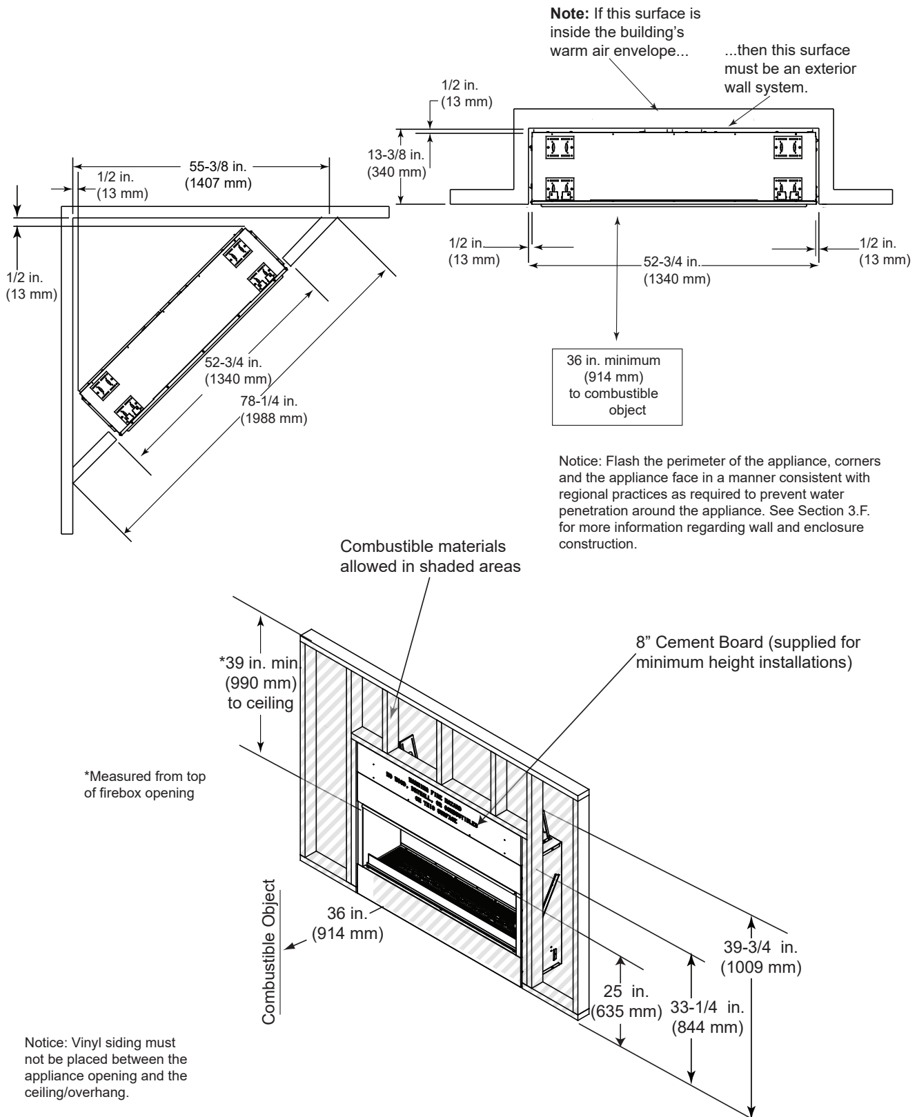
► Figure 3.2. Appliance Locations and Framing Dimensions - ODLANAIG-48
