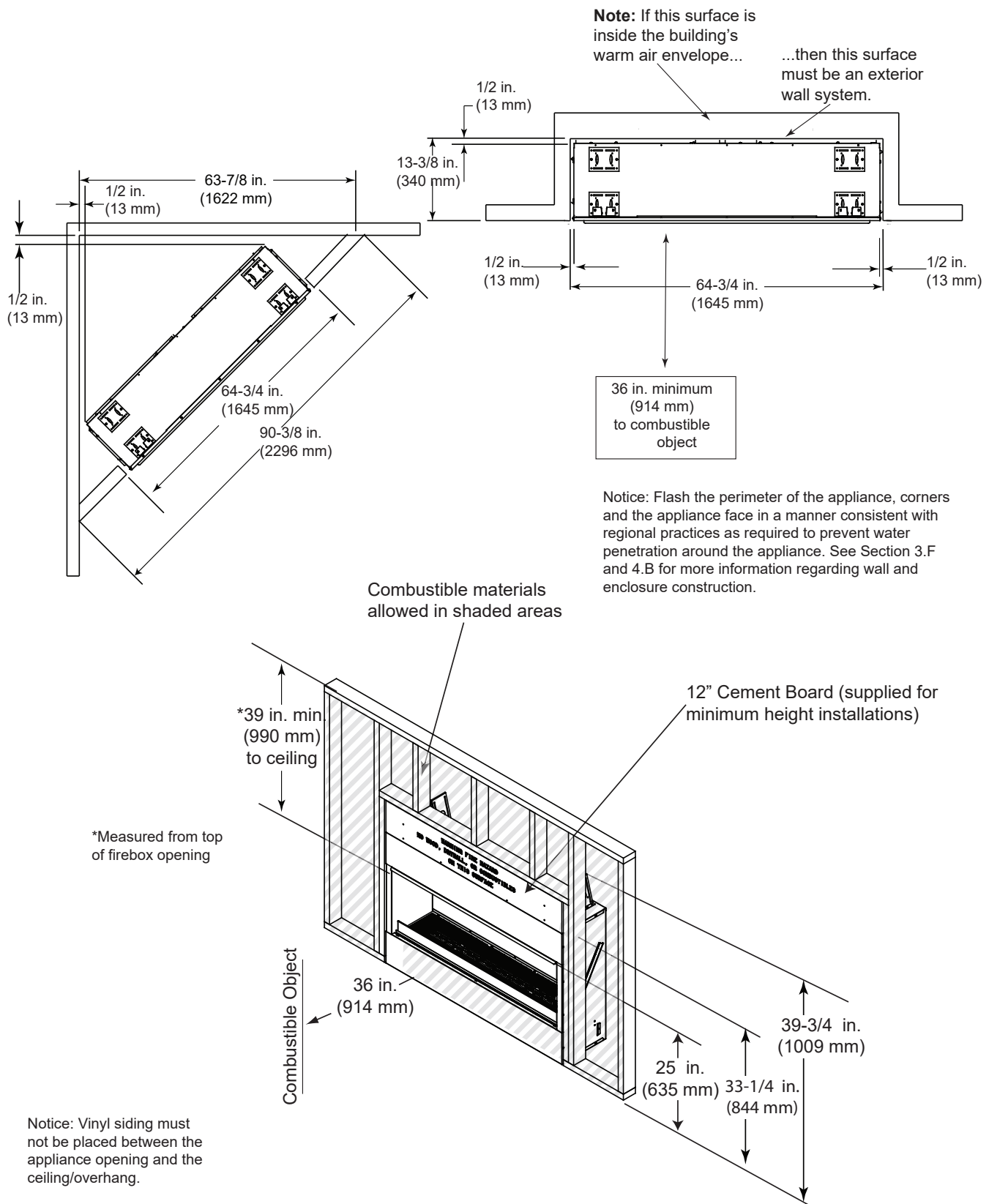
► Figure 3.3. Appliance Locations and Framing Dimensions - ODLANAIG-60
