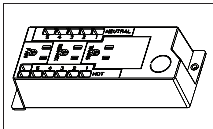
Figure 5.2. Junction Box
