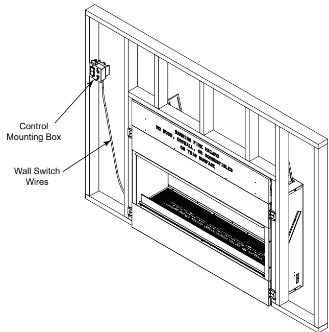
Figure 5.7. Wall Switch Mounting
