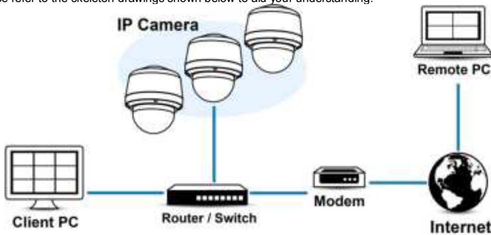
FIGURE 1-11: NETWORK TOPOLOGY
