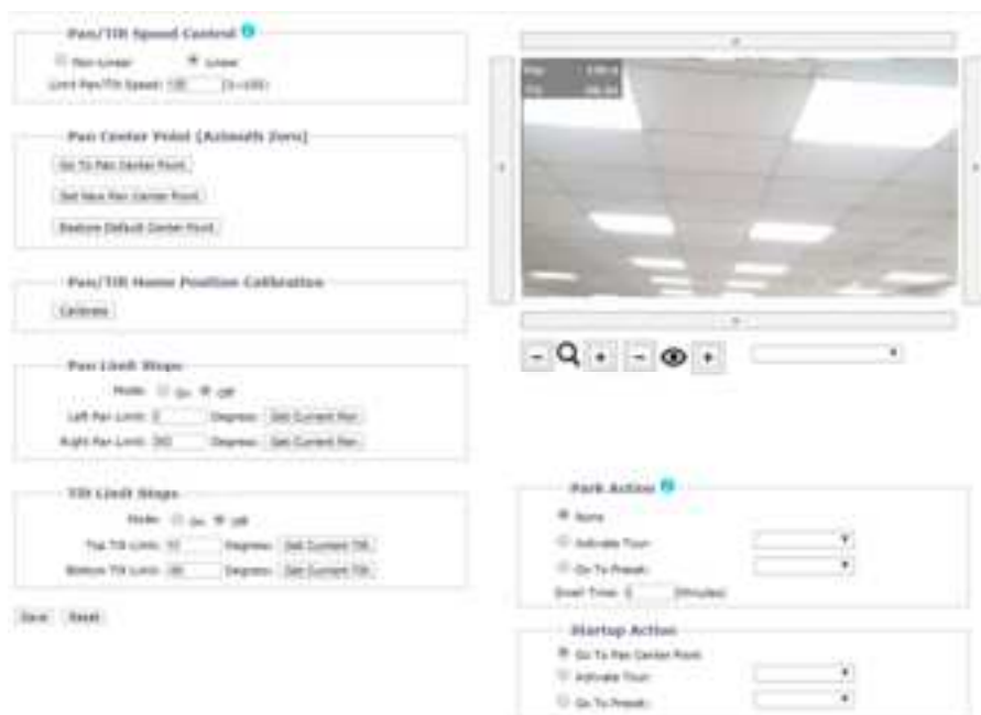
FIGURE 2-42: POSITIONING SETTINGS
