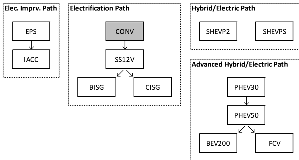
Figure 4. Vehicle-Level (Electrification) Paths
