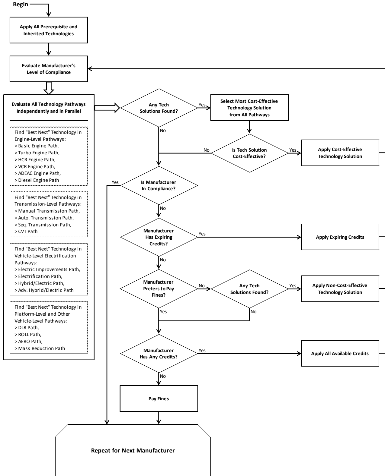
Figure 9. Compliance Simulation Algorithm
