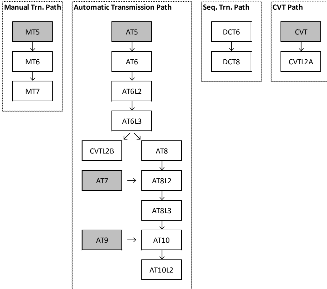
Figure 3. Transmission-Level Paths
