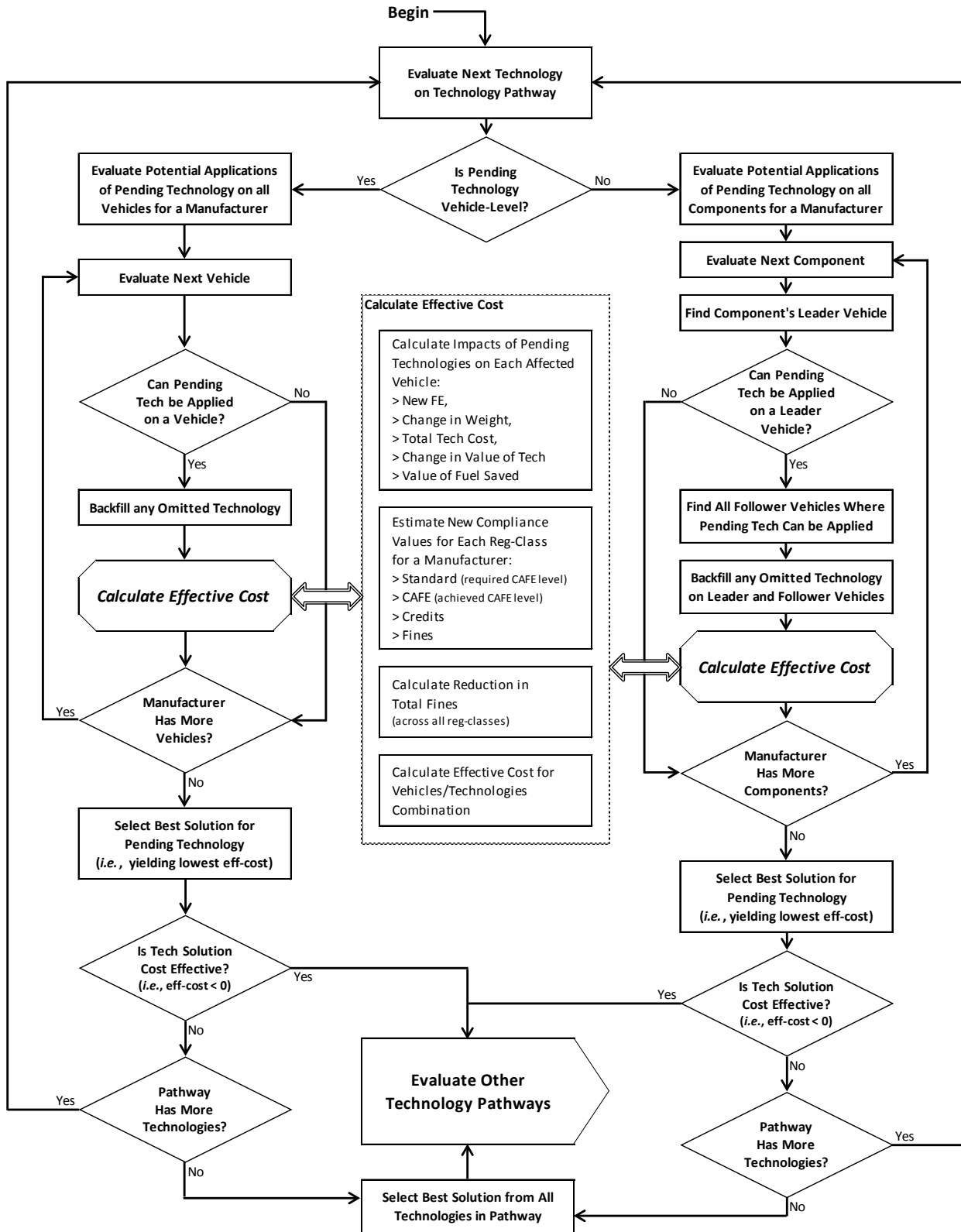
Figure 10. Determination of “Best Next” Technology Solution
