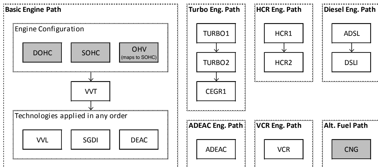
Figure 2. Engine-Level Paths
