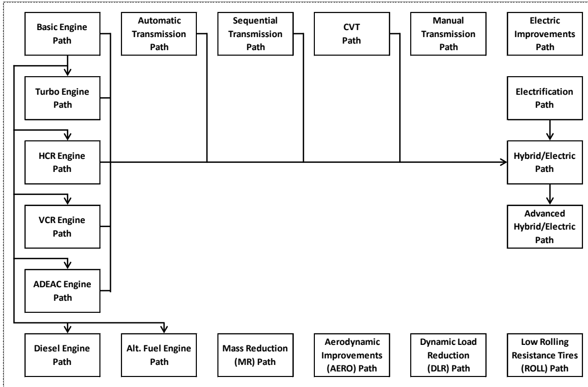
Figure 6. Technology Pathways Diagram
