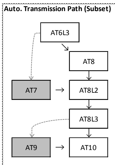
Figure 7. Automatic Transmission Path (Subset)
