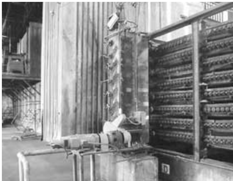
Cut-to-length wet perlite boards are loaded onto an 8-level conveyor prior to passing through the dryer.
