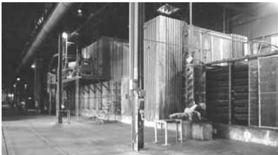
A 400' long, 3-zone oven dries wet perlite board by circulating hot air at approximately 400° to 600° F.
