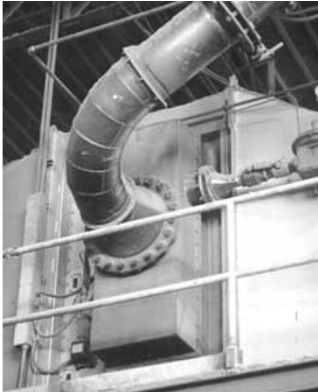
Six Minnox direct fired air-heating burners were retrofitted in the drying oven to significantly reduce NOx and CO emissions.
