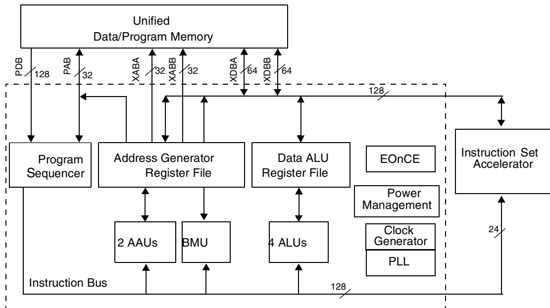
Figure 1. SC140 Core Block Diagram
