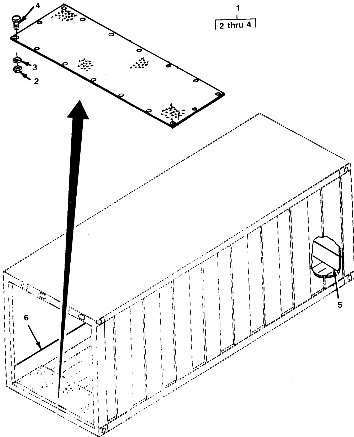
Figure C-7. Threshold Plate.
