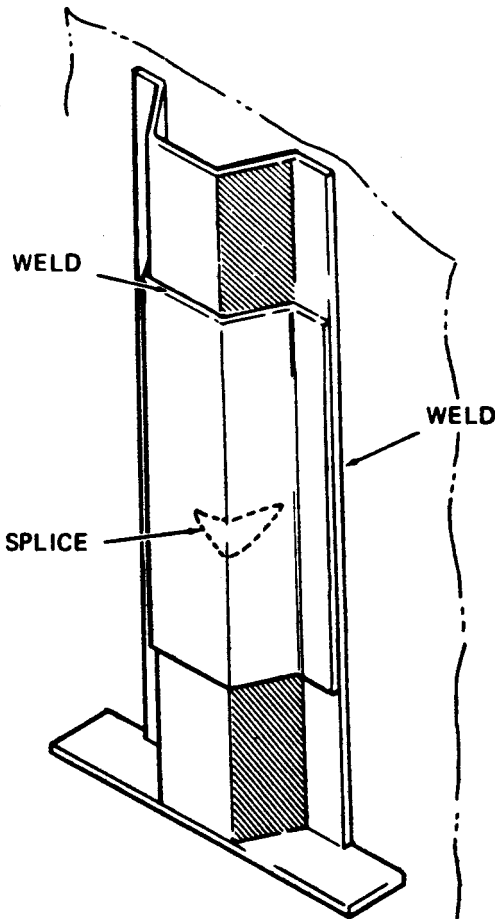
Figure 4-3 Corrugated Panel Repair.
