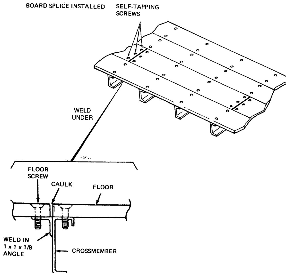
Figure 4-7. Floorboard Section Repairs.
