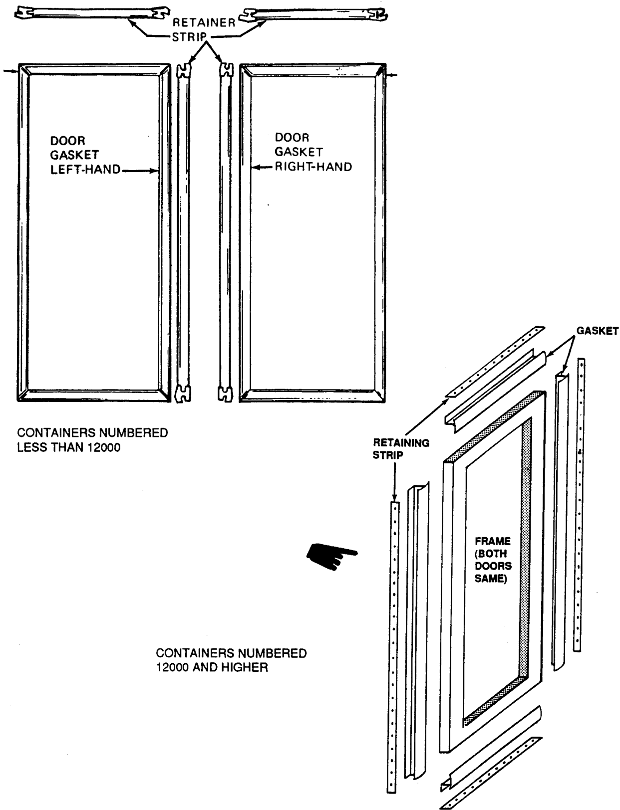
Figure 4-2. Door Gasket Assembly.
