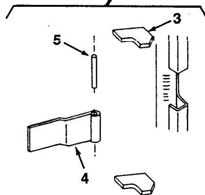
Figure 3-1.1. Door Assembly (Containers Numbered 12,000 and higher)
