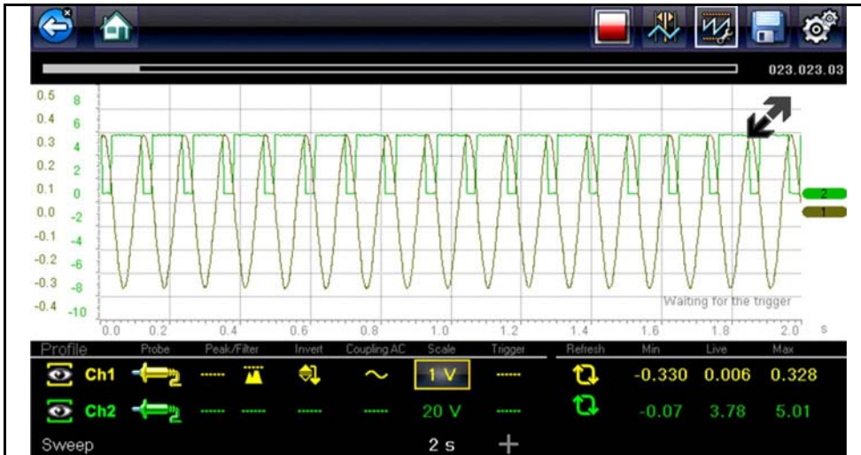
Figure 3-27 Grid on
