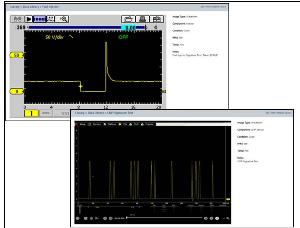
Figure 3-45 Waveform examples
