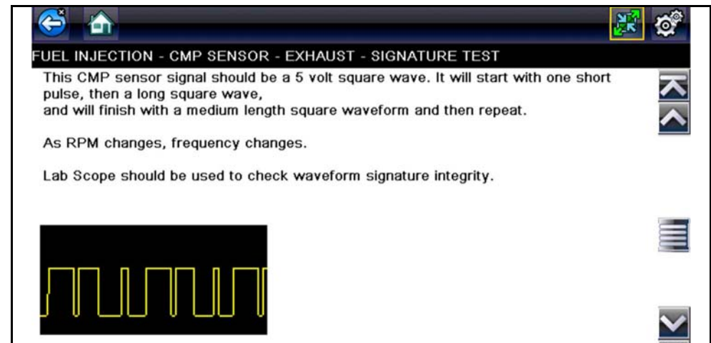
Figure 4-14 Waveform Example
