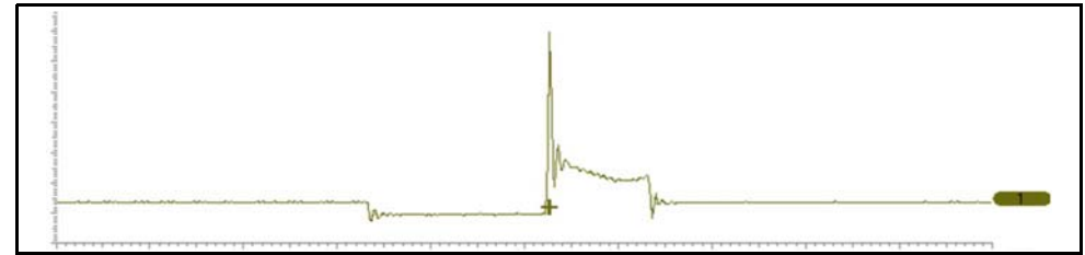
Figure 3-26 Typical Secondary Ignition Signal
