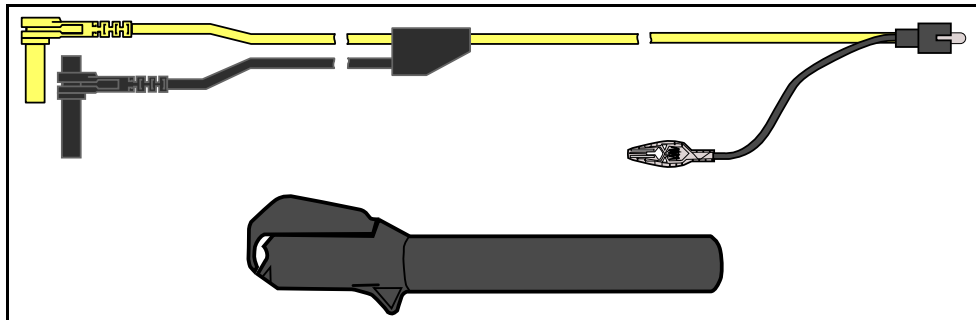
Figure 3-4 Secondary Ignition Coil Adapter Lead and Clip-on Wire Adapter
