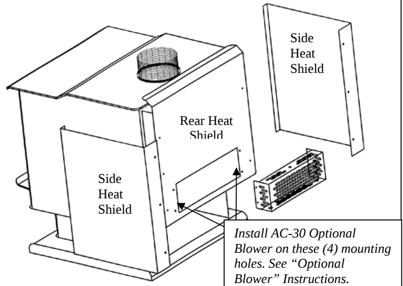
Illustration 3 – Side Heat Shield and Optional Blower Installation
