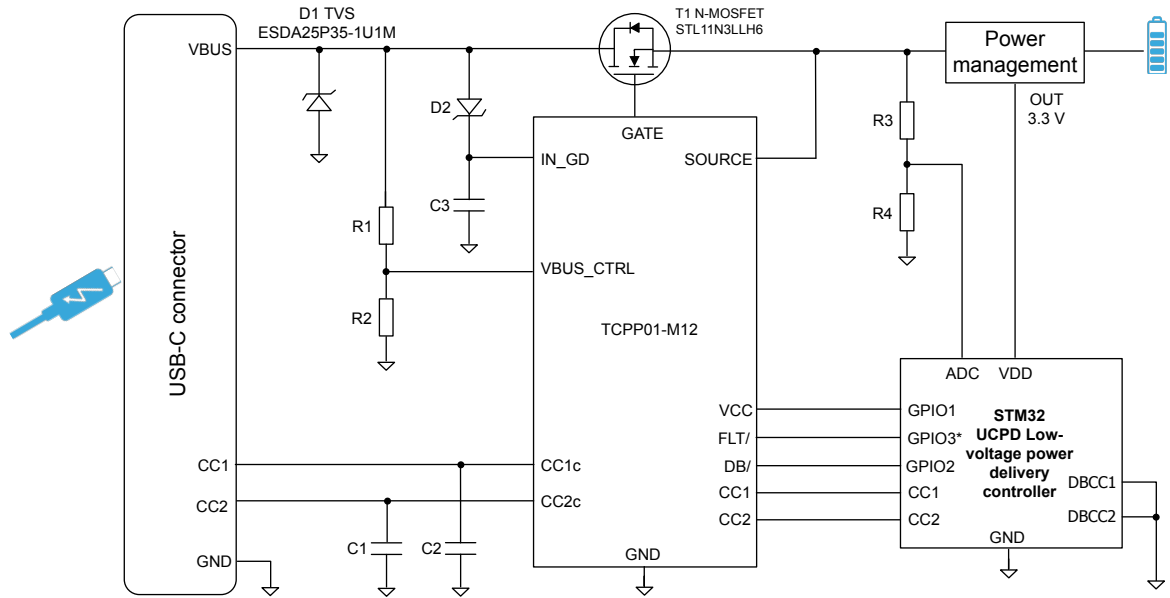
Figure 42. Sink application with battery (PD3.0)
