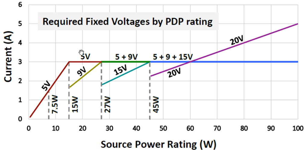
Figure 4. Power profile
