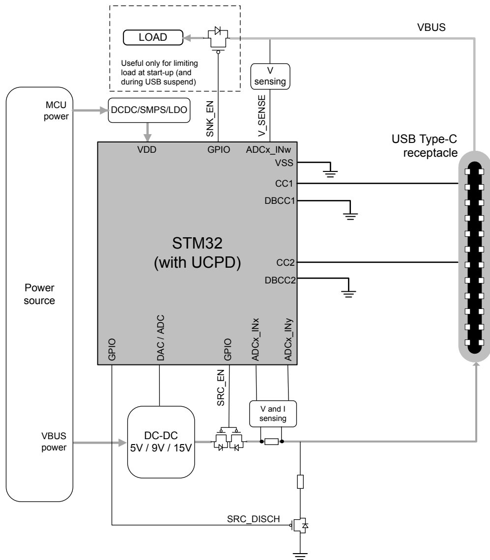
Figure 26. DRP connections
