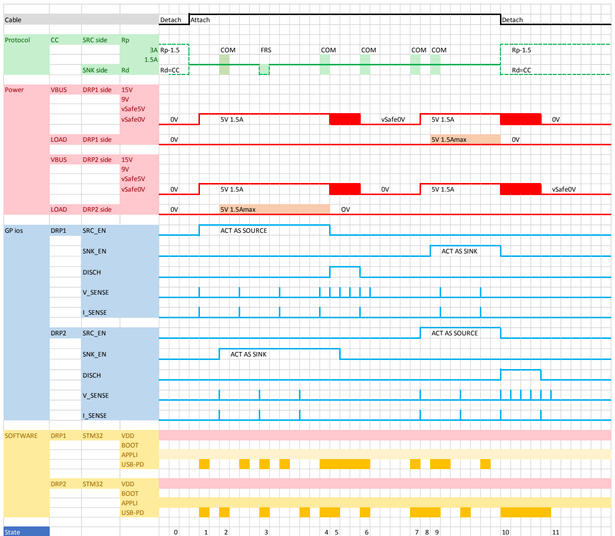
Figure 29. DRP with FRS - time line example
