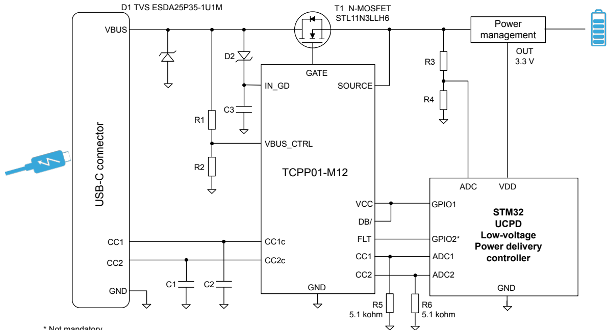
Figure 43. 15 W sink application with battery
