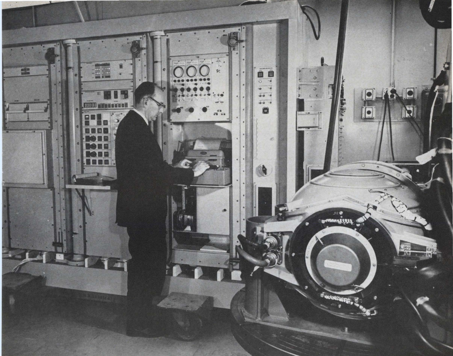
The Polaris missile guidance system is tested by General Electric's MK 462 Autotester. Results are printed on a Flexowriter, and can also be recorded on punched tape for later analysis.
