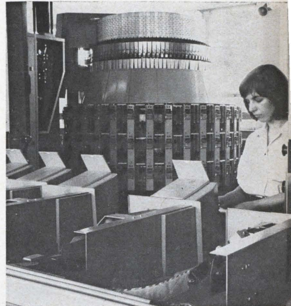
Mail sorting is masterminded from central electronic rack at left, which provides memory and logic. Girl at right stamps zip-code destinations on envelopes, which are sorted in the chandelier-like tower to her right.
