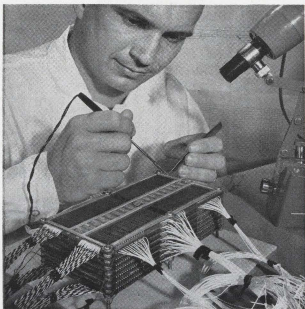
Memory stack (above) can be repaired by using spare words in each plane. Stack is built by wiring board edges (right) and folding up the planes.
