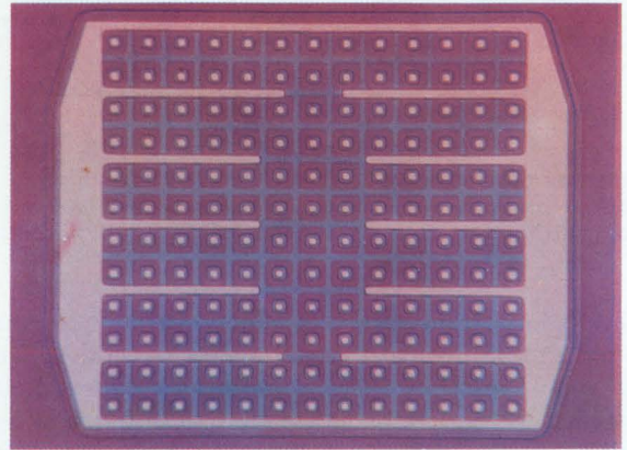
In the fourth step, the contact areas to the emitter and the base are etched.
