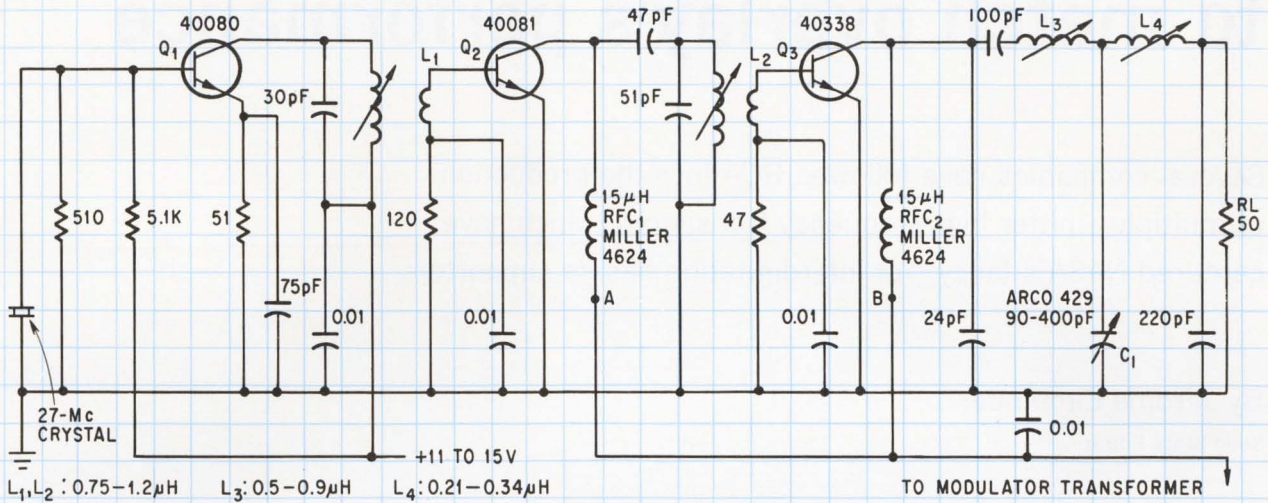
Three overlay transistors are used to form a five-watt 27-Mc citizens-band a-m transmitter. This circuit can handle three watts of carrier power, and can deliver up to 10 watts of peak power under 100% modulation. In citizens-band applications, overlay transistors are competing against conventional silicon planar transistors.
