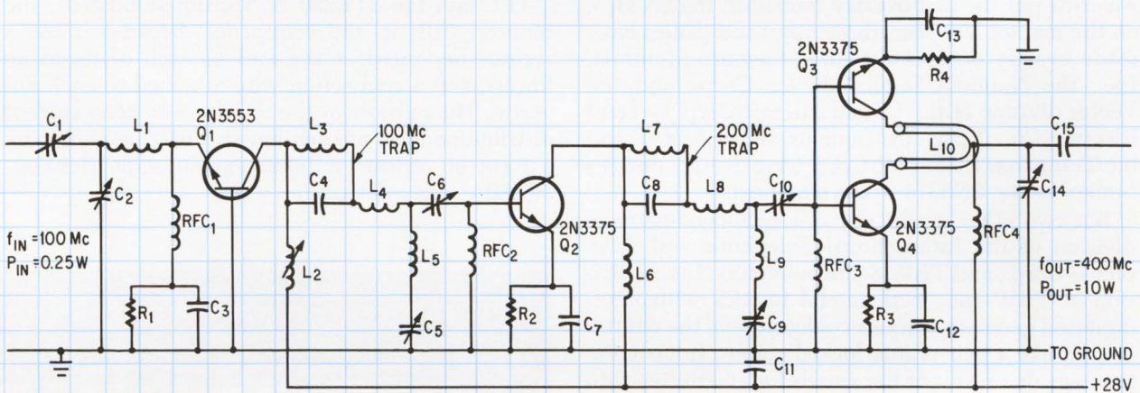
A three-stage power amplifier circuit designed with four overlay transistors for use in telemetry equipment. This circuit serves as both a frequency quadrupler and as an amplifier. In the final stage, two 2N3375's are operated in parallel. The circuit converts a 100-Mc, 0.25-watt input signal into a 400-Mc, 10-watt output signal. The over-all power gain is 16db.
