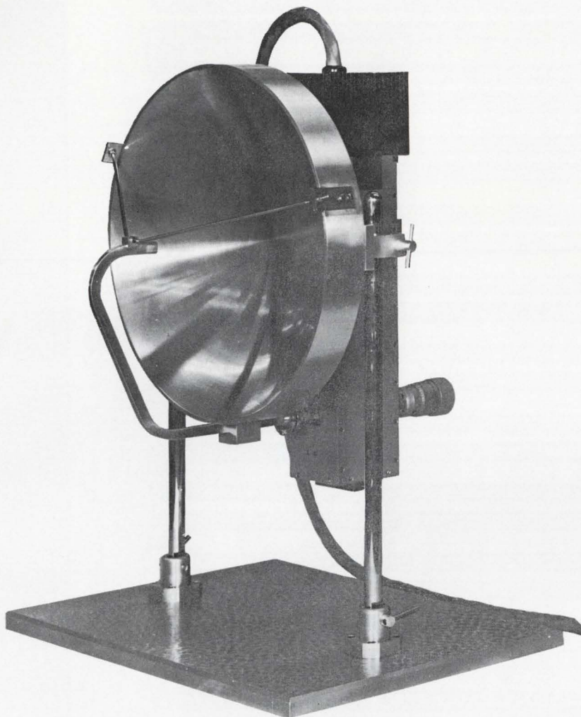
Elliptical antenna focuses microwave energy to a point 17 inches away. It is used for measurements on targets that are relatively inaccessible. Heat sink, at top of assembly at rear of antenna, dissipates heat from klystron.
