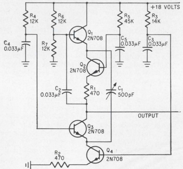
Rise and fall times of high-frequency multivibrator are not dependent on timing capacitor C_1 , because of emitter coupling through Q_1 and Q_3 .
