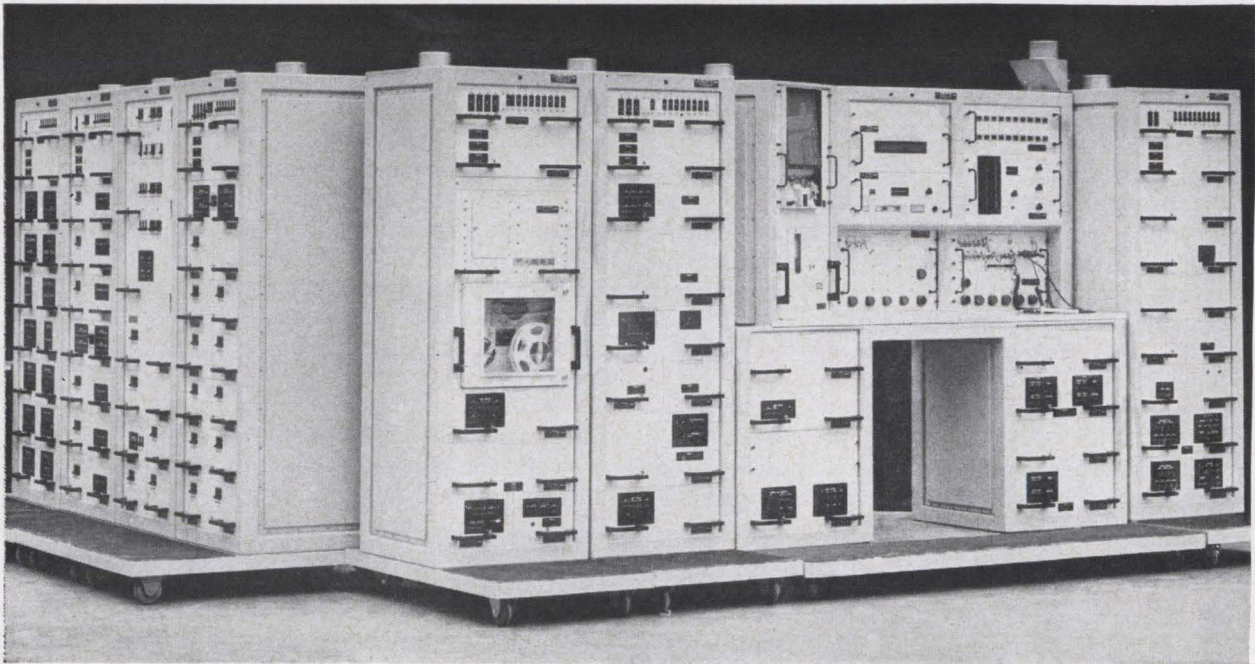
Dimate , the depot installed maintenance automatic test equipment being supplied to the Army Electronics Material Agency, is a modularized test system capable of automatic, semiautomatic, and manual operation.
