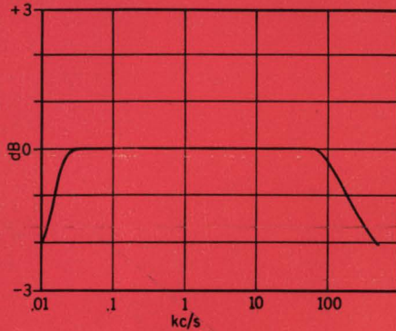
Linear response at 25 watts output from 20 c/s to 200 kc/s for push-pull operation with RCA 2N3878
