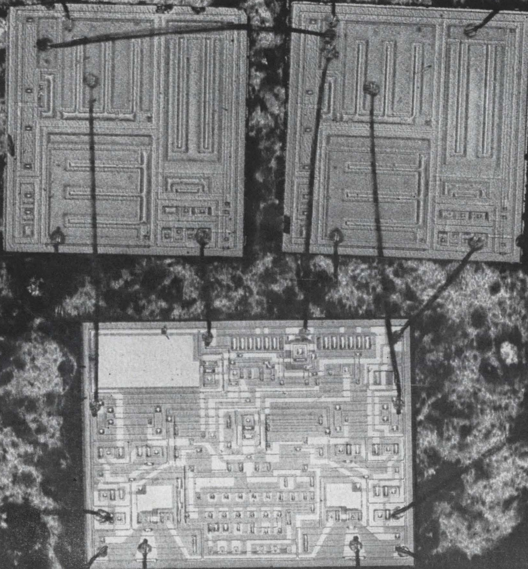
Forty-watt servo amplifier is made with three silicon chips, two carrying high-power transistors and one for control circuitry. Leads are aluminum wire; chips are aluminum-bonded to molybdenum.
