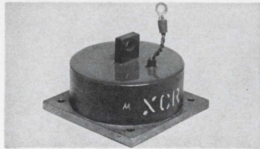
Array of scr's is shown with resistors attached to cathode leads of individual rectifiers. The entire unit is covered by a metal case.
