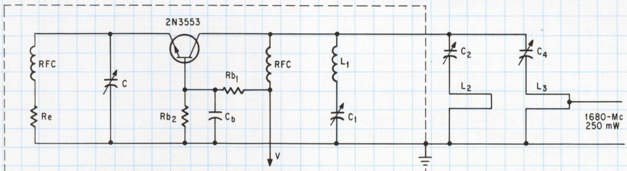
In this frequency-multiplier circuit using a 2N3553, the transistor oscillates at 420 Mc. The frequency is quadrupled to 1,680 Mc by the circuit. Power output is 250 milliwatts.
