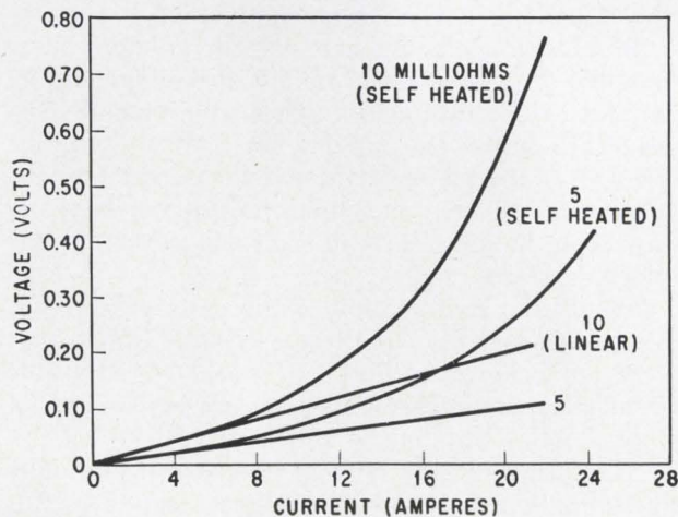
Characteristics of equalizing resistors: The self-heating copper resistors provide sharp increases in resistance at high anode currents. This accounts for the high voltage drops which they produce at high currents.
