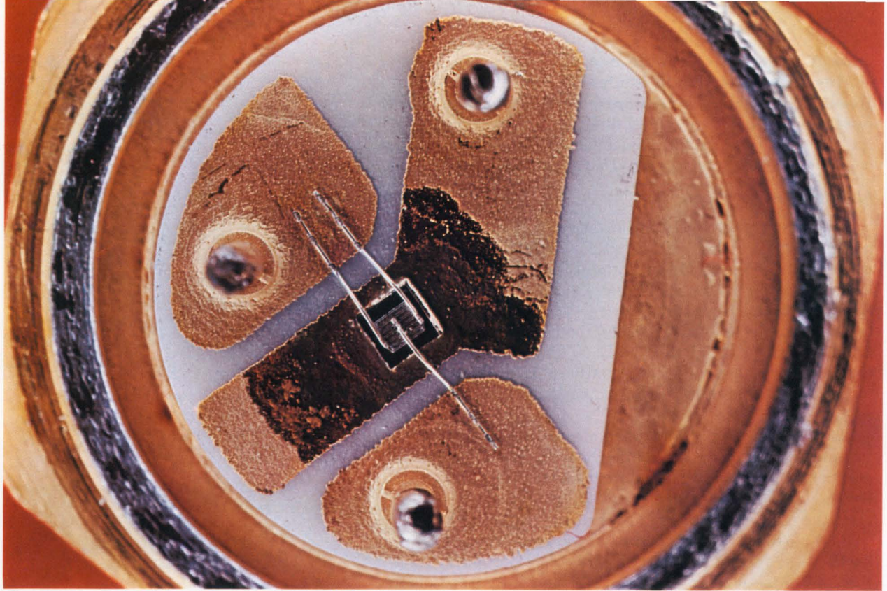
The 2N3375 pellet after mounting and ultrasonic aluminum-to-aluminum bonding. The center lead is the emitter connection. The two outer leads are connected to the base. Center metal area of package carries the collector current to the collector riser wire. Emitter, base, and collector are insulated from the Jedec TO-60 stud-mounted case by a thick layer of beryllium oxide (white region).
