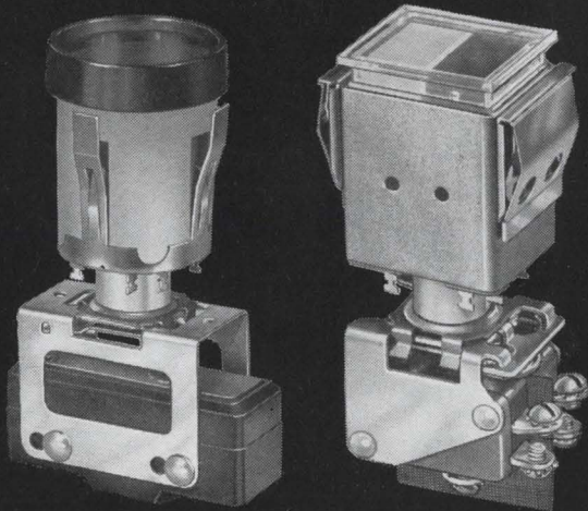
Series 2—The original Series 2 introduced modular construction in lighted pushbutton switches. Choice of round or rectangular display, Snap-in mounting. Available with RFI shield, and solenoid pull-in and/or hold-in coil for remote control.
