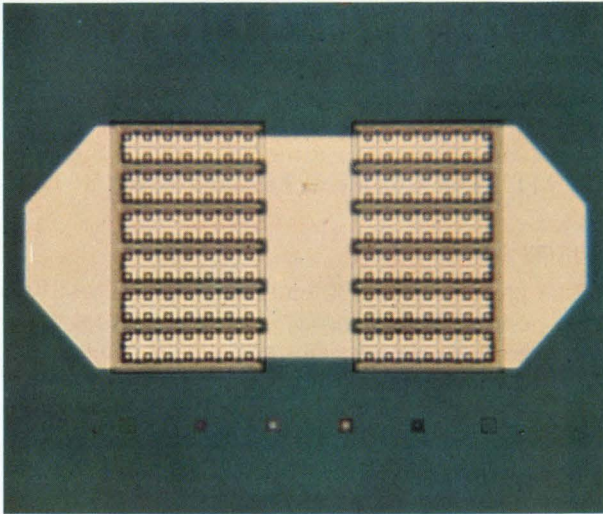
Vector's experimental VX168-10 is a 168-emitter device with a power output of 1 watt and 6-db power gain at 800 Mc. It can dissipate 12 watts.
