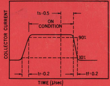
Total saturated switching time at 4 amperes less than 1 µs (typ) with RCA 2N3879
