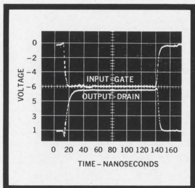
Figure 5. Unretouched sampling scope photograph illustrates zero storage time and fast response of TI 2N3823 FET.
