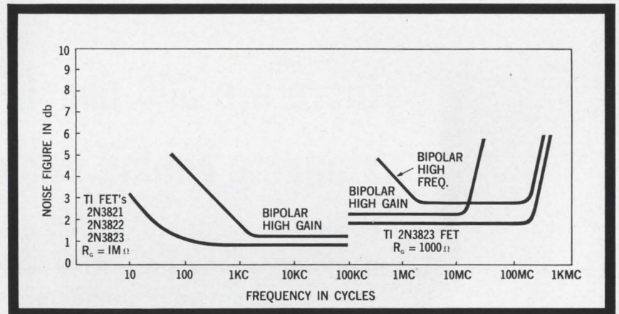
Figure 6. Optimum noise figure vs frequency TI 2N3823 FET vs widely used bipolar transistors.
