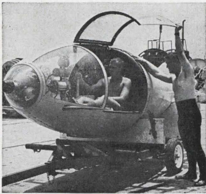
Wet submarines travel at 9 knots but are too maneuverable to use at deep levels where a quick ascent would be dangerous to aquanauts. The miniature sub might be used by surface divers to take supplies to Sealab.
