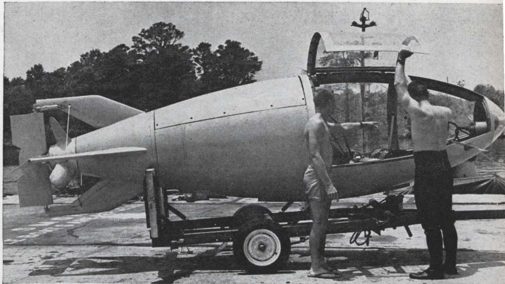
Wet submarines travel at 9 knots but are too maneuverable to use at deep levels where a quick ascent would be dangerous to aquanauts. The miniature sub might be used by surface divers to take supplies to Sealab.
