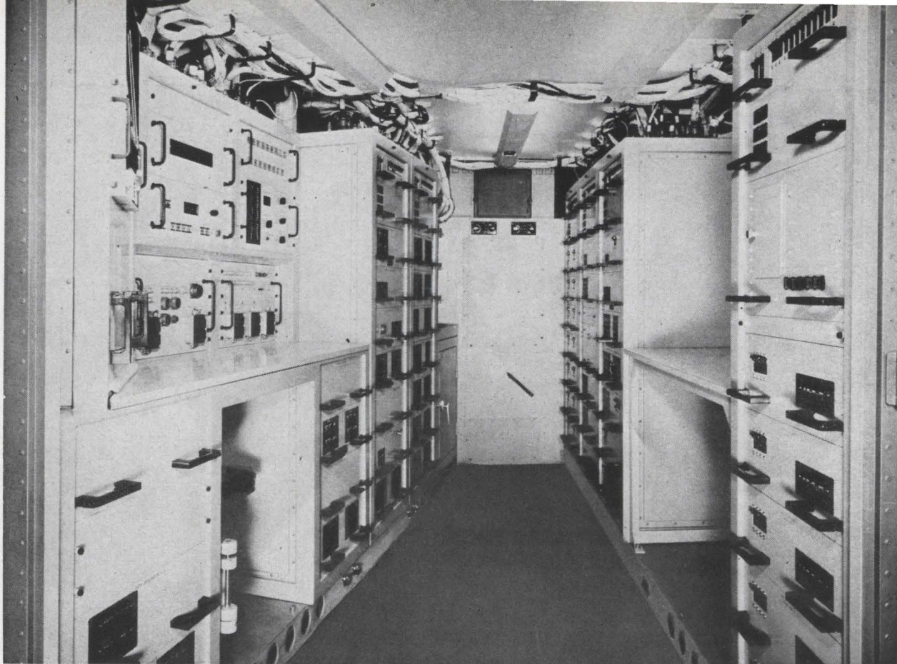
ETS-1 shelter for the Army's Multisystem Test Equipment. Units under test are connected to the panel above the operator's work bench at left. The visual instructor, as well as a test result panel and printer, are also located over the test bench. Measurements chassis are housed in the rack at rear left, to the right of the test bench. Power supplies are at right foreground and low-frequency stimuli at right rear.
