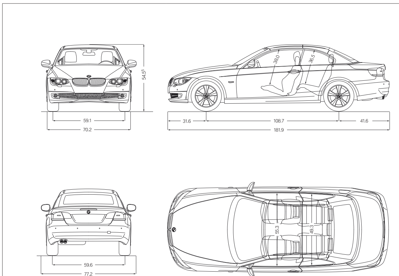
Illustrations above: all dimensions in inches.
