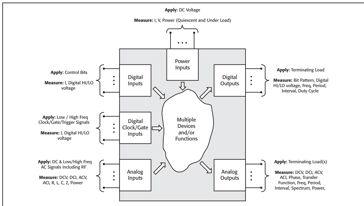
Figure 2. Complex ICs can have multiple analog and digital inputs and outputs. Testing may require multiple measurements with multiple stimuli.
