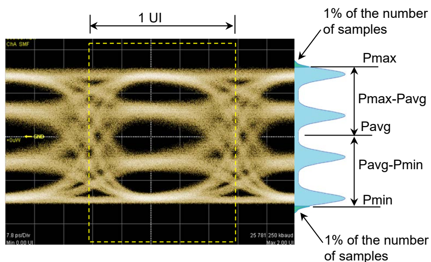
Figure 1.5-24 Power Excursion Measurement Level
