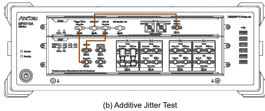
Figure 7.3.4-2 Additive Jitter Test Connection Diagram
