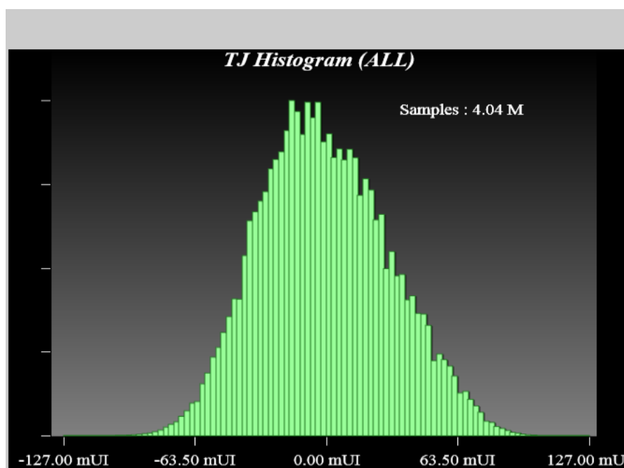
Figure 6.2.2.2-1 TJ Histogram
