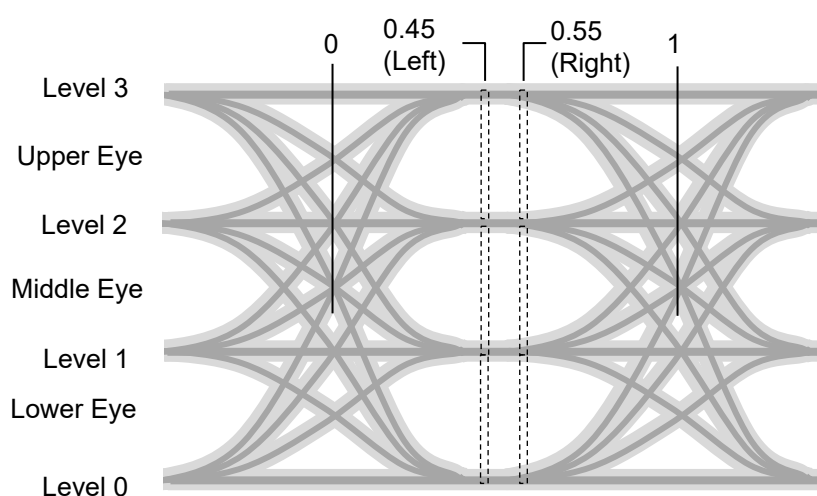
Figure 1.5-23 Partial Noise Margin Measurement Positions
