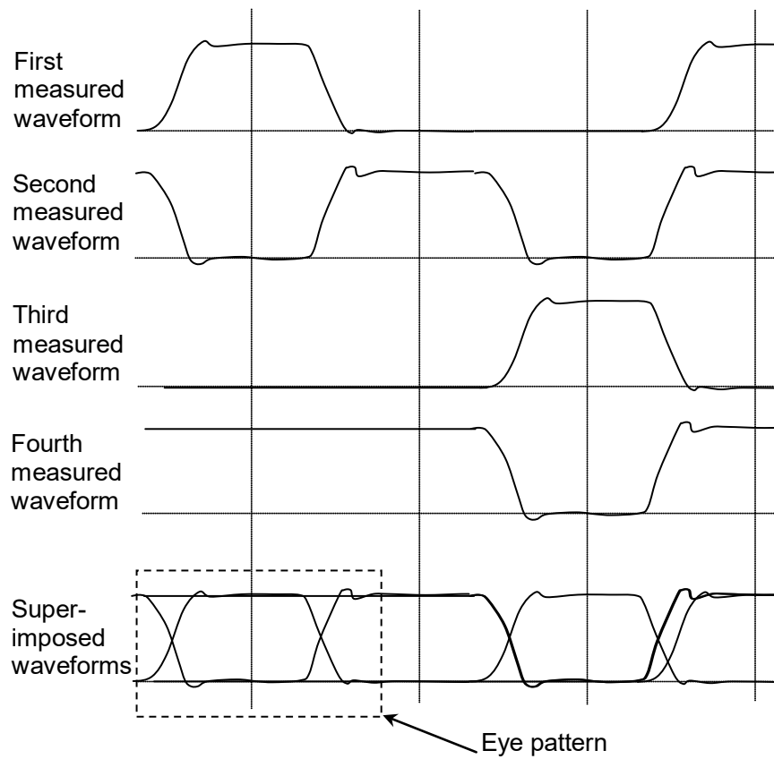
Figure 1.5-14 Eye Pattern Drawing Method
