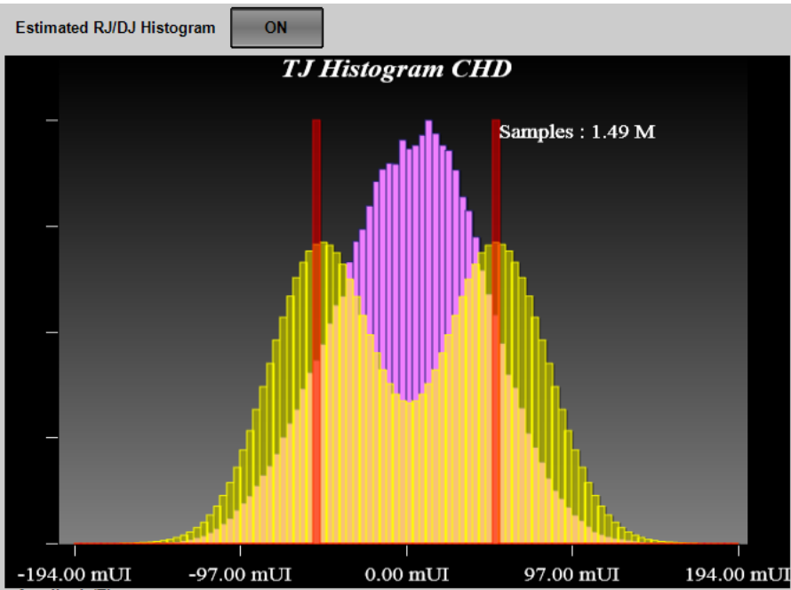
Figure 6.2.2.1-1 TJ Histogram
