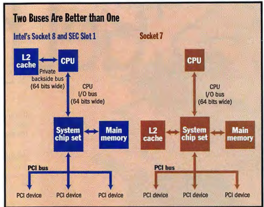
Socket 8 and Slot 1 have two independent 64-bit buses, improving cache access bandwidth over Socket 7.
