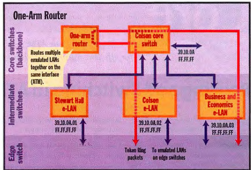
A router manages the Layer 3 protocols for multiple emulated LANs through one point on the ATM network.
