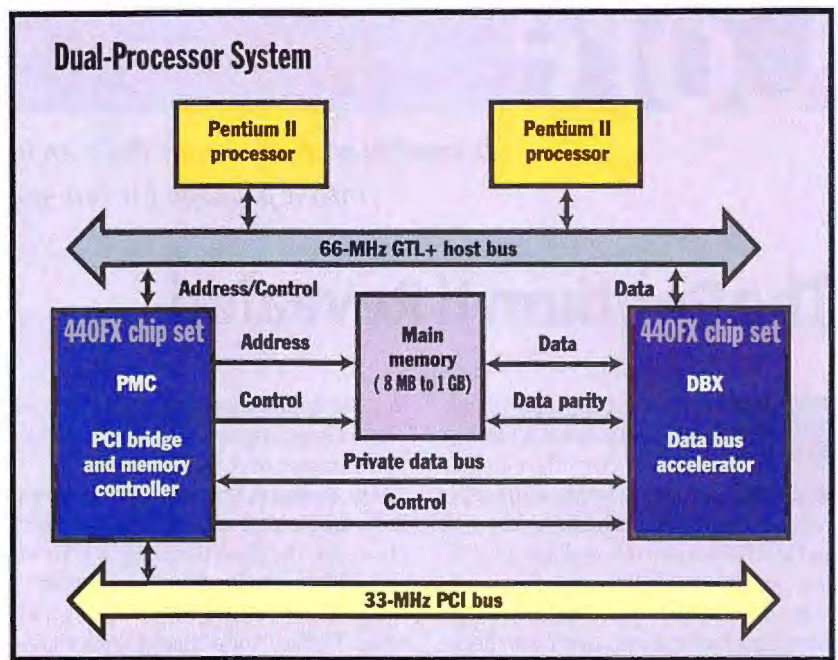
Support for two processors and EDO DRAM reduces system costs.
