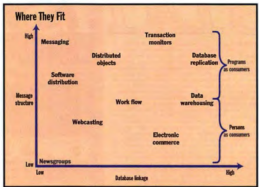
P&S software is described by how structured its messages are and how tight its database integration is.
