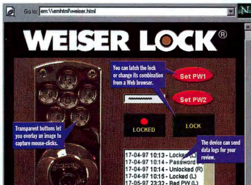
EMIT enables you to obtain logging information from a device.
