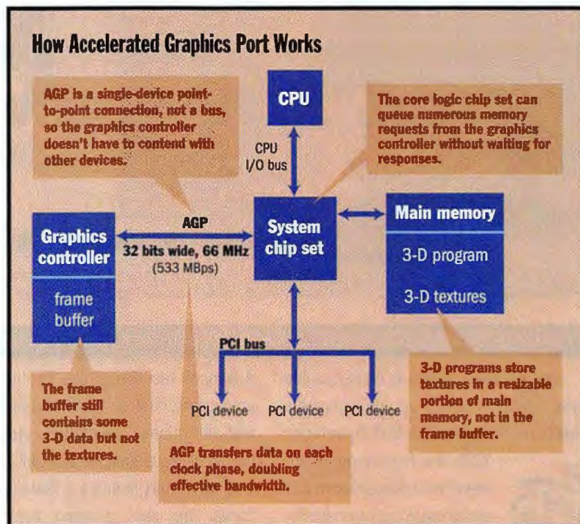
AGP bypasses the PCI bus. Thus, the graphics controller can access memory four times faster.
