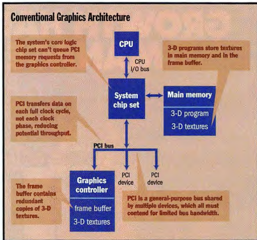
There are several problems with the graphics architectures of today's PCs.
